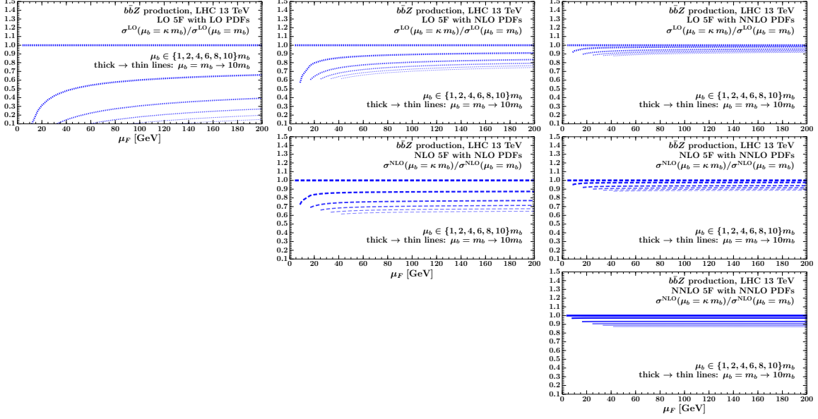
Figure 7. The ratio eq. (4.3) as a function of \mu_F for \bar{b}bZ production at LHC 13 TeV.
