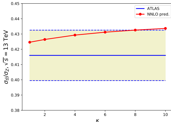
Figure 11. Ratio of total inclusive t\bar{t} and Z cross-sections for \sqrt{s} = 13 TeV for a series of \mu_b = \kappa m_b values versus the ATLAS measurement [62] (shaded band).
