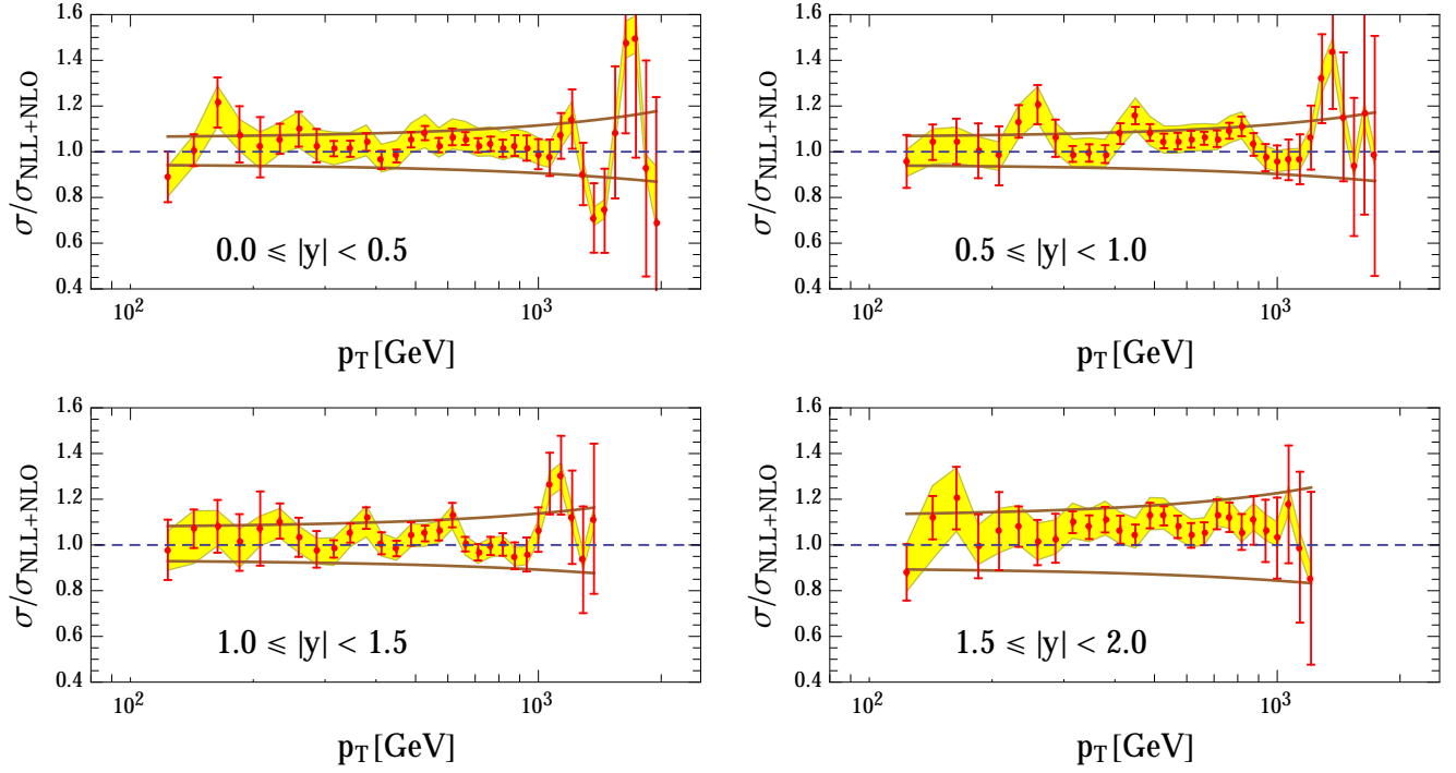
FIG. 9: The ratio \sigma_{\text{Data}}/\sigma_{\text{NLO+NLL}} for CMS data collected at \sqrt{S} = 13 TeV [22] with R = 0.4 to the theoretical results using the PDFs of CT14 [70] at NLO. The error bars represent the experimental statistical errors and the solid (brown) lines the systematic ones. The band (yellow) indicates theoretical scale uncertainties.
