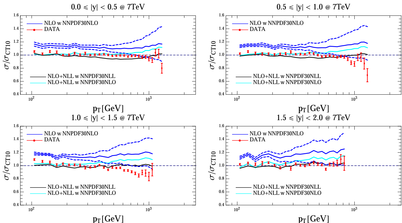
FIG. 16: Same as in Figs. 11 and 13 for the cross sections \sigma_{\text{NLO+NLL}} and \sigma_{\text{NLO}} using the PDF sets NNPDF3.0 at NLO without and with resummation [39], labeled as NNPDF30NLO and NNPDF30NLL in the plots, respectively. The dashed lines (blue) indicate the PDF uncertainties for \sigma_{\text{NLO}} with the set NNPDF30NLO.
