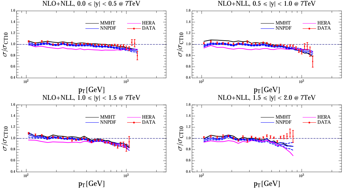
FIG. 11: Cross sections \sigma_{\text{NLO+NLL}} at NLL + NLO accuracy with R = 0.5 using the central PDF sets HERAPDF2.0 [74], MMHT2014 [64] and NNPDF3.1 [75] normalized to the one with CT10 PDFs [71] at NLO. The dashed lines (blue) indicate the PDF uncertainties for the NNPDF3.1 set. The CMS data collected at \sqrt{S} = 7 TeV [17] with R = 0.5 with their experimental statistical errors are displayed as dots (red).
