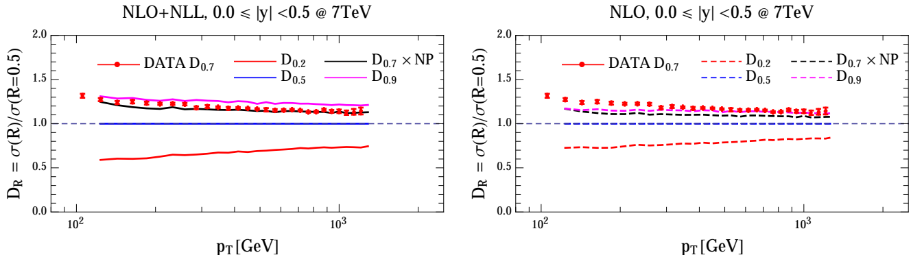
FIG. 2: Ratios D_R of Eq. (5) with R_{\text{fixed}} = 0.5 at \sqrt{S} = 7 TeV for the cross sections at NLO + NLL (left) and NLO (right) accuracy using the MMHT PDF set [64] at NLO with NP correction factors which are taken from [17]. The red dots indicate the single-inclusive jet data for D_R from CMS collected at \sqrt{S} = 7 TeV with R = 0.7 [17].
