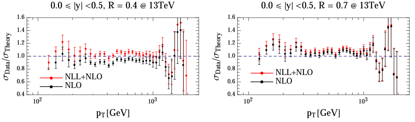
FIG. 5: Same as Fig. 4 for the CMS data of [22] at \sqrt{S} = 13 TeV with R = 0.4 (left) and R = 0.7 (right).
