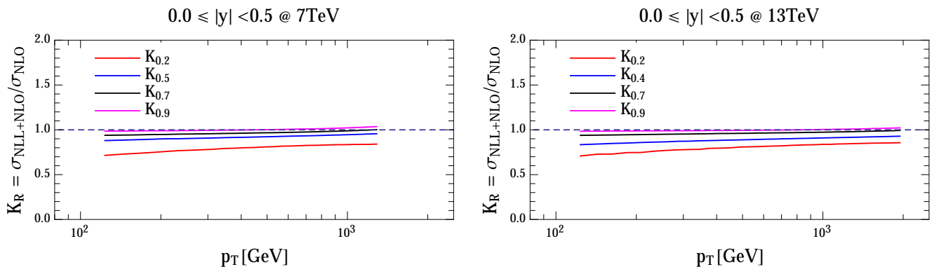
FIG. 1: Cross section ratios K_R of Eq. (4) with different jet radii at \sqrt{S} = 7 TeV (left) and 13 TeV (right) using the MMHT PDF set [64] at NLO.
