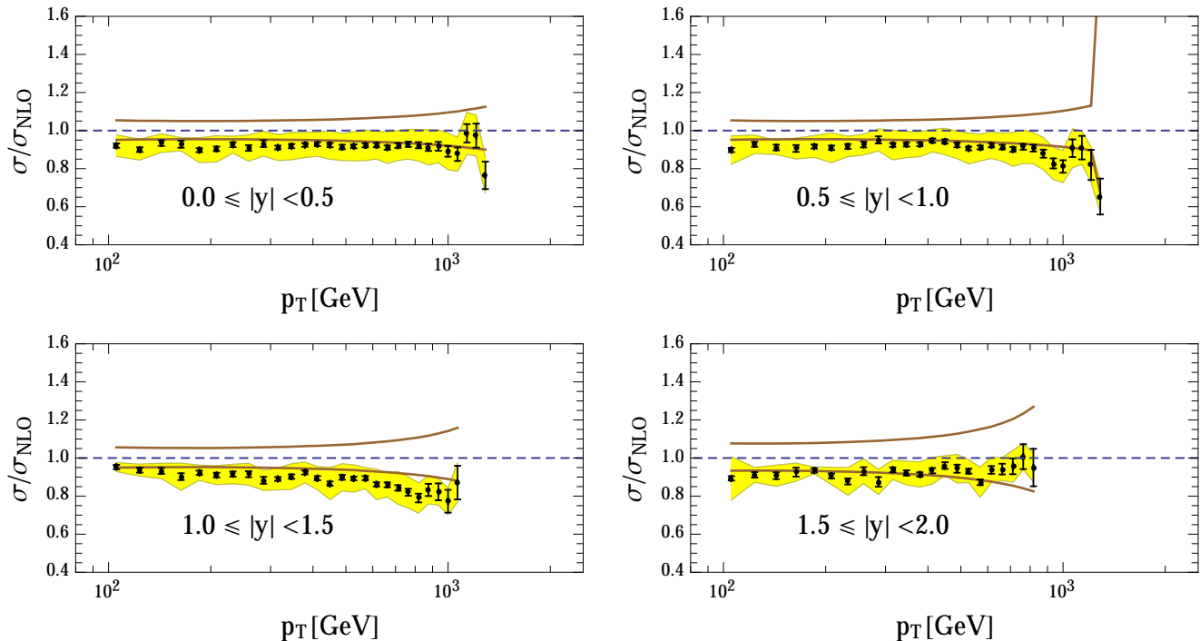
FIG. 8: Same as Fig. 7 for the ratio \sigma_{\text{Data}}/\sigma_{\text{NLO}} .
