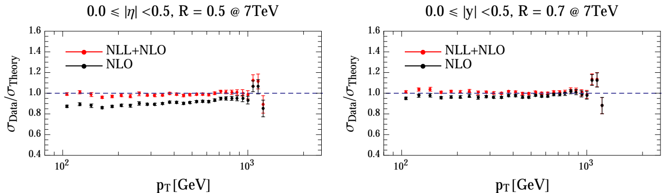
FIG. 4: The ratio \sigma_{\text{Data}}/\sigma_{\text{Theory}} for the CMS data \sqrt{S} = 7 TeV of [17] with R = 0.5 (left) and R = 0.7 (right) to the theoretical results at NLO (black) and at NLO + NLL (red) accuracy using the MMHT PDF set [64] at NLO.
