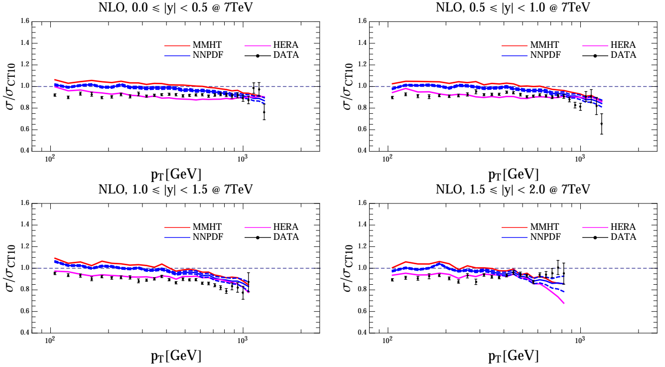
FIG. 13: Same as Fig. 11 for cross sections \sigma_{\text{NLO}} at NLO in pQCD.
