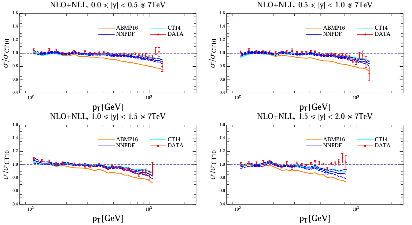
FIG. 12: Same as Fig. 11 for the PDF sets ABMP16 [72], CT14 [70] and NNPDF3.1 [75].
