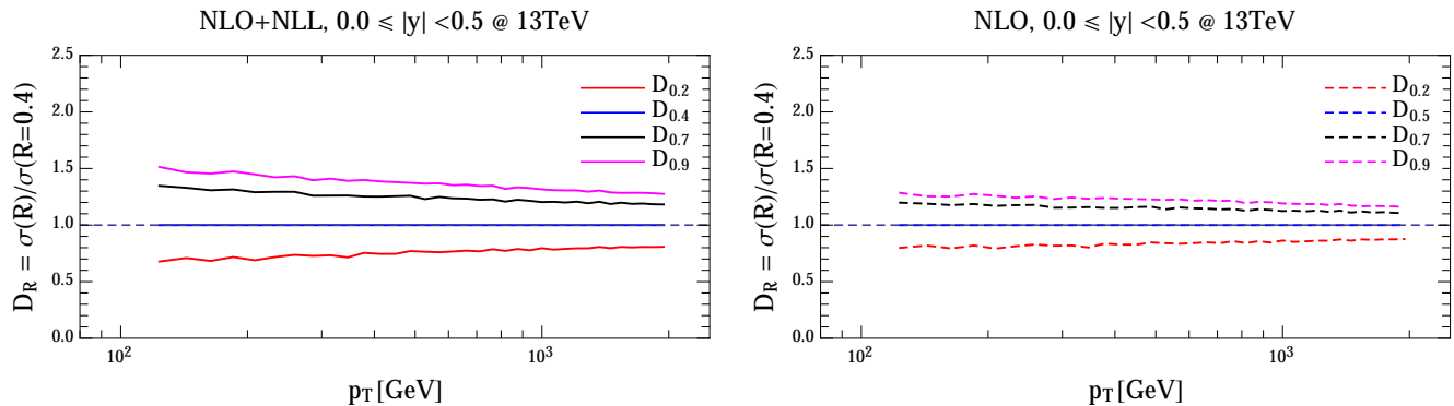
FIG. 3: Ratios D_R of Eq. (5) with R_{\text{fixed}} = 0.4 at \sqrt{S} = 13 TeV for the cross sections at NLO + NLL (left) and NLO (right) accuracy using the MMHT PDF set [64] at NLO.
