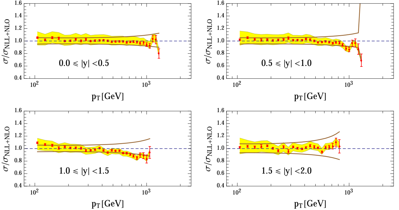
FIG. 7: The ratio \sigma_{\text{Data}}/\sigma_{\text{NLO+NLL}} for the CMS data collected at \sqrt{S} = 7 TeV [17] with R = 0.5 to the theoretical results using the CT10 PDF set [71] at NLO. The error bars represent the experimental statistical errors and the solid (brown) lines the systematic ones. The band (yellow) indicates theoretical scale uncertainties. The NP corrections from [17] have been included.
