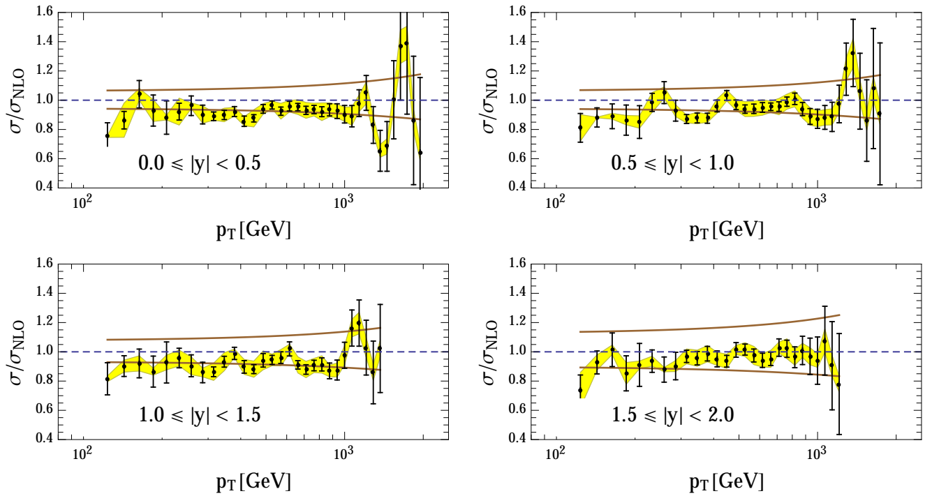
FIG. 10: Same as Fig. 9 for the ratio \sigma_{\text{Data}}/\sigma_{\text{NLO}} .
