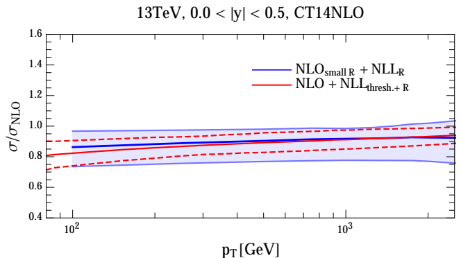
FIG. 6: Comparison of the scale dependence of the jointly resummed cross section (red) and the case where only small- R logarithms are resummed to all orders (blue) [30]. As an example, we use the CT14 PDF set [70] at NLO with R = 0.4 and both results are normalized to NLO. See text for more details.
