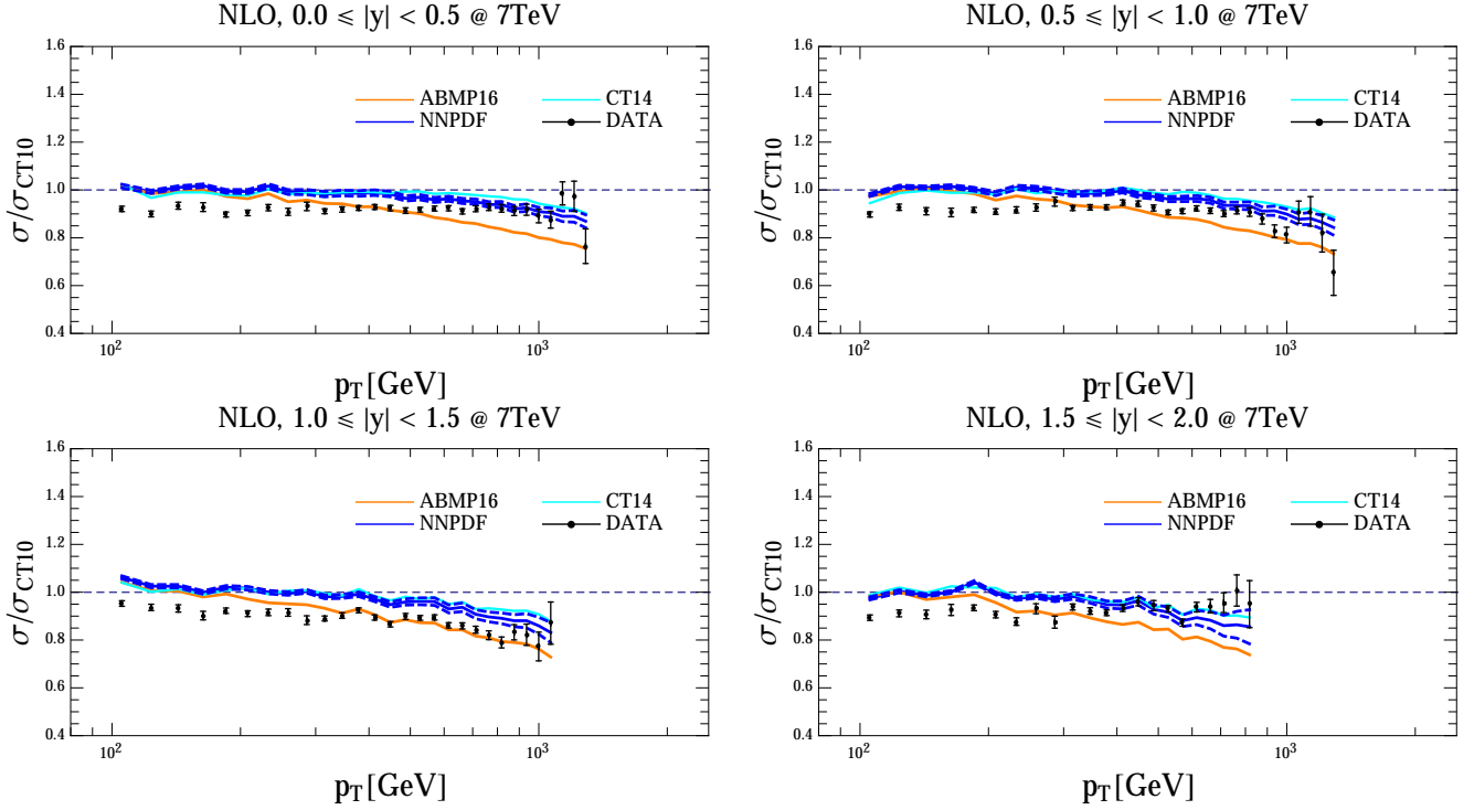
FIG. 14: Same as Fig. 12 for cross sections \sigma_{\text{NLO}} at NLO in pQCD.
