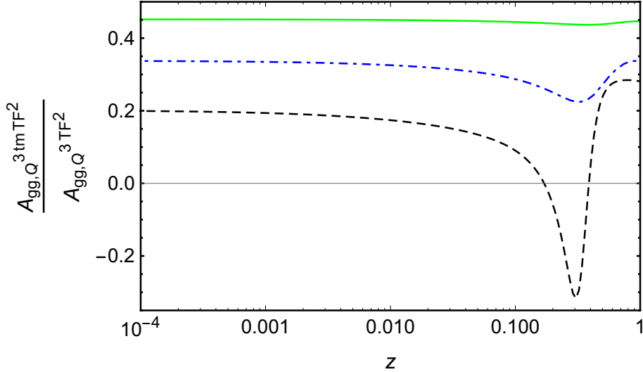
Figure 2: The ratio of the two-mass (tm) contributions to the massive OME A_{gg,Q}^{(3)\text{tm}} to all contributions to A_{gg,Q}^{(3)} of \mathcal{O}(T_F^2) as a function of z and \mu^2 . Dashed line (black): \mu^2 = 50 \text{ GeV}^2 . Dash-dotted line (blue): \mu^2 = 100 \text{ GeV}^2 . Full line (green): \mu^2 = 1000 \text{ GeV}^2 . Here the on-shell heavy quark masses m_c = 1.59 \text{ GeV} and m_b = 4.78 \text{ GeV} [1, 2] have been used.
