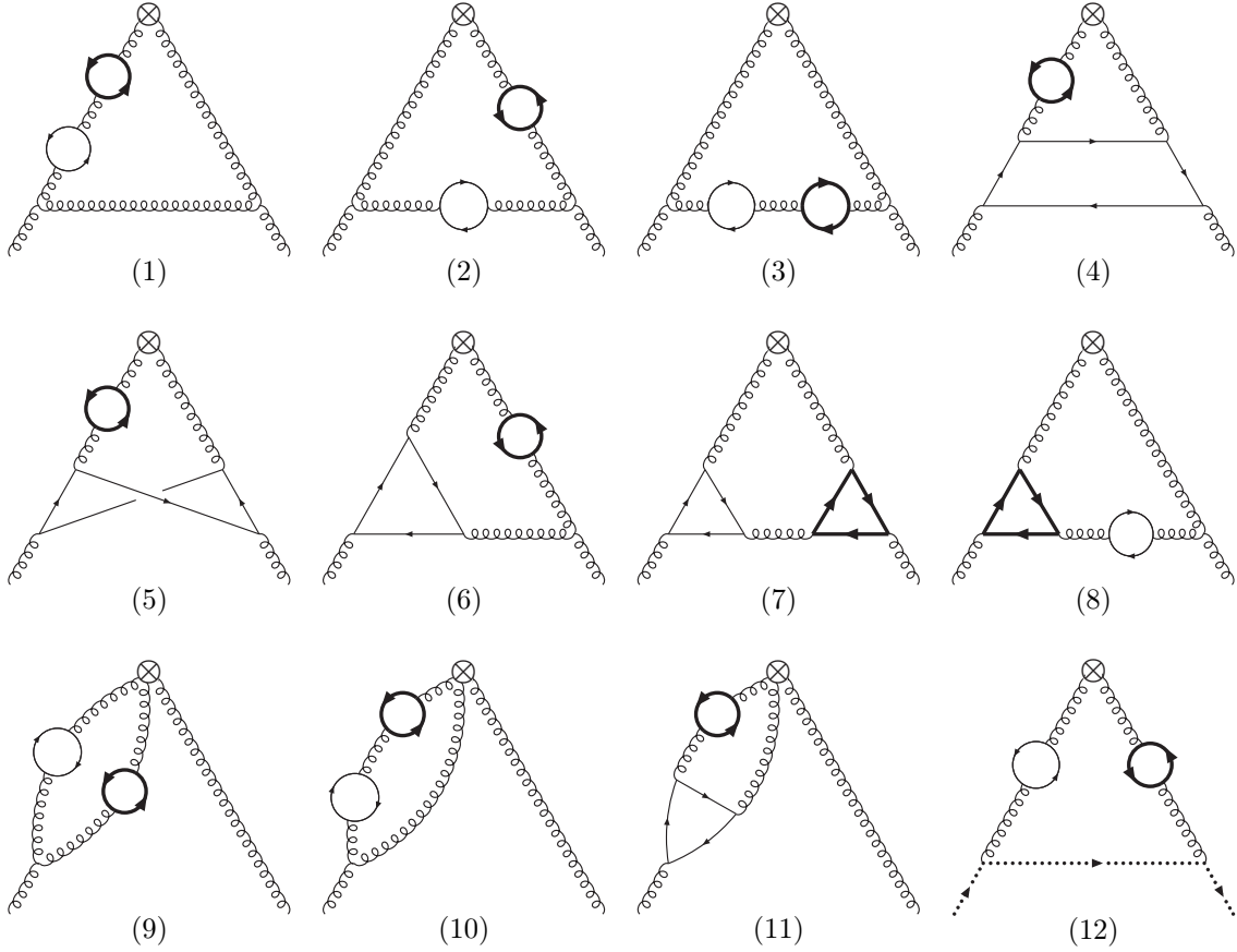
Figure 1: The twelve different topologies for \tilde{A}_{gg,Q}^{(3)} . Curly lines: gluons; dotted lines: ghosts; thin arrow lines: lighter massive quark; thick arrow lines: heavier massive quark; the symbol \otimes represents the corresponding local operator insertion, cf. [35].
