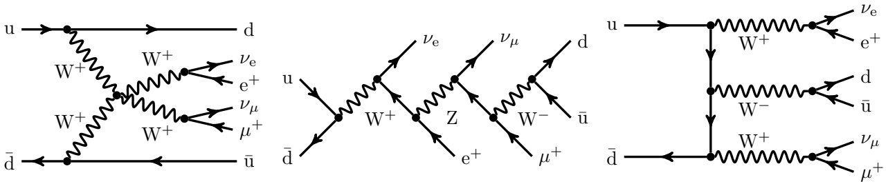
Fig. 1: Sample tree-level diagrams that contribute to the process pp \rightarrow \mu^+\nu_\mu e^+\nu_e jj at order \mathcal{O}(\alpha^6) . In addition to typical VBS contributions (left), this order also possesses s -channel contributions such as decay chain (middle) and tri-boson contributions (right).
