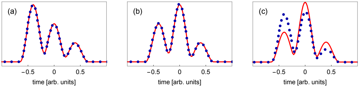
Figure 16: Three cosine-squared pulses of equal width and with uniform spacing. The amplitude ratios are A_2/A_1 = 2/3 , A_3/A_1 = 1/3 . (a) The largest peak is at the front. (b) The largest peak is in the center. The KK phase yields a perfect reconstruction in both cases. (c) For amplitude ratios of A_2/A_1 = 1/2 , A_3/A_1 = 1/3 , the KK reconstruction is perfect when the highest peak is at the front but fails if it is in the center.
