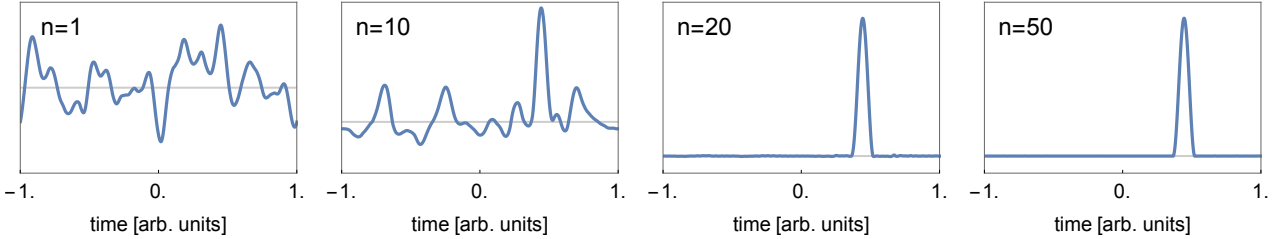
Figure 20: Iterative reconstruction of a cosine-squared charge distribution. Shown are the iteration steps n = 1 , n = 10 , n = 20 and n = 50 .
