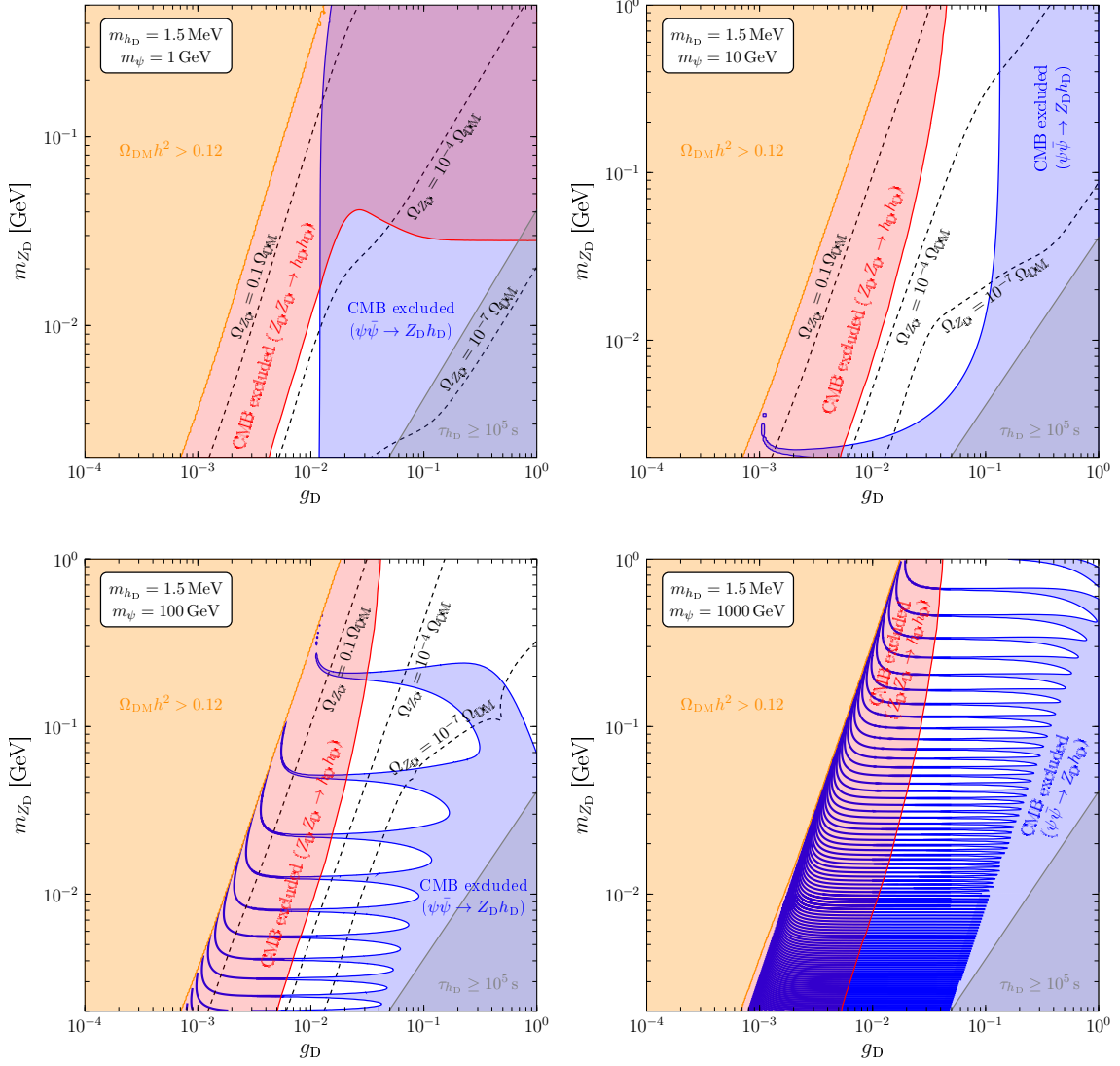
Figure 2. Constraints in the g_{\text{D}}-m_{\text{Z}_{\text{D}}} plane for m_{\psi} = 1 GeV (upper left panel), m_{\psi} = 10 GeV (upper right panel), m_{\psi} = 100 GeV (lower left panel), and m_{\psi} = 1000 GeV (lower right panel). In each case we fix m_{h_{\text{D}}} = 1.5 MeV, and choose the coupling g_{\psi} such that \Omega_{\psi} h^2 + \Omega_{\text{Z}_{\text{D}}} h^2 \simeq 0.12 . In the orange shaded regions the DM density exceeds the observed value irrespective of the value of g_{\psi} . The regions of parameter space excluded by CMB constraints on late-time energy injection are given in blue for the process \psi\bar{\psi} \rightarrow \text{Z}_{\text{D}} h_{\text{D}} and in red for \text{Z}_{\text{D}} \text{Z}_{\text{D}} \rightarrow h_{\text{D}} h_{\text{D}} . In the grey shaded areas, the lifetime of the dark Higgs h_{\text{D}} exceeds 10^5 s, leading to significant spectral distortions in the CMB. Note that the range of m_{\text{Z}_{\text{D}}} shown for m_{\psi} = 1 GeV (upper left plot) is smaller than in the rest of the panels.
