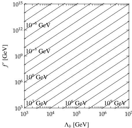
Figure 11. Contours of m_\phi in the f' - \Lambda_b plane. The thick lines correspond to the indicated labels.
