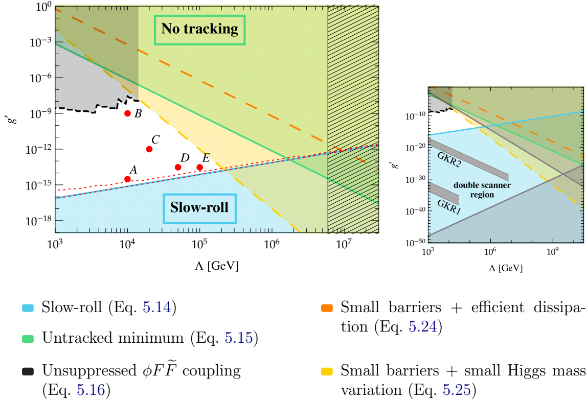
Figure 8. Summary of the available region of parameter space in the g' - \Lambda plane consistent with the relaxation mechanism exploiting particle production instead of inflation. Constraints come from Eqs. (5.14)–(5.16), (5.24) and (5.25). The red dots correspond to the five benchmark cases of Fig. 9. The dashed lines correspond to the bounds which rely on conservative assumptions about the thermalisation process. The region between the red dotted lines corresponds to the one in which the inflaton is allowed to reheat the SM before relaxation takes place (see Fig. 3). The rectangular hashed region at large \Lambda is the one in which the approximation of instantaneous particle production fails. Right plot: This smaller plot indicates in comparison the parameter space relevant for the two original relaxation models (GKR1 for the relaxation being the QCD axion and GKR2 for the model with strong dynamics at the weak scale) proposed in [1]) as well as for the double-scanner mechanism of Ref. [2], which all use inflation as a source of friction.
