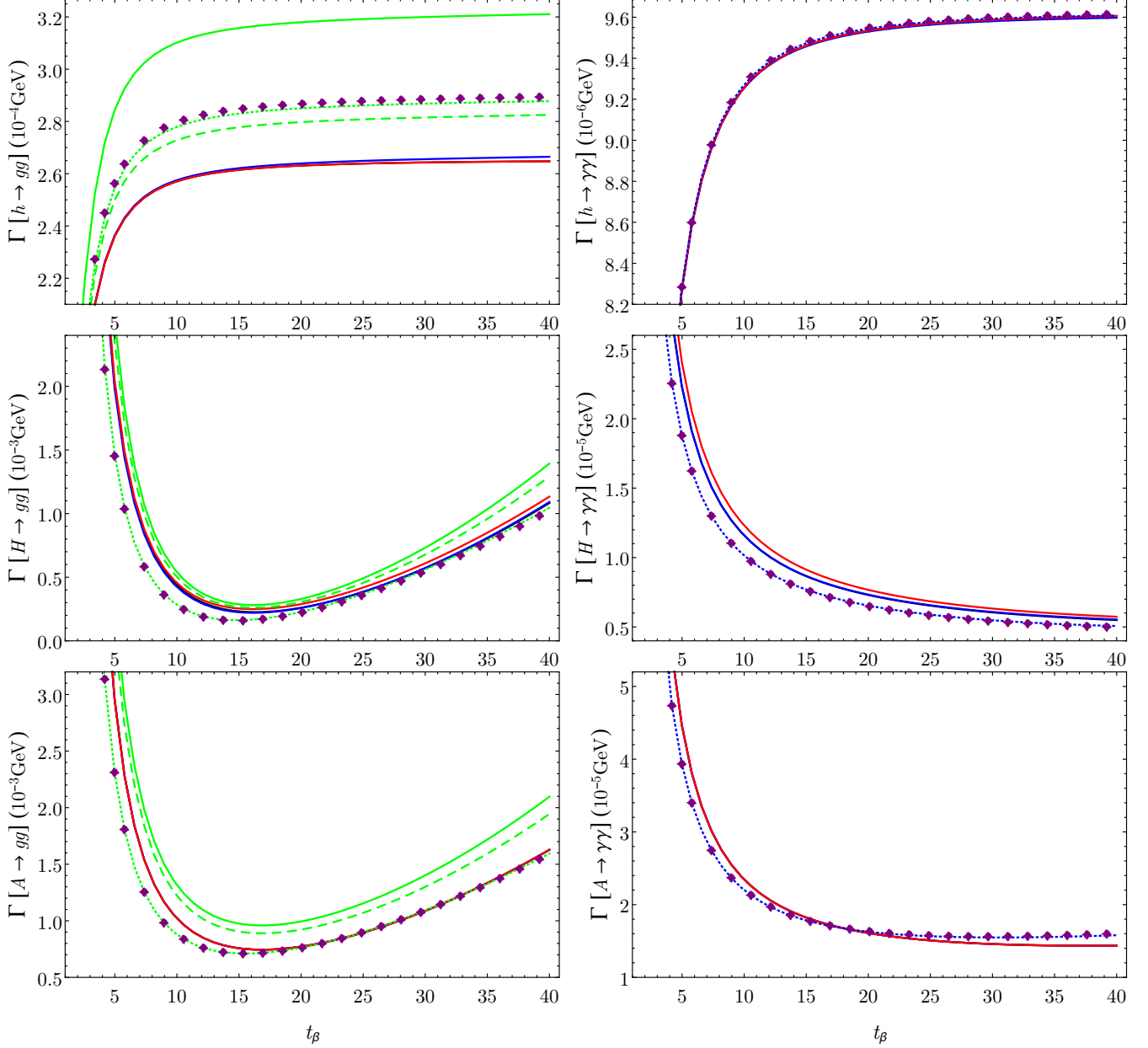
Figure 4: Comparison with FeynHiggs of the decay widths of the doublet Higgs states into gg and \gamma\gamma in the MSSM-limit of the NMSSM. The input parameters are provided in Tab. 1. The black, blue and red curves correspond to a rotation to the physical Higgs states via \mathbf{U}^0 , \mathbf{U}^m and \mathbf{X} respectively. In the case of the gg final state, these lines are obtained for three radiated quark flavors in the QCD corrections. The green curves are obtained for five radiated quark flavors, employing universal QCD corrections at NLO (dashed) or beyond (solid). Furthermore the dotted green line shows the widths for NLO QCD-correction factors and \overline{\text{MS}} quark masses, which is the current approach of FeynHiggs (purple diamonds). In the case of the diphoton final state, the dashed lines are obtained with QCD corrections in the approximation of heavy quarks/squarks and \overline{\text{MS}} masses like in the current version of FeynHiggs .
