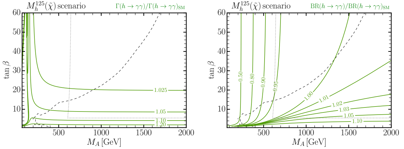
Figure 6: Left: Decay width of the lighter \mathcal{CP} -even scalar into photons as a function of M_A and \tan\beta in the M_h^{125}(\tilde{\chi}) scenario, normalized to the corresponding width of a SM Higgs boson of the same mass. Right: same as the left plot for the branching ratio of the decay h \rightarrow \gamma\gamma . In each plot, the boundaries of the blue and the hatched exclusion regions of Fig. 5 are also shown as a dashed and a dotted black line, respectively.
