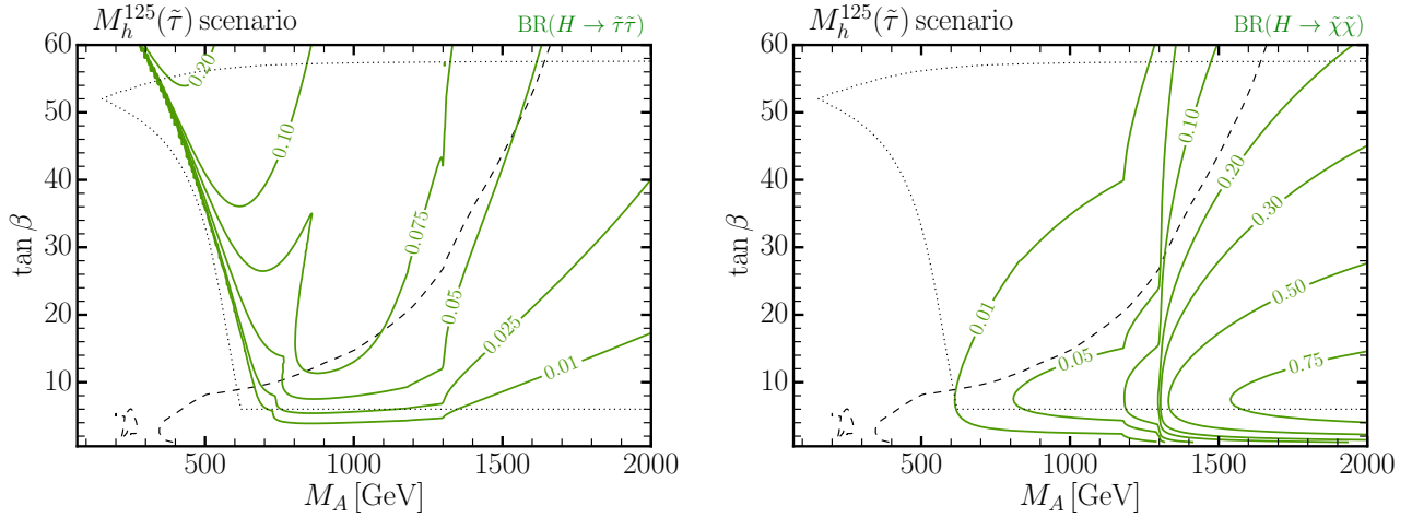
Figure 4: Left: Total branching ratio for the decays of the heavier \mathcal{CP} -even scalar H into stau pairs, as a function of M_A and \tan\beta in the M_h^{125}(\tilde{\tau}) scenario. Right: same as the left plot for the total branching ratio of the decays of H into chargino or neutralino pairs. In each plot, the boundaries of the blue and the hatched exclusion regions of Fig. 2 are also shown as a dashed and a dotted black line, respectively.
