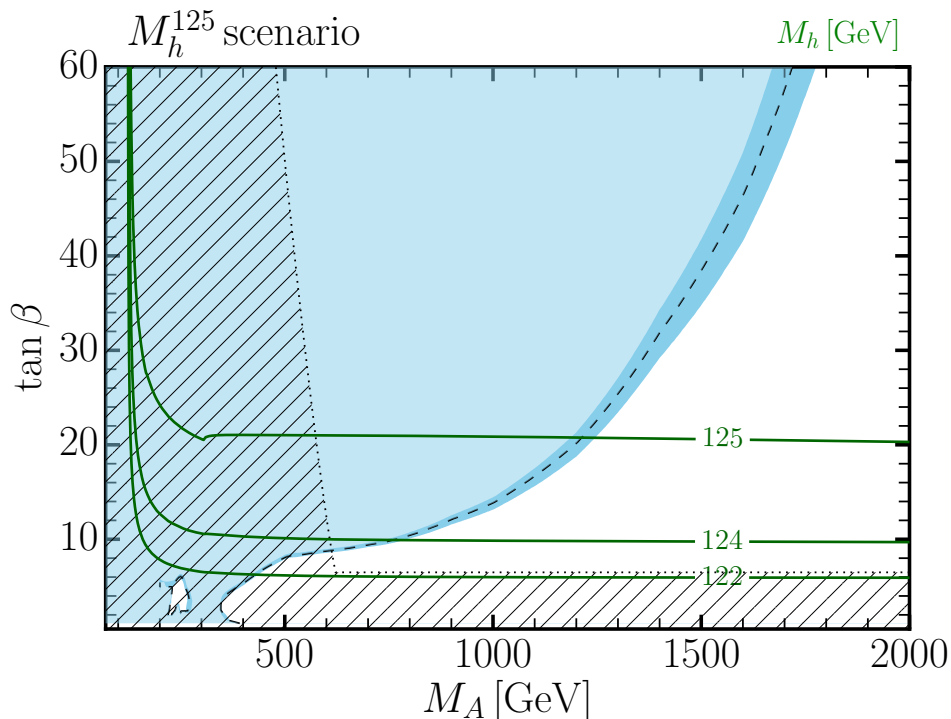
Figure 1: Constraints on the M_h^{125} scenario from Higgs searches at the LHC, in the (M_A, \tan \beta) plane. The green solid lines are predictions for the mass of the lighter \mathcal{CP} -even scalar h , the hatched area is excluded by a mismatch between the properties of h and those of the observed Higgs boson, and the blue area is excluded by the searches for additional Higgs bosons (the darker-blue band shows the theoretical uncertainty of the exclusion).
