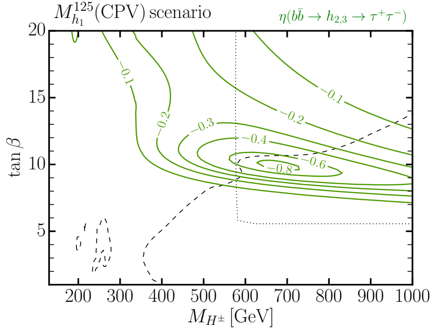
Figure 13: The same exclusion boundaries as in Fig. 12 above are overlaid with contours of the relative interference factor \eta(b\bar{b} \rightarrow h_{2,3} \rightarrow \tau^+\tau^-) defined in Eq. (2).
