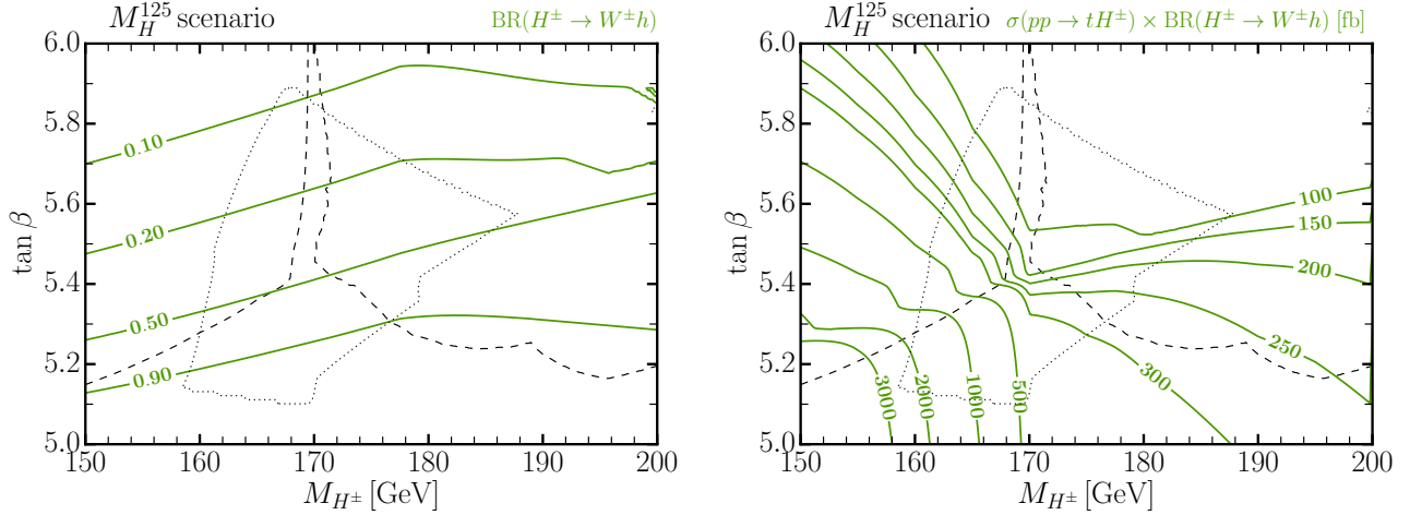
Figure 11: Left: Branching ratio for the decay H^\pm \rightarrow W^\pm h as a function of M_{H^\pm} and \tan\beta in the M_H^{125} scenario. Right: Total rate (in fb) for the production of a charged Higgs boson in association with a top quark, followed by the decay to a W^\pm h pair, at the LHC with 13 TeV center-of-mass energy. In each plot, the boundaries of the exclusion regions from Fig. 10 are shown as a dashed and a dotted black line, respectively.
