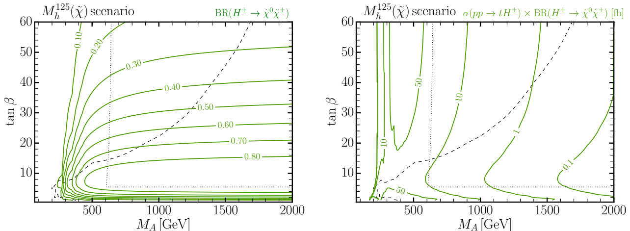
Figure 8: Left: Branching ratio for the charged-Higgs decays to chargino–neutralino pairs, as a function of M_A and \tan\beta in the M_h^{125}(\tilde{\chi}) scenario. A sum is taken over all the kinematically allowed combinations of particles in the final state. Right: Total rate (in fb) for the production of a charged Higgs boson in association with a top quark, followed by its decay to EW-inos, at the LHC with 13 TeV center-of-mass energy. In each plot, the boundaries of the blue and the hatched exclusion regions of Fig. 5 are shown as a dashed and a dotted black line, respectively.
