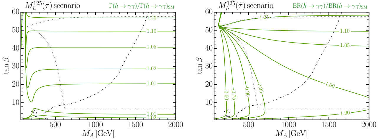
Figure 3: Left: Decay width of the lighter \mathcal{CP} -even scalar into photons as a function of M_A and \tan\beta in the M_h^{125}(\tilde{\tau}) scenario, normalized to the corresponding width of a SM Higgs boson of the same mass. Right: same as the left plot for the branching ratio of the decay h \rightarrow \gamma\gamma . In each plot, the boundaries of the blue and the hatched exclusion regions of Fig. 2 are also shown as a dashed and a dotted black line, respectively.
