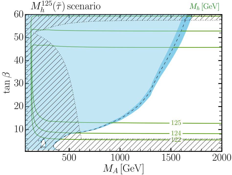
Figure 2: Constraints on the M_h^{125}(\tilde{\tau}) scenario from Higgs searches at the LHC, in the (M_A, \tan \beta) plane. The green solid lines are predictions for the mass of the lighter \mathcal{CP} -even scalar h , the hatched area is excluded by a mismatch between the properties of h and those of the observed Higgs boson, and the blue area is excluded by the searches for additional Higgs bosons (the darker-blue band shows the theoretical uncertainty of the exclusion).
