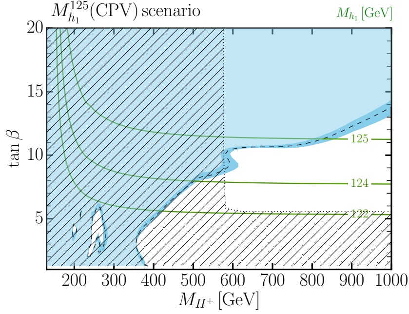
Figure 12: Constraints on the M_{h_1}^{125} (CPV) scenario from Higgs searches at the LHC, in the (M_{H^\pm}, \tan\beta) plane. The green solid lines are predictions for the mass of the lightest neutral scalar h_1 , the hatched area is excluded by a mismatch between the properties of h_1 and those of the observed Higgs boson, and the blue area is excluded by the searches for additional Higgs bosons (the darker-blue band shows the theoretical uncertainty of the exclusion).
