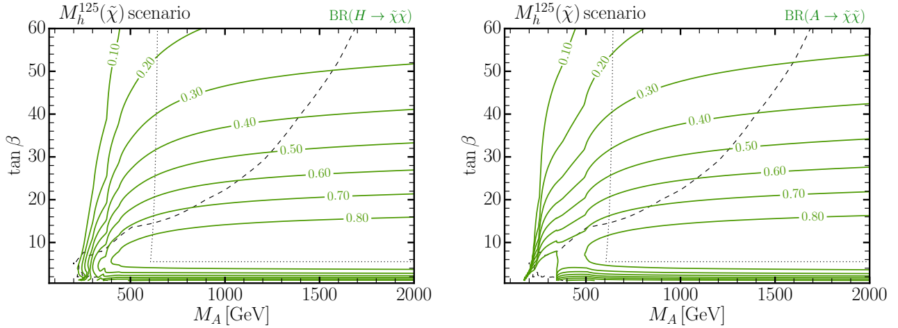
Figure 7: Branching ratio for the decays of the heavier \mathcal{CP} -even scalar H (left) or the \mathcal{CP} -odd scalar A (right) into EW-ino pairs, as a function of M_A and \tan\beta in the M_h^{125}(\tilde{\chi}) scenario. A sum is taken over all the kinematically allowed combinations of particles in the final state. In each plot, the boundaries of the blue and the hatched exclusion regions of Fig. 5 are also shown as a dashed and a dotted black line, respectively.
