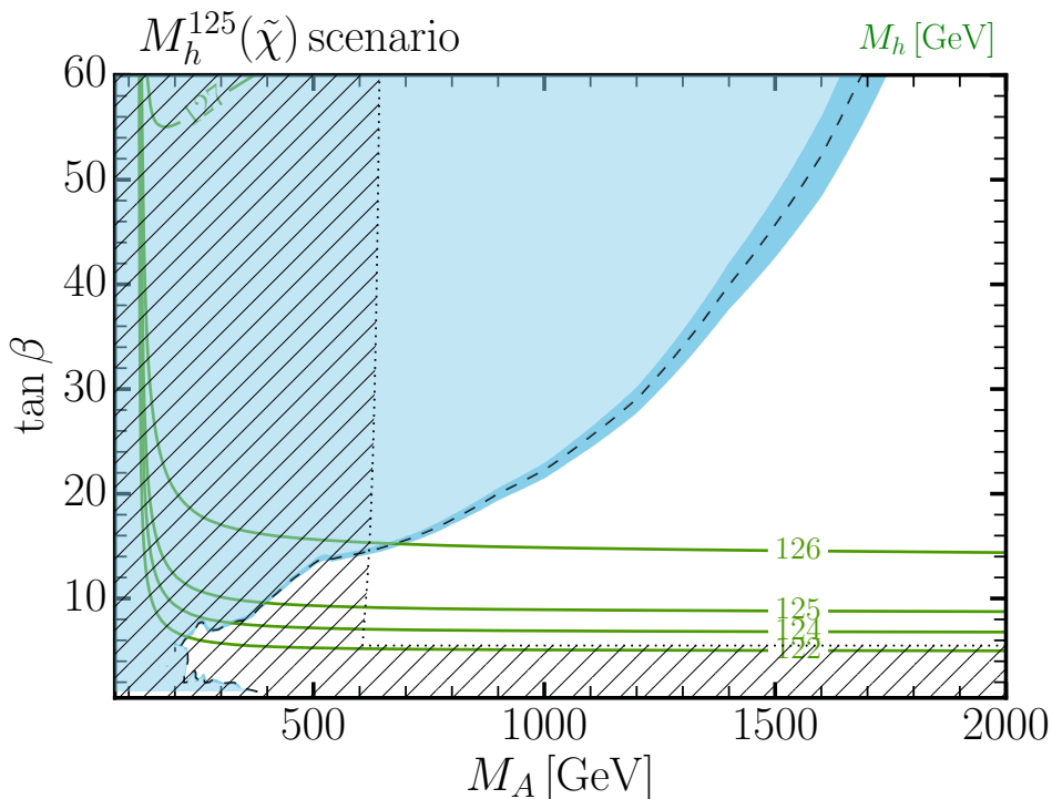
Figure 5: Constraints on the M_h^{125}(\tilde{\chi}) scenario from Higgs searches at the LHC, in the (M_A, \tan \beta) plane. The green solid lines are predictions for the mass of the lighter \mathcal{CP} -even scalar h , the hatched area is excluded by a mismatch between the properties of h and those of the observed Higgs boson, and the blue area is excluded by the searches for additional Higgs bosons (the darker-blue band shows the theoretical uncertainty of the exclusion).
