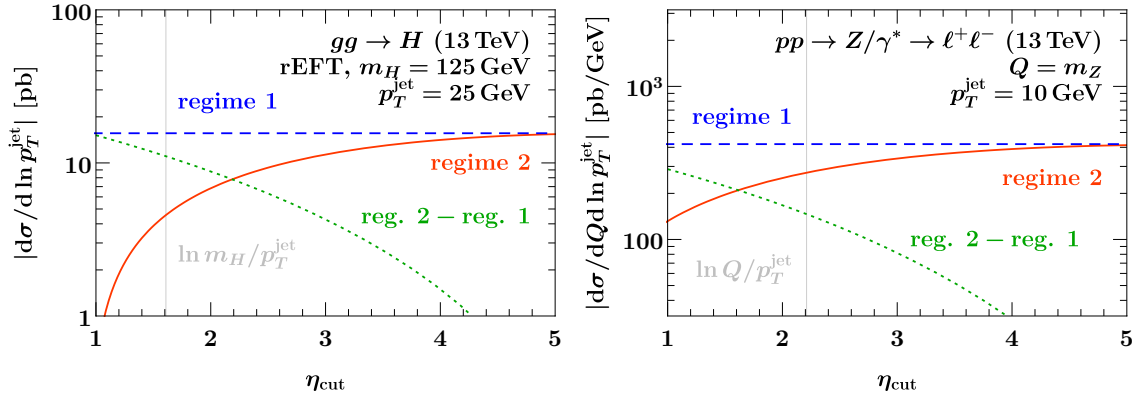
Figure 3. Comparison of the singular contributions to the fixed \mathcal{O}(\alpha_s) (LO 1 ) p_T^{\text{jet}} spectrum for gg \rightarrow H (left) and Drell-Yan (right). The orange solid lines show the singular contributions in regime 2 with \eta_{\text{cut}} dependent beam functions. The dashed blue lines show the singular contributions in regime 1 in the limit \eta_{\text{cut}} = \infty , p_T^{\text{cut}} \gg Qe^{-\eta_{\text{cut}}} . Their difference, shown by the dotted green lines, correctly scales as a power in Qe^{-\eta_{\text{cut}}}/p_T^{\text{jet}} . The vertical lines indicate the point p_T^{\text{jet}} = Qe^{-\eta_{\text{cut}}} .
