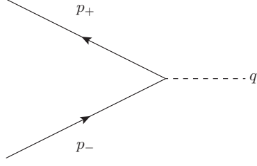
Figure 1: The Born cross section for the process e^+e^- \rightarrow Z^*/\gamma^* .
