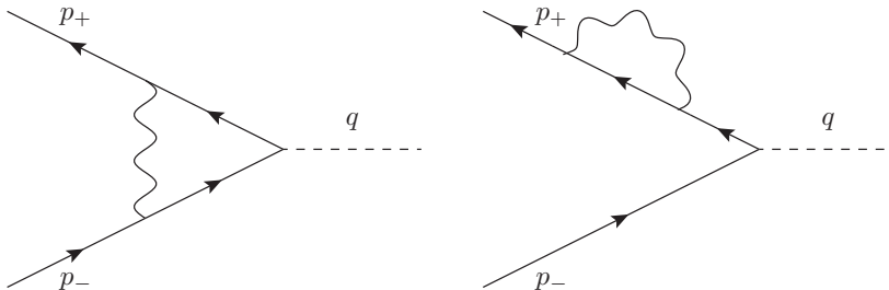
Figure 3: The O(\alpha) virtual corrections to e^+e^- annihilation into virtual gauge boson.
