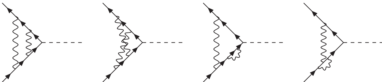
Figure 5: The double virtual corrections of O(a^2) to e^+e^- annihilation into a virtual gauge boson. The external self-energy corrections are not shown.
