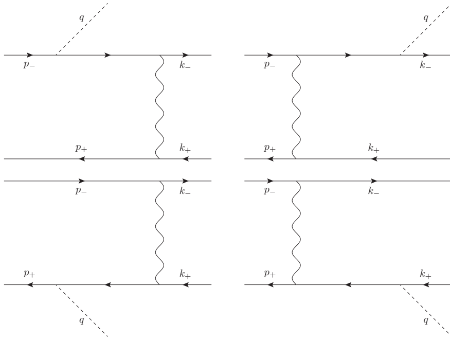
Figure 8: The e^+e^- annihilation graphs into a fermion pair and a gauge boson (process A ).
