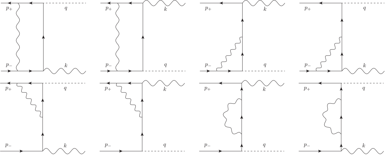
Figure 6: The O(a^2) virtual corrections to e^+e^- annihilation graphs into one photon and a virtual gauge boson. The external self-energy corrections are not shown.
