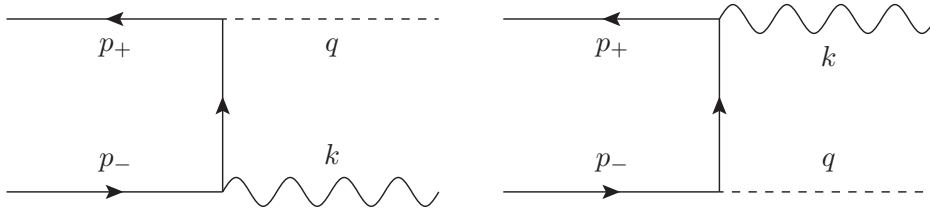
Figure 2: The O(\alpha) e^+e^- annihilation graphs into a photon and a virtual gauge boson.
