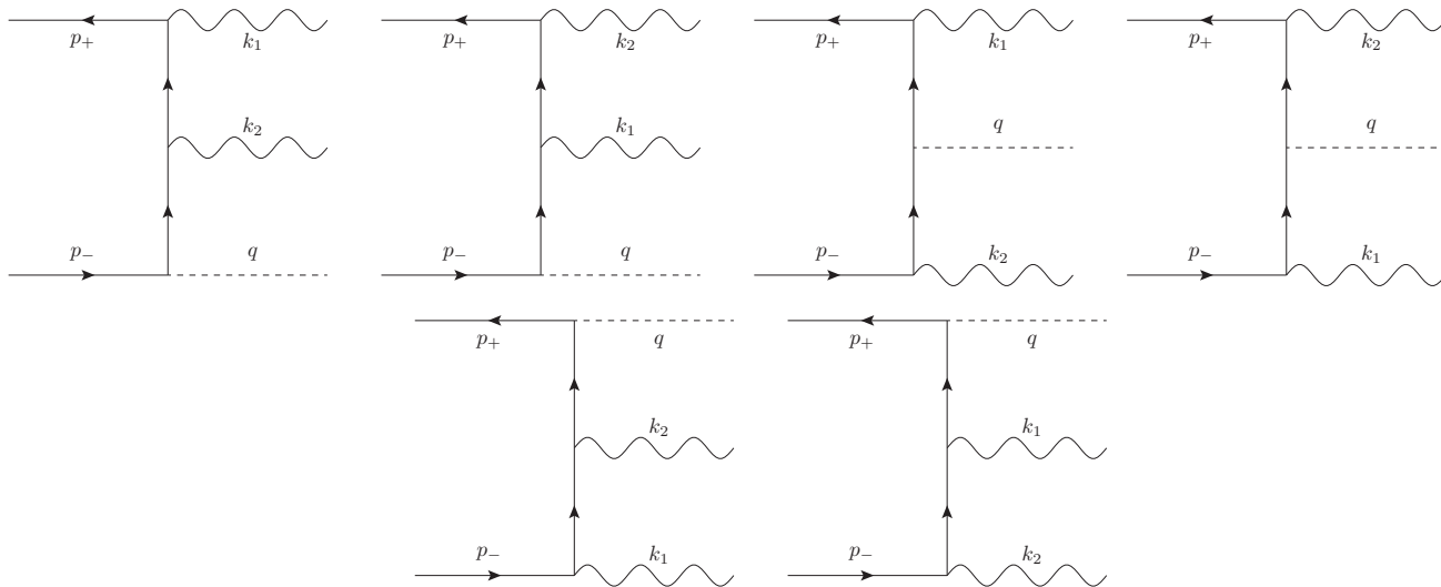
Figure 4: The e^+e^- annihilation graphs into two photons and a virtual gauge boson.
