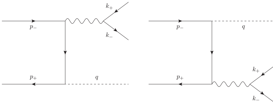
Figure 7: The e^+e^- annihilation graphs into a fermion pair and a gauge boson (process A).
