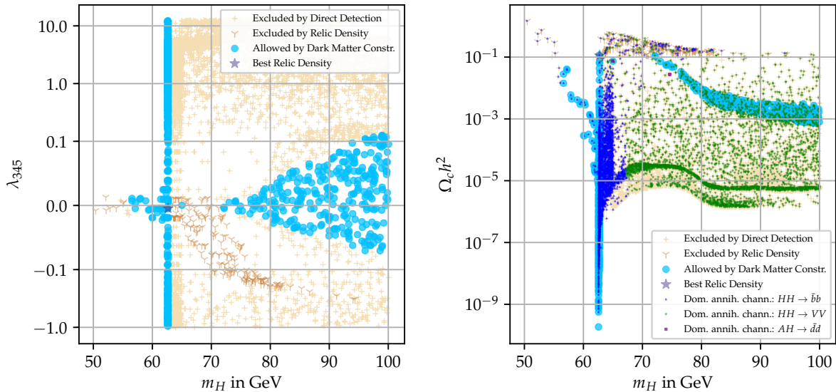
FIG. 3. Parameter space after including dark matter relic density and direct detection constraints. Left: allowed and forbidden regions in the (m_H, \lambda_{345}) plane. Right: Constraints in the (m_H, \Omega_c h^2) plane. On the right plot, we also show the dominant annihilation cross section for each parameter point. The “Best Relic Density” point yields \Omega_c h^2 = 0.1141 which is the closest to the nominal Planck value, c.f. Eq. (18), out of all tested points.
