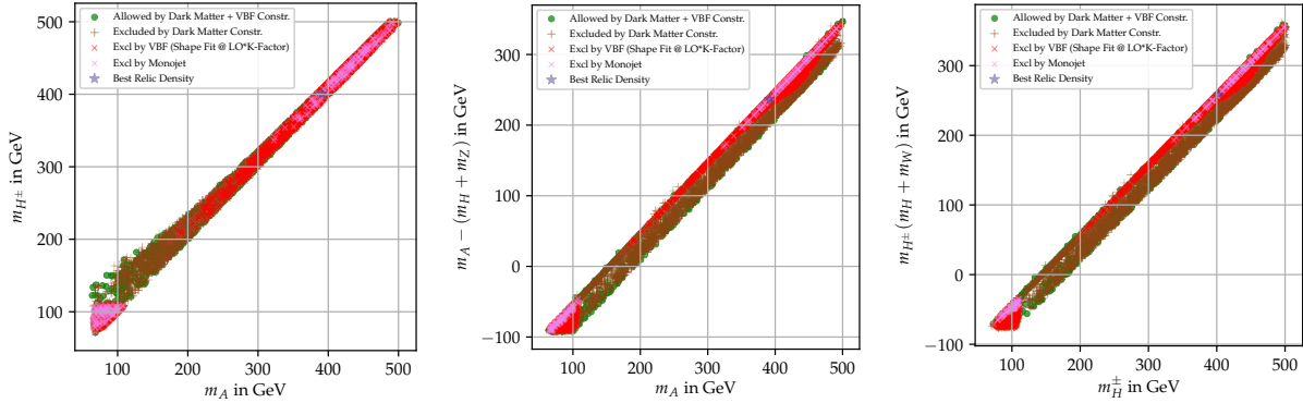
FIG. 5. Allowed combinations of the scalar masses m_{H^\pm} , m_A and m_H which are relevant for collider analysis of the channels pp \rightarrow HA and pp \rightarrow H^\pm A .
