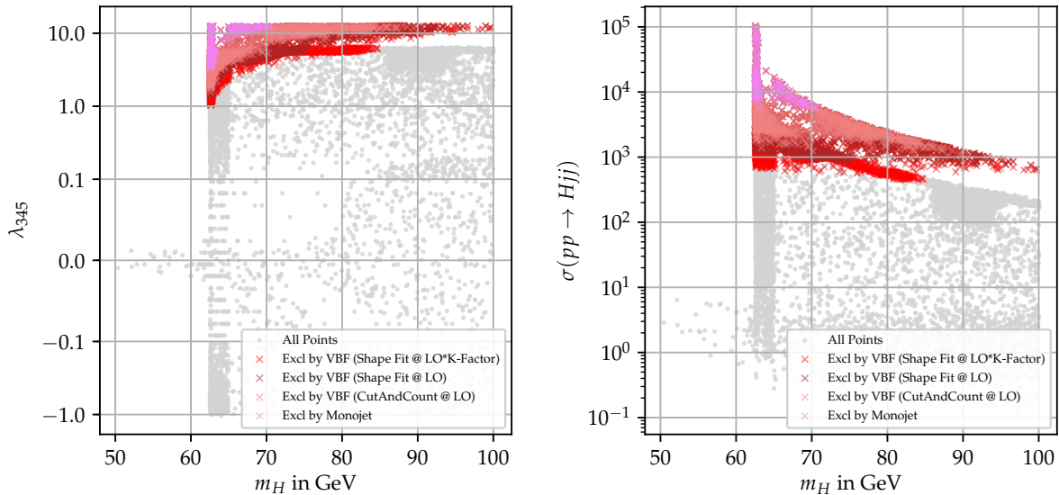
FIG. 2. Allowed and excluded points after consideration of VBF and monojet analysis but without dark matter relic density and direct detection constraints. VBF results are shown using different results, see in-text discussion. Left : Results in (m_H, \lambda_{345}) parameter plane. Right : Results in m_H - \sigma plane where \sigma is the LHC VBF production cross sections at 13 TeV including the partonic cuts given in Sec. IV.2.
