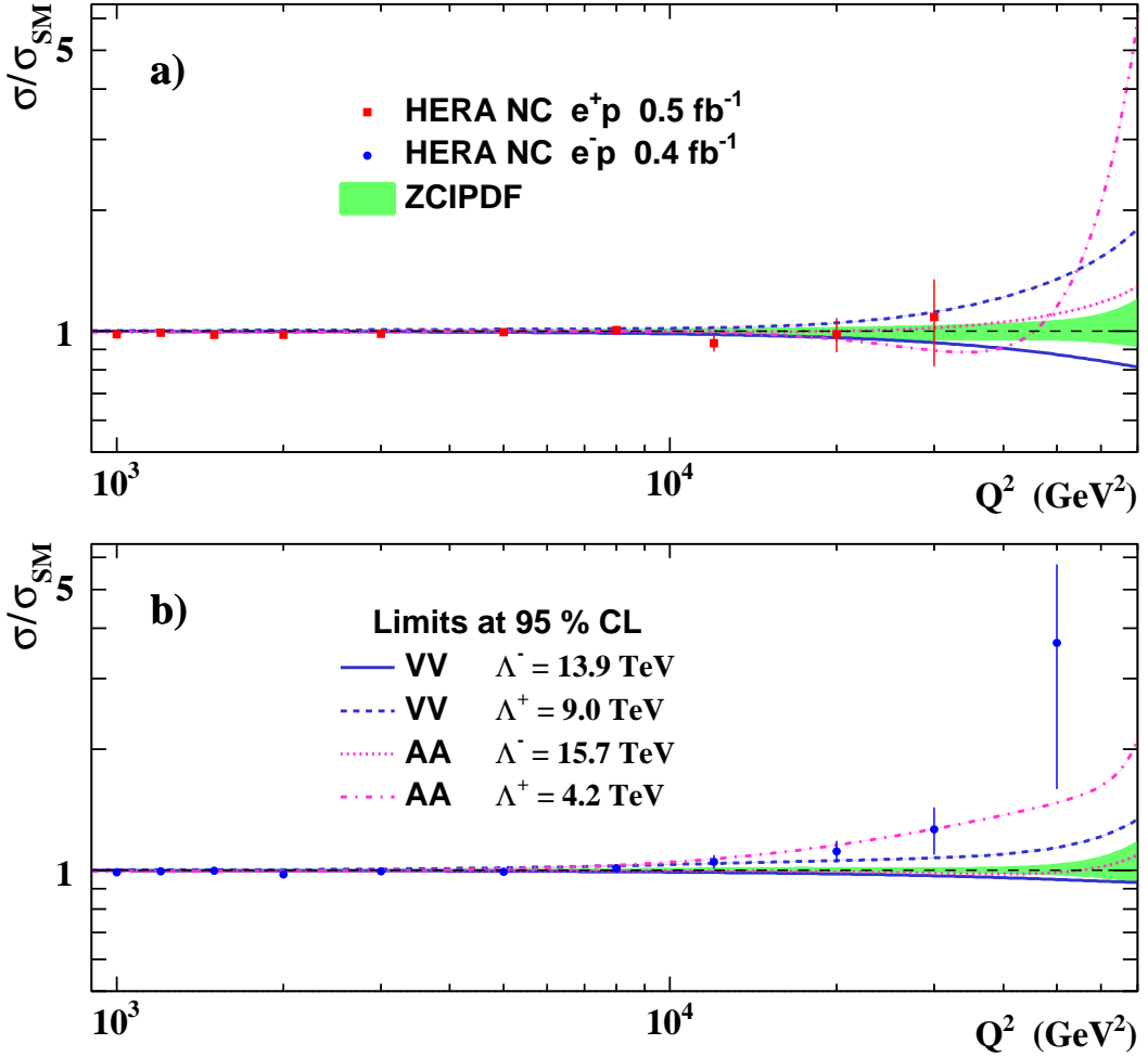
Figure 4: HERA (a) e^+p and (b) e^-p NC DIS data, relative to the SM expectations based on the ZCIPDF fit to the HERA inclusive data, compared to expectations from the VV and AA contact-interaction models with the effective mass scale for positive ( \Lambda^+ ) and negative ( \Lambda^- ) couplings corresponding to the 95% C.L. limits. The same four models are shown on both plots. The bands represent the total uncertainty on the ZCIPDF fit predictions.
