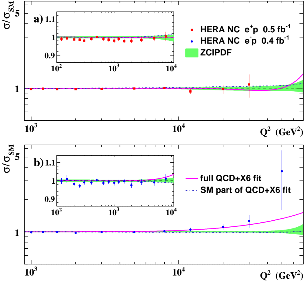
Figure 1: Result of the simultaneous QCD+CI fit to the HERA inclusive data, for the X6 CI model, compared to the combined HERA (a) e^+p and (b) e^-p NC DIS data, relative to the SM expectations based on the QCD fit without the CI contribution (ZCIPDF). The bands represent the total uncertainty of the SM expectations. Also shown is the SM contribution to the cross section resulting from the combined fit.
