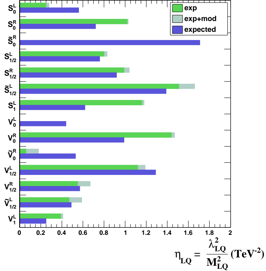
Figure 5: Upper 95% C.L. limits on the LQ coupling strength, \eta_{LQ} = \lambda_{LQ}^2/M_{LQ}^2 . Compared are the limits calculated without (dark upper bars) and with (light upper bars) modelling uncertainties, and the expected limits (lower bars).
