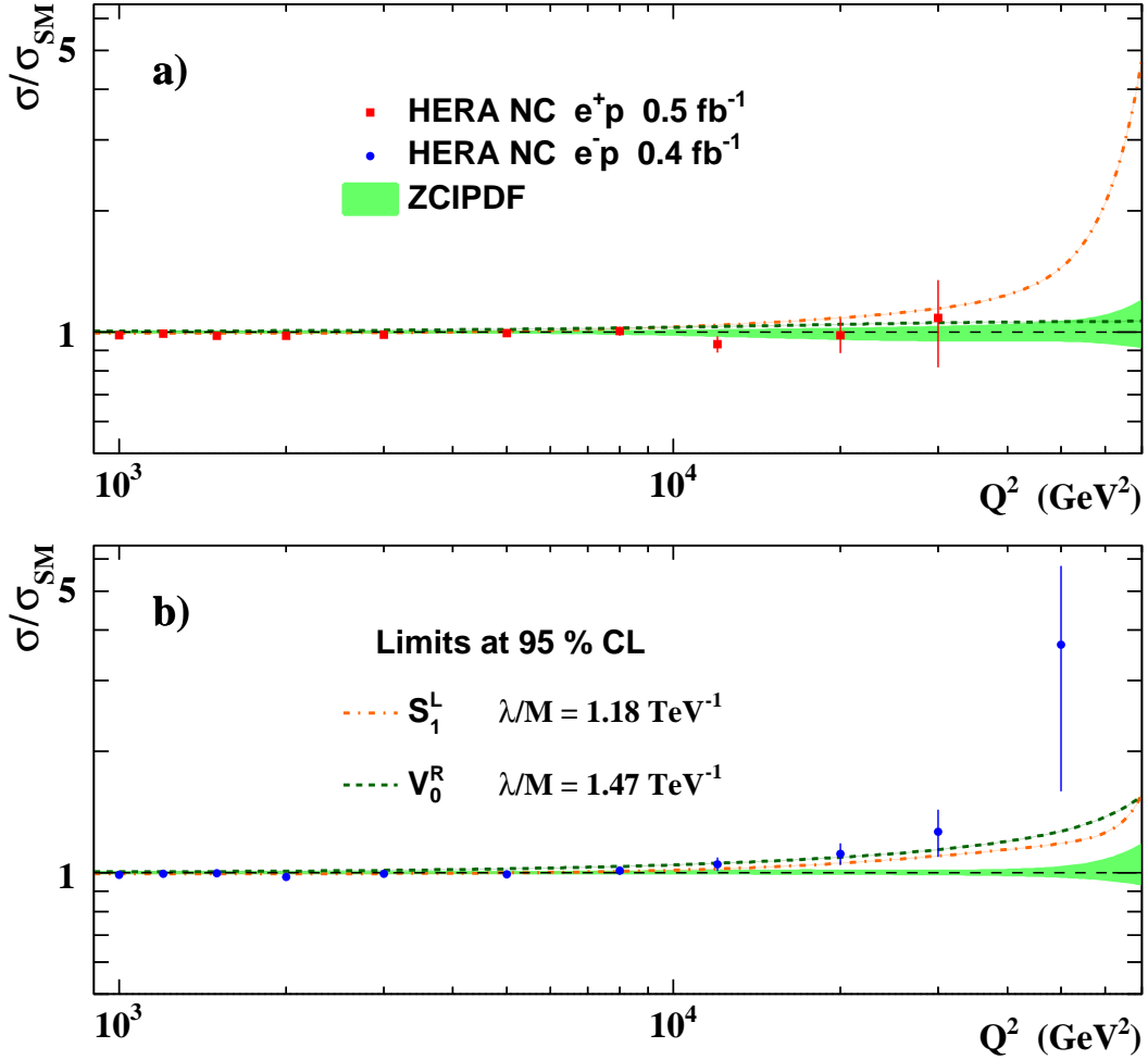
Figure 6: HERA (a) e^+p and (b) e^-p NC DIS data, relative to the SM expectations based on the ZCIPDF fit to the HERA inclusive data, compared to expectations from the S_1^L and V_0^R leptoquark models with the ratios of the LQ Yukawa couplings to the LQ mass, \lambda/M , corresponding to the 95% C.L. limits. The same two models are shown on both plots. The bands represent the total uncertainty on the ZCIPDF fit predictions.
