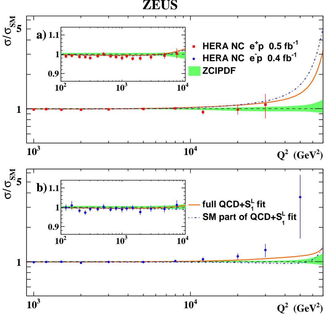
Figure 2: Result of the simultaneous QCD+LQ fit to the HERA inclusive data, for the S_1^L LQ model in the contact interaction limit, M_{LQ} \gg \sqrt{s} , compared to the combined HERA (a) e^+p and (b) e^-p NC DIS data, relative to the SM expectations based on the QCD fit without the CI contribution (ZCIPDF). The bands represent the total uncertainty of the SM expectations. Also shown is the SM contribution to the cross section resulting from the combined fit.
