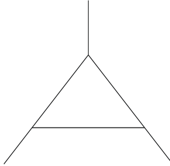
Fig. B.32: One loop 3-point master integral I_1(x, y) .
