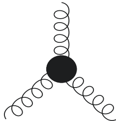
Fig. B.31: Triple gluon vertex function.
