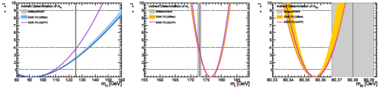
Fig. C.8: Comparisons of \chi^2 distributions for scanning different observables using the Gfitter and the GAPP using the current experimental values and uncertainties. The theoretical uncertainties are indicated by the filled blue and yellow areas, respectively.
