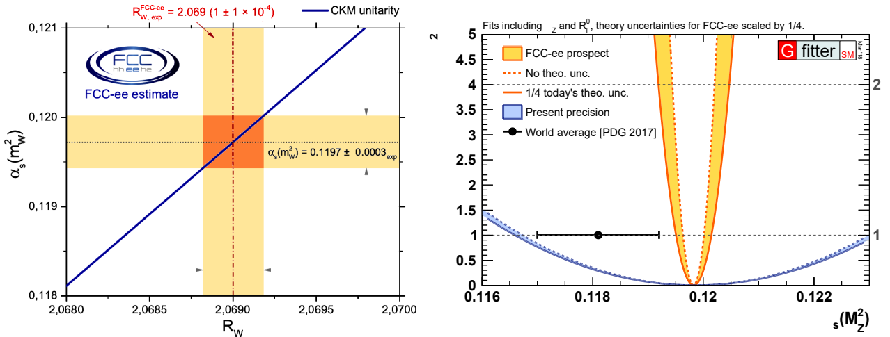
Fig. B.18: Left: Expected \alpha_s determination from the W hadronic-to-leptonic decay ratio ( R_\ell^W ) at the FCC-ee (the diagonal blue line assumes CKM matrix unitarity) [28]. Right: Precision on \alpha_s derived from the electroweak fit today (blue band) [31] and expected at the FCC-ee (yellow band, without theoretical uncertainties and with the current theoretical uncertainties divided by a factor of four).
