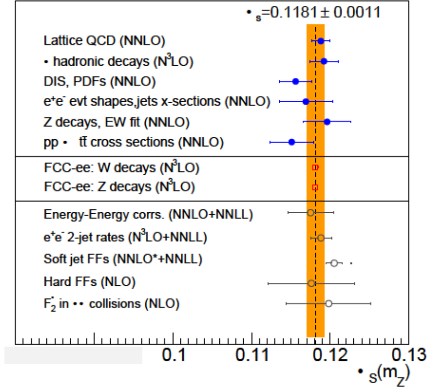
Fig. B.19: Summary of the \alpha_s(m_Z) determinations discussed here. Upper: Subclasses entering in the current PDG world-average (solid dots, orange band) whose numerical value is listed on top [10]. Middle: Expected FCC-ee values via W, Z hadronic decays (open squares). Lower: Other methods based on e^+e^- data not (yet) in the \alpha_s(m_Z) world-average: recent EEC [40] and 2-jet rates [41], plus other extractions at a (currently) lower level of theoretical accuracy.
