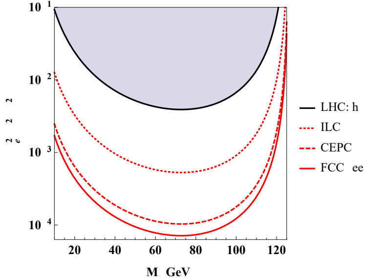
Fig. E.3: Estimated sensitivities on the heavy sterile neutrino properties from the decay H \rightarrow W^+W^- , assuming 10 years of data taking. The black line denotes the bound from the LHC coming from H \rightarrow \gamma\gamma with up to 2015 data. Taken from Ref. [25].
