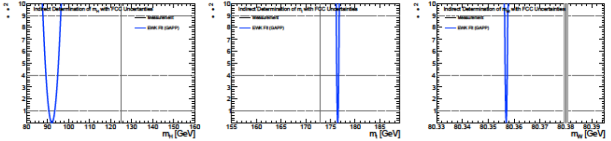
Fig. C.9: Comparisons of \chi^2 distributions for scanning different observables using GAPP with the current experimental values and but the expected uncertainties from FCC.
