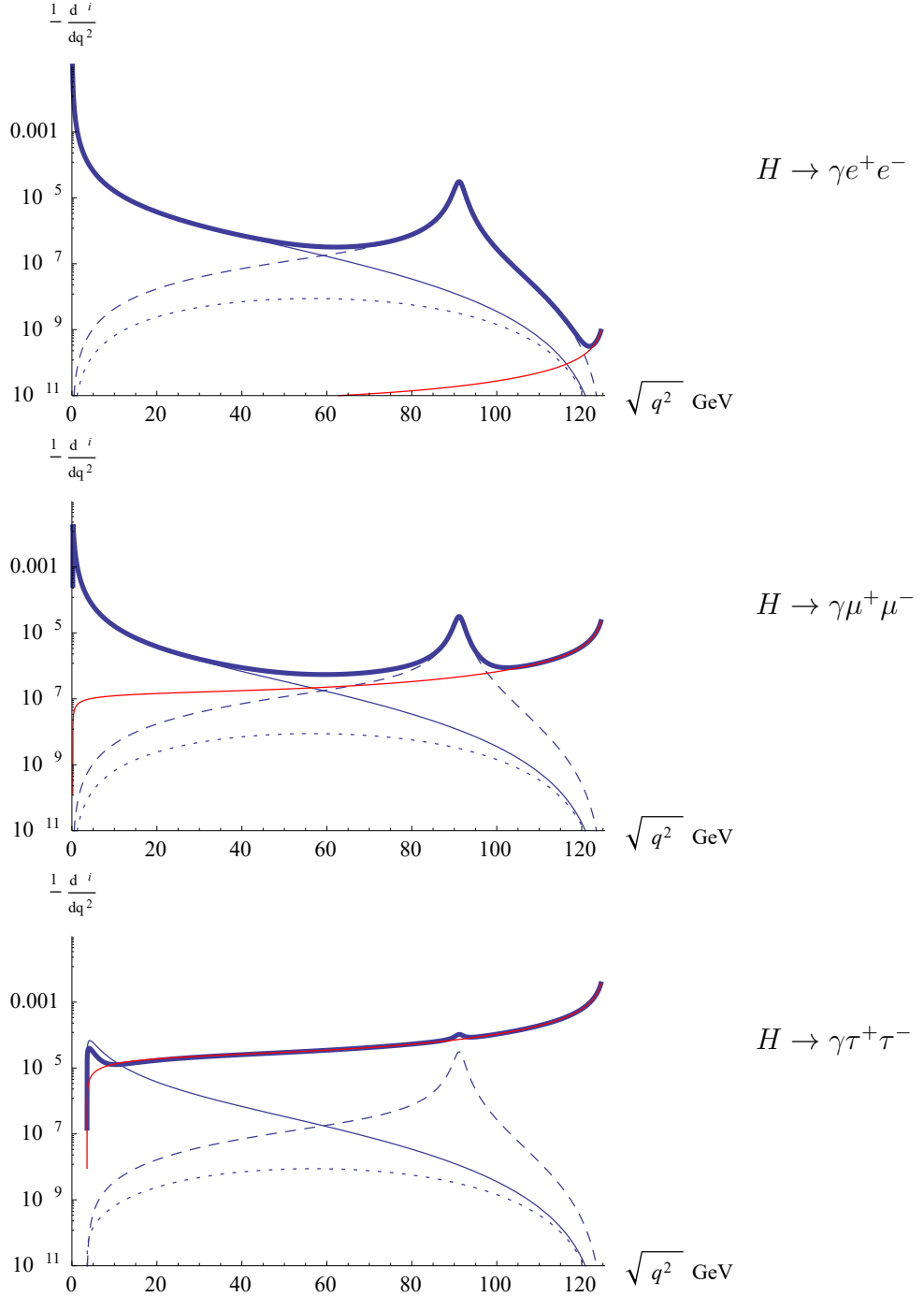
Fig. B.38: The invariant mass distributions in \sqrt{q^2} = M_{\ell^+\ell^-} of the Dalitz decays H \rightarrow \gamma + e^+e^-/\mu^+\mu^-/\tau^+\tau^- normalized to \Gamma(H \rightarrow \gamma\gamma) with a cut E_\gamma > 1 GeV on the photon energy. The red lines show the contribution of the tree diagrams, the thin solid lines denote the contribution of the photon conversion H \rightarrow \gamma\gamma^* \rightarrow \gamma\ell^+\ell^- , and the dashed line the contribution from the Z^* exchange diagrams, while the thick lines present the total contributions. The dotted lines denote the contribution from the box diagrams (in 't Hooft–Feynman gauge). From Ref. [89].
