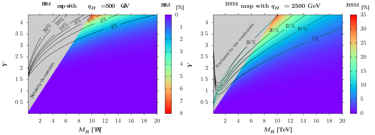
Fig. E.5: Contour maps of the heavy neutral lepton correction \Delta^{\text{BSM}} to the triple Higgs coupling \lambda_{HHH} (in %) as a function of the heavy neutral lepton parameters M_R (in TeV) and |Y_\nu| at a fixed off-shell Higgs momentum q_{H^*} = 500 GeV (left) and q_{H^*} = 2500 GeV (right). The details of the spectrum are given in Ref. [32]. The grey area is excluded by the constraints on the model and the green lines on the right figure are contour lines that correspond to our approximate formula while the black lines correspond to the full calculation.
