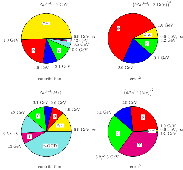
Fig. B.9: Contributions and square errors from e^+e^- data ranges and form pQCD to \Delta \alpha_{\text{had}}^{(5)}(-M_0^2) vs. \Delta \alpha_{\text{had}}^{(5)}(M_Z^2) .
