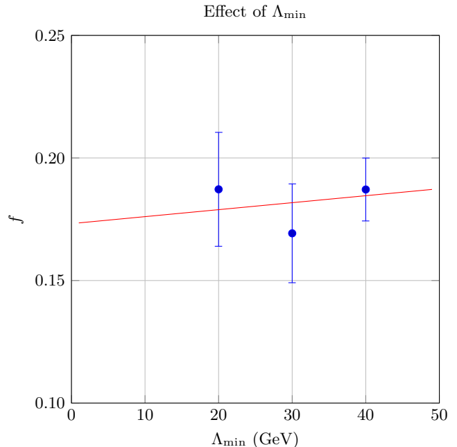
FIG. 4. Gap fraction f in the range 300 \text{ GeV} < \bar{p}_T < 400 GeV and 4 < y_{12} < 5 as a function of \Lambda_{\text{min}} . The calculation uses N_{\Delta}^{\text{thr}} = 1 at the start of the shower, then N_{\text{Re}} = 2 , N_{i\pi} = 2 for the shower in the range \mu_s > \Lambda > \Lambda_{\text{min}} , then N_{\text{Re}} = N_{i\pi} = 0 in the range \Lambda_{\text{min}} > \Lambda > 1 GeV. The maximum color suppression index is I_{\text{max}} = 4 . The curve is a linear fit to the numerical results.
