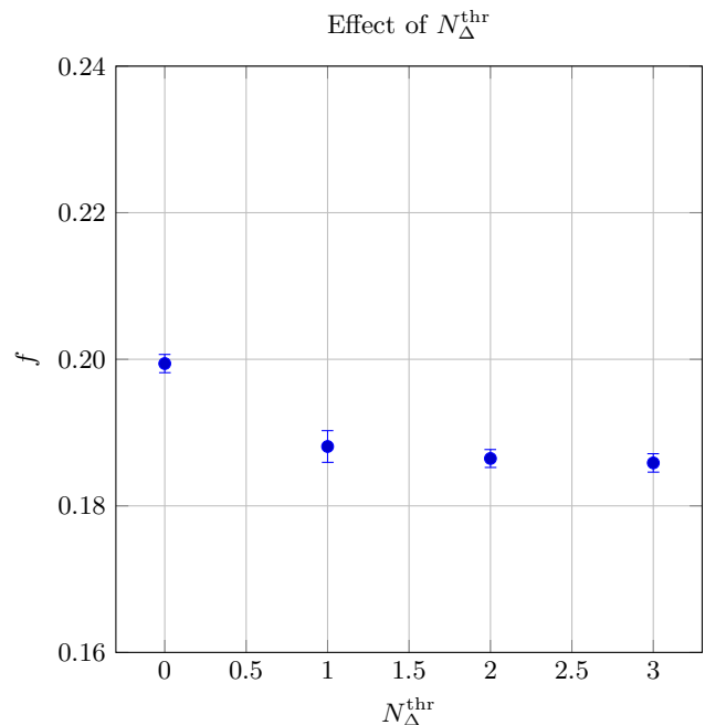
FIG. 3. Gap fraction f as in Fig. 1 calculated with different values of N_{\Delta}^{\text{thr}} with N_{\text{Re}} = N_{i\pi} = 0 .
