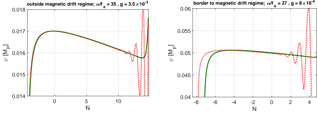
Figure 7: Analytic background field with the c_2 solution (solid green) compared to its numerical solution (dashed red). The matching condition (43) is sufficient for large gauge group couplings and/or small effective interaction couplings.
