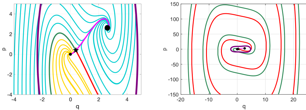
Figure 1: Flow of the vector field of the autonomous gauge field background differential equation for \xi = 3 . The zeros of the field are given by \mathbf{z}_0 = 0 (small dot), \mathbf{z}_1 = c_1(\xi, \xi) (star) and \mathbf{z}_2 = c_2(\xi, \xi) (big dot). Yellow and blue flow lines correspond to an evolution into the \mathbf{z}_1 and \mathbf{z}_2 zero respectively. The magenta line indicates a possible tunneling between the different zeros. Further, we especially highlight with red and green the one parameter family of flow lines evolving into the unstable \mathbf{z}_1 zero. These two lines mark the boundary for which a randomly located point evolves into either one of the \mathbf{z}_{0,2} zeros. For reference, the purple line denotes the transition regime – after transforming into the new coordinates – between an oscillatory and constant solution. This transition happens within \sim 2 e-folds once this line is reached.
