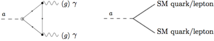
Figure 2. Model-dependent axion couplings to photons and SM quarks and leptons.
