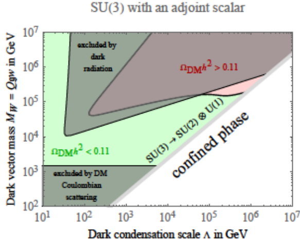
Figure 1: We consider a typical model with DM charged under dark photons: one Higgs phase of gauged SU(3) with a scalar in the adjoint. The cosmological DM abundance is reproduced thermally around the boundary between the green (DM under-density) and red (DM over-density) regions. The regions in grey are excluded by the resulting dark radiation and Coulombian scatterings among DM particles. The confined phase of this model (in white) features no DM candidate.
