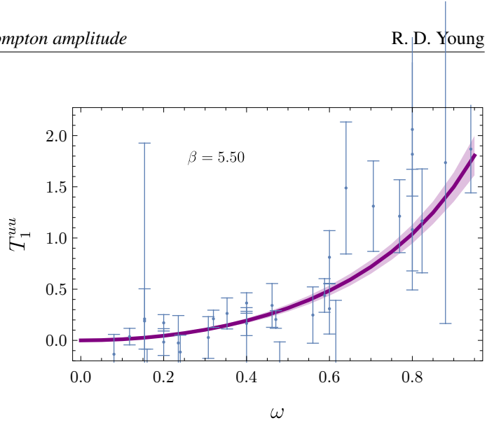
Figure 1: Compton amplitude extracted as a function of \omega = 2p \cdot q/Q^2 for five different Q^2 values ( 2.7 \dots 6.9 \text{ GeV}^2 ). The curve shows a combined fit, as described in the text, including the leading-order perturbative QCD evolution (at a factorisation scale \mu^2 = 4 \text{ GeV}^2 ).
