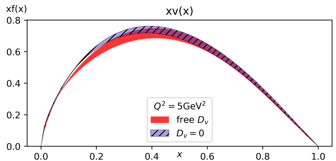
FIG. 2. The valence distribution when using minimal parameterisation ( D_v = 0 ) and the extended parameterisation with free D_v . The shown uncertainty bands do not include scale variations.
