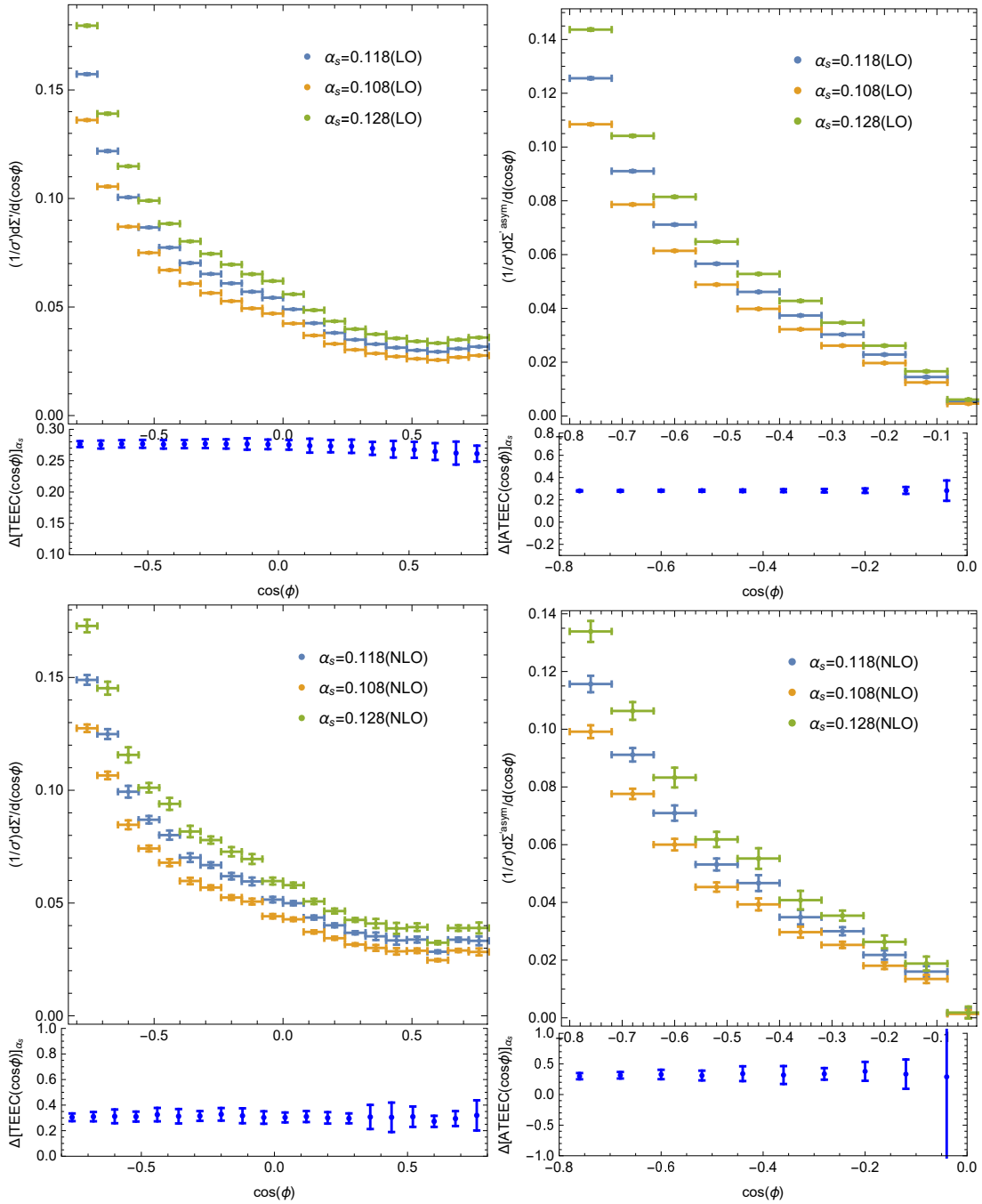
FIG. 8: Dependence of the differential distribution 1/\sigma' d\Sigma'/d(\cos\phi) (left) and its asymmetry 1/\sigma' d\Sigma'^{asym}/d(\cos\phi) (right) on the QCD coupling constant \alpha_s(M_Z) for three indicated values of \alpha_s(M_Z) = 0.108, 0.118, 0.128 using the PDFs of MMHT14 in the low- Q^2 range at HERA setting the scales \mu_F = \mu_R = \mu_0 .
