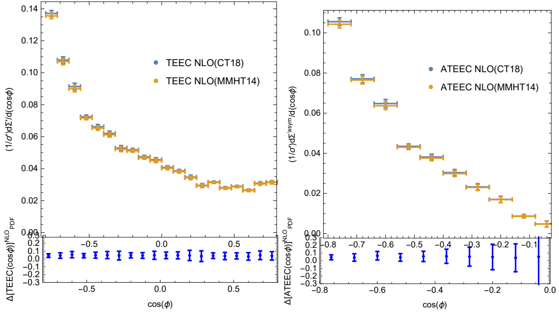
FIG. 3: Differential distribution 1/\sigma' d\Sigma'/d(\cos\phi) and its asymmetry 1/\sigma' d\Sigma'^{asym}/d(\cos\phi) as in Fig. 2, but for the high- Q^2 range 150 \text{ GeV}^2 < Q^2 < 1000 \text{ GeV}^2 at HERA.
