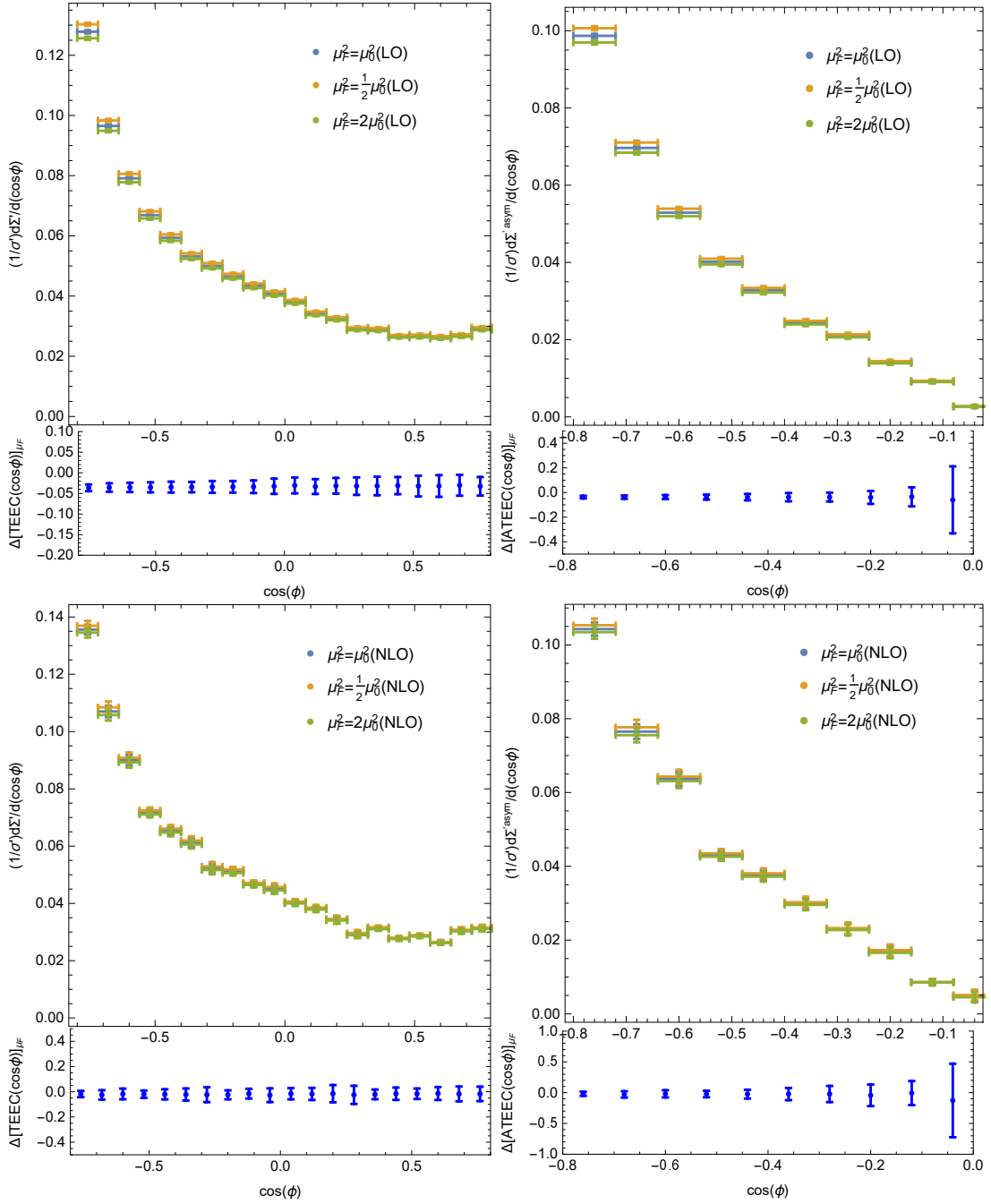
FIG. 5: Factorization scale dependence of the differential distribution 1/\sigma' d\Sigma'/d(\cos\phi) and its asymmetry 1/\sigma' d\Sigma'^{asym}/d(\cos\phi) in the leading order (upper frames) and the next to leading order (lower frames) as in Fig. 4, but for the high- Q^2 range 150 \text{ GeV}^2 < Q^2 < 1000 \text{ GeV}^2 at HERA.
