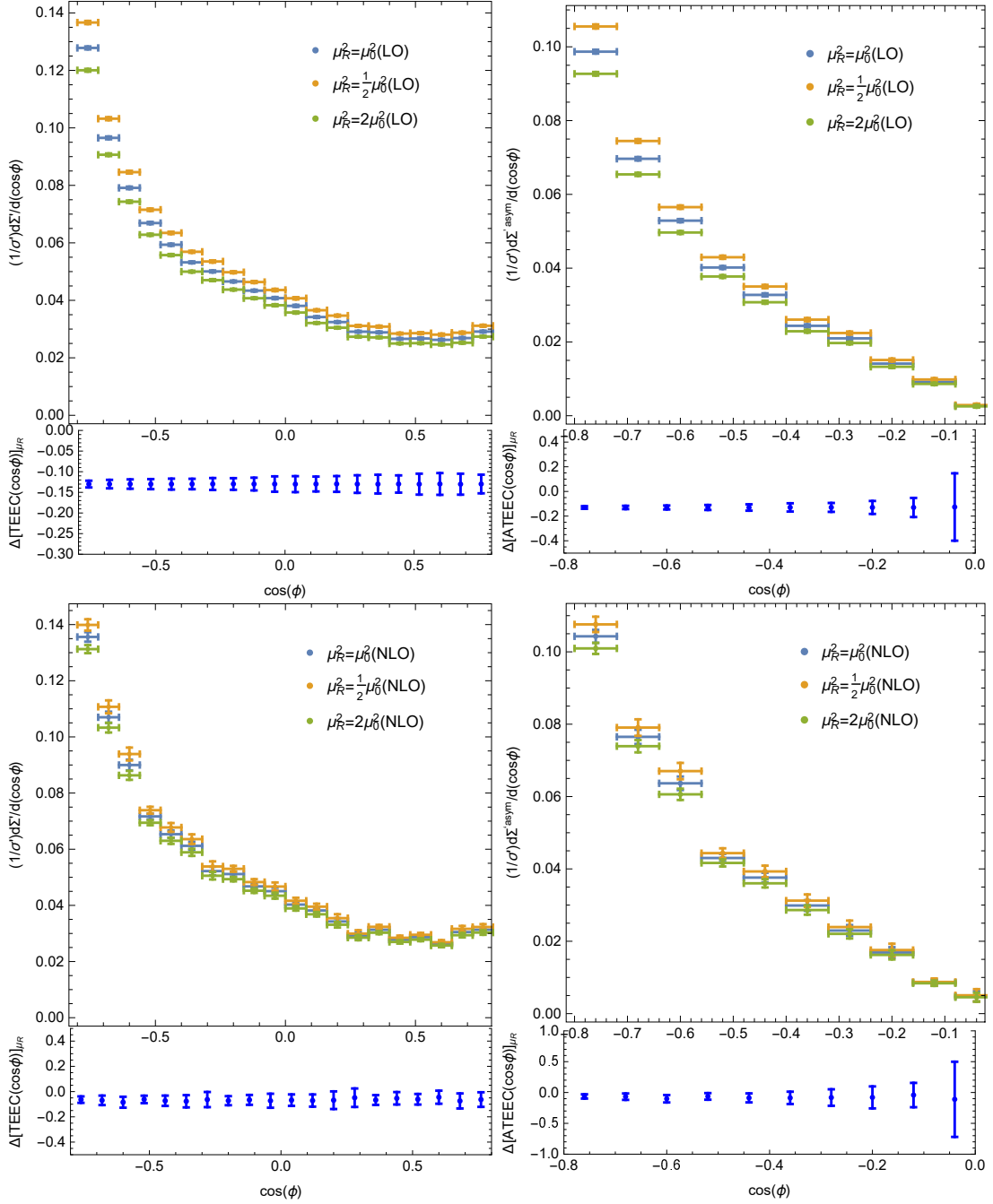
FIG. 7: Renormalization scale dependence of the differential distribution 1/\sigma'd\Sigma'/d(\cos\phi) and its asymmetry 1/\sigma'd\Sigma'^{asym}/d(\cos\phi) in the leading order (upper frames) and the next to leading order (lower frames) as in Fig. 6, but for the high- Q^2 range: 150 \text{ GeV}^2 < Q^2 < 1000 \text{ GeV}^2 at HERA.
