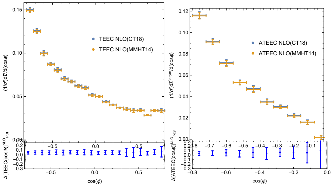
FIG. 2: Differential distribution 1/\sigma' d\Sigma'/d(\cos \phi) and its asymmetry 1/\sigma' d\Sigma'^{asym}/d(\cos \phi) , calculated in Next-to-Leading order for the low- Q^2 range 5.5 \text{ GeV}^2 < Q^2 < 80 \text{ GeV}^2 for the ep center-of-mass energy \sqrt{s} = 314 GeV at HERA. The two input PDFs are indicated on the upper frames. The lower frames show \Delta[\text{TEEC}(\cos \phi)]_{\text{PDF}}^{\text{NLO}} and \Delta[\text{ATEEC}(\cos \phi)]_{\text{PDF}}^{\text{NLO}} , defined in Eq. (15).
