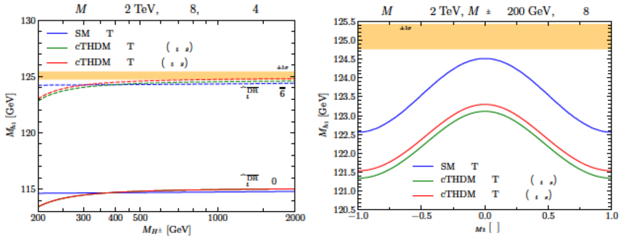
Figure 1: Left: M_{h_1} in dependence of M_{H^\pm} for \hat{X}_t^{\text{DR}} = 0 (solid) and \hat{X}_t^{\text{DR}} = \sqrt{6} (dashed). The result obtained using a SM-EFT calculation (blue) are compared to results using cTHDM-EFT calculations not including the \mathcal{O}(\alpha_t \alpha_s) threshold corrections (green) and including the \mathcal{O}(\alpha_t \alpha_s) threshold corrections (red). The yellow band displays the Higgs mass as measured by ATLAS and CMS within one standard deviation of experimental accuracy. 6 Right: Same as left plot but M_{h_1} is shown in dependence of \phi_{M_3} for \hat{X}_t^{\text{DR}} = \sqrt{6} .
