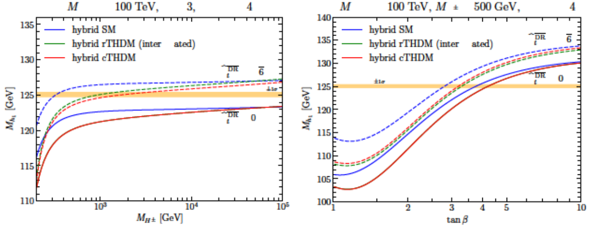
Figure 2: Left: M_{h_1} in dependence of M_{H^\pm} for \hat{X}_t^{\overline{\text{DR}}} = 0 (solid) and \hat{X}_t^{\overline{\text{DR}}} = \sqrt{6} (dashed). The result obtained using the SM hybrid calculation (blue) are compared to results using the interpolated hybrid THDM calculation (green) and the hybrid cTHDM calculation (red). The yellow band displays the Higgs mass as measured by ATLAS and CMS within one standard deviation of experimental accuracy. Right: Same as left plot but M_{h_1} is shown in dependence of t_\beta .
