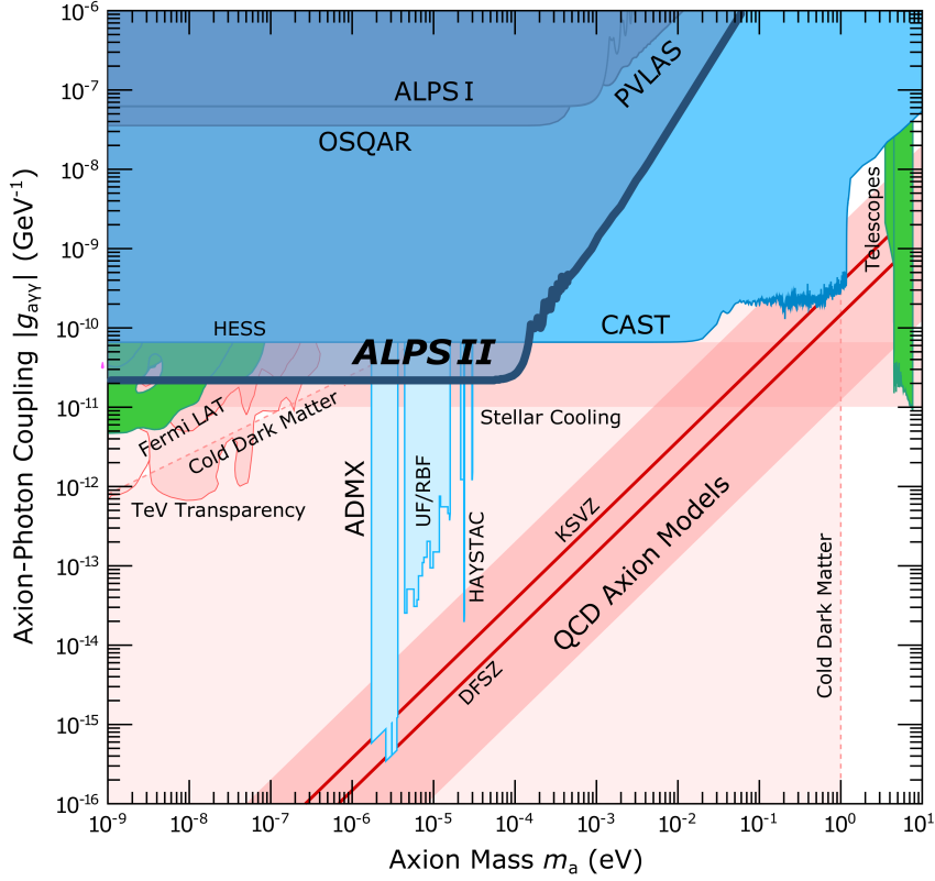
Figure 1: ALPS II target sensitivity, shown in the transparent blue region, along with current exclusion limits for axion-like-particles given in blue for the helioscopes [6], dark blue for the LSW experiments [7, 8, 9], light blue for dark matter haloscopes [10, 11, 12, 13, 14, 15, 16, 17, 18], and green for the astronomical observations [19, 20, 21]. Regions of the parameter space which offer hints of their existence are shown in red [22, 23, 24, 25, 26, 27, 28, 29, 30, 31]. Please note that several exclusion limits rely on mostly untested assumptions such as axions or axion-like particles making up 100% of the dark matter in the milky way, structures of galactic and intergalactic magnetic fields, or axion and axion-like particles production in dense stellar plasmas.
