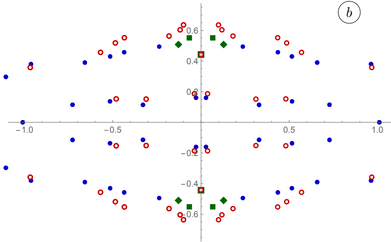
Figure 15: The open circles depict the distribution of b(N) = \frac{n}{4\pi} \log(B) in the complex plane, where B is the eigenvalue of the quasi-shift operator, for the 42 = 34 + 8 states with L = 3 , \bar{L} = 0 and w = 0 as indicated in tab.1. The filled circles, squares and diamonds correspond to the solutions b_* of eq. (18.14). For the circles \lim_{N \rightarrow \infty} \Im m(b_*(N)) = 0 , while for the squares, b_*(N) \rightarrow \pm \frac{9i}{20} as N \rightarrow \infty . The filled diamonds form two pairs which have the same value of \Im m(b_*(N)) and opposite real part. At large but finite N the diamonds from the upper pair collide at the imaginary axis at which point for one of the diamonds b_*(N) \rightarrow +\frac{9i}{20} while for the other one b_*(N) \rightarrow 0 . The N dependence of b_*(N) for the lower pair of diamonds is obtained from that of the upper pair via complex conjugation.
