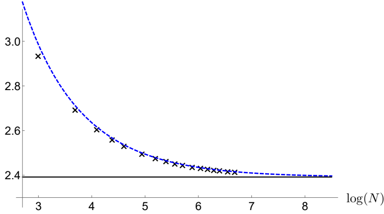
Figure 11: Numerical data for an RG trajectory \Psi_N with L = \bar{L} = S^z = \mathbf{w} = 0 and labeled by pure imaginary s = i(-p - \frac{1}{2}) = \frac{i}{4} is used to illustrate the asymptotic formula (11.29). The parameters have been set to be n = 3 , \mathbf{k} = -\frac{3}{10} . Depicted by the crosses is the r.h.s. of (11.29), calculated from the solution of the Bethe ansatz equations corresponding to \Psi_N and then divided by the leading and subleading large N asymptotic that is given in the second line of that relation, i.e., (\frac{N}{2N_0})^{-\frac{4np}{n+2}-8|s|} (\frac{4n}{n+2})^{-N} \prod (\zeta_m^{-2} + q^2)(\zeta_m^{-2} + q^{-2}) . The predicted limiting value of the last quantity, 2^{-\frac{1}{3}} 5^{-\frac{4}{5}} \pi^3 / \Gamma^4(\frac{7}{10}) = 2.392\dots , is represented by the solid line. The dashed line corresponds to (\frac{N}{2N_0})^{-8|b|} (R_{p,b}^{(0)})^2 , where b = b(N) was obtained by solving eq. (9.11) with the correction terms ignored, \sigma = +1 and e^{\frac{1}{2}\delta} is given by (9.3).
