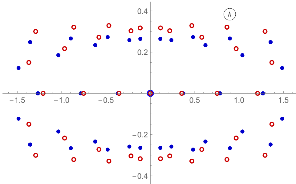
Figure 22: The value of b(N) for the 40 = 40 + 0 states (open circles) having w = 0 and (L, \bar{L}) = (0, 2) .
