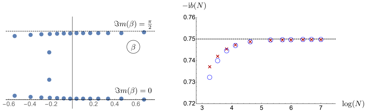
Figure 4: The left panel depicts the pattern of Bethe roots \beta_j = -\frac{1}{2} \log(\zeta_j) for a low energy state \Psi_N for which \lim_{N \rightarrow \infty} b(N) = \frac{im}{4} , i.e., belongs to the boundary of the strip (8.7). The parameters are n = 3 , \mathbf{k} = \frac{1}{10} , while the state belongs to the sector S^z = \mathbf{w} = 0 and L = \bar{L} = 1 . On the right panel -ib(N) (which turns out to be real) is plotted as a function of \log(N) for this RG trajectory. The red crosses correspond to b(N) calculated from the eigenvalue of the quasi-shift operator using eq. (8.6), while the dashed line shows the limiting value \lim_{N \rightarrow \infty} b(N) = 0.75i . To illustrate that the energy for this state obeys eq. (8.2a), we depict via the open circles the values of b(N) computed from the numerical data for the energy by inverting (8.2a) for b(N) with the correction terms ignored.
