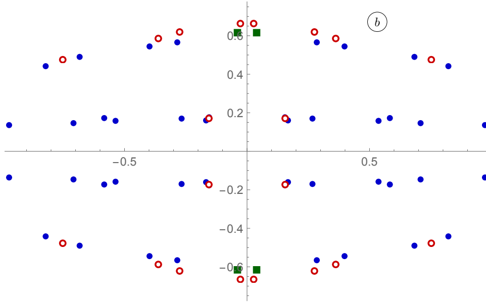
Figure 23: The value of b(N) for the 20 = 16 + 4 states (open circles) having w = 0 and (L, \bar{L}) = (2, 1) .
