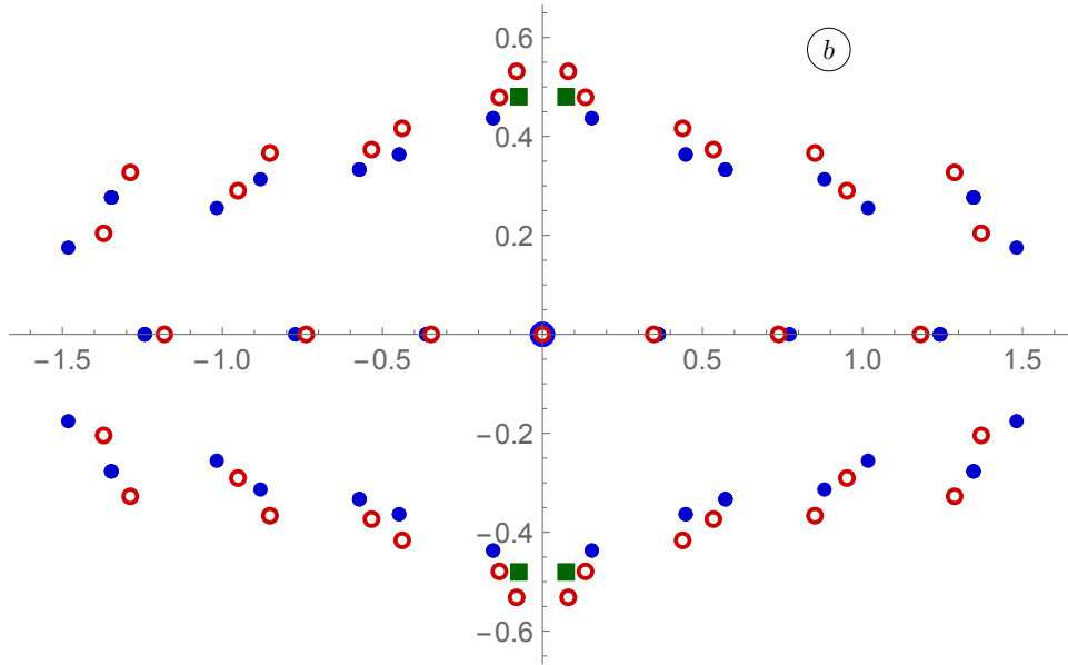
Figure 21: The value of b(N) for the 40 = 36 + 4 states (open circles) having w = 0 and (L, \bar{L}) = (2, 0) .
