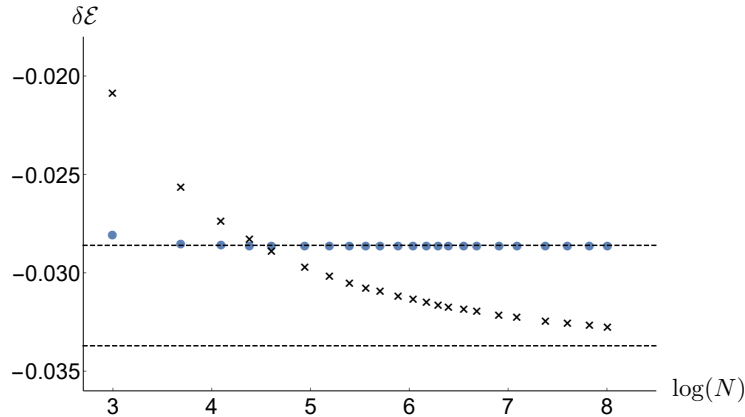
Figure 7: The value of \delta\mathcal{E} = \frac{N}{4\pi v_F} (\mathcal{E} - e_\infty N) is plotted as a function of \log(N) for two RG trajectories in the case n = 3 and \mathbf{k} = 0.235 > \frac{1}{n+2} . The blue dots depict \delta\mathcal{E} for the trajectory having \mathbf{L} = \bar{\mathbf{L}} = S^z = \mathbf{w} = 0 and with s = 0 . If \log(N) \gtrsim 4.5 the corresponding Bethe state is the ground state of the Hamiltonian \mathbb{H} . For the second RG trajectory (crosses) the RG invariants \mathbf{L}, \bar{\mathbf{L}}, S^z, \mathbf{w} are also zero but s = \frac{i}{2}((n+2)\mathbf{k} - 1) = \frac{7i}{80} is a pure imaginary number. The dashed lines denote the limiting values \delta\mathcal{E} = -0.0286\dots for the RG trajectory with zero s and \delta\mathcal{E} = -0.0337\dots for the other one.
