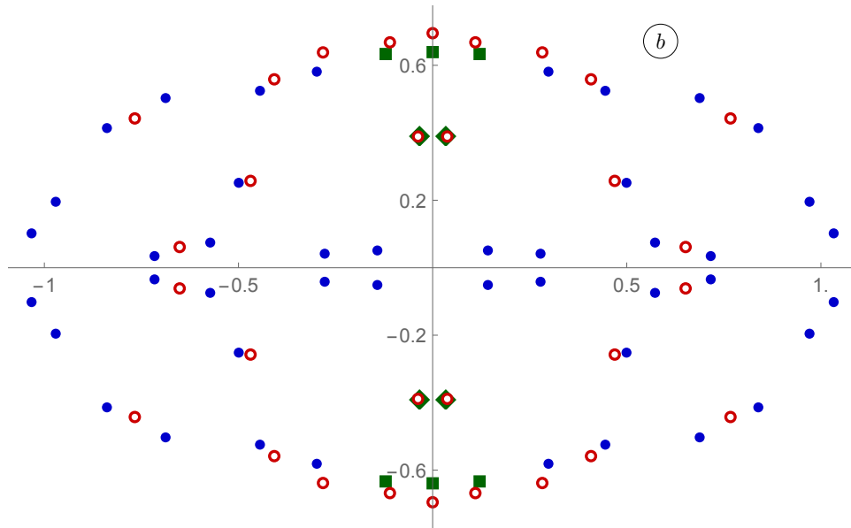
Figure 24: The value of b(N) for the 30 = 22 + 8 states (open circles) having w = 0 and (L, \bar{L}) = (1, 2) . As with the filled circles and squares, the filled diamonds correspond to solutions b_*(N) of eq. (18.14). These form two pairs which have the same value of \Im m(b_*(N)) and opposite real part. At large but finite N the diamonds from the upper pair collide at the imaginary axis at which point for one of the diamonds b_*(N) \rightarrow +\frac{9i}{20} while for the other one b_*(N) \rightarrow 0 . The N dependence of b_*(N) for the lower pair of diamonds is obtained from that of the upper pair via complex conjugation.
