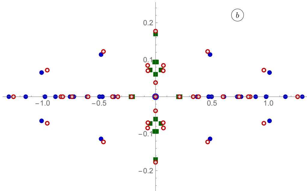
Figure 26: The value of b(N) for the 37 = 21 + 16 states (open circles) with w = 1 and any values of L and \bar{L} .
