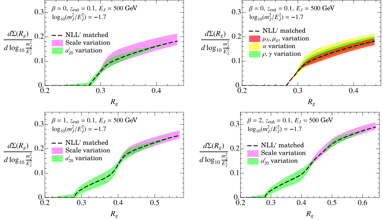
Figure 7: Theoretical uncertainty on the cross section cumulant in R_g , for \log_{10}(m_J^2/E_J^2) = -1.7 and different values of \beta . The central curve (black dashed) is obtained with the matching prescription described in the text, while the colored bands probe respectively scale variation (magenta), and variation of the fixed order two-loop constants a_{20}^{S_c} and a_{20}^C , collectively denoted as a_{20}^i variation (green). In the top right plot, the envelope of scale variations for \beta = 0 is broken down into various components: overall variation by a common factor (red), variation by a trumpet factor preserving canonical relations (yellow), breaking of canonical relations (green).
