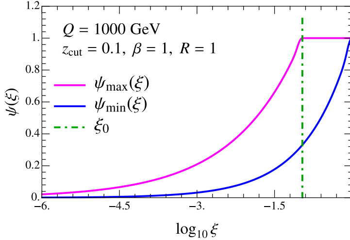
Figure 3: The range of values of allowed \psi values as a function of \xi are shown by the region between the solid (magenta and blue) lines. The dot-dashed (green) line indicates where the transition to the ungroomed regime takes place. The maximum value of \psi corresponds to R_g = \theta_g^*(\xi) , or \psi = R in the ungroomed regime.
