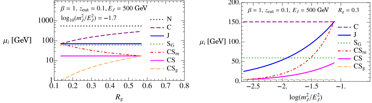
Figure 4: Profile scales \mu_i as a function of the groomed radius at fixed jet mass (top left) and as a function of the mass at fixed radius (top right), for \beta = 1 . For more clarity the former plot uses a logarithmic scale, while we omit the hard scale \mu_N in the latter. At small groomed radii (large jet masses) \mu_{CS_m} and \mu_J merge into \mu_C , while at large radii (small masses) \mu_{CS_m} and \mu_{CS_g} become a single soft-collinear scale \mu_{CS} , consistent with the mode picture.
