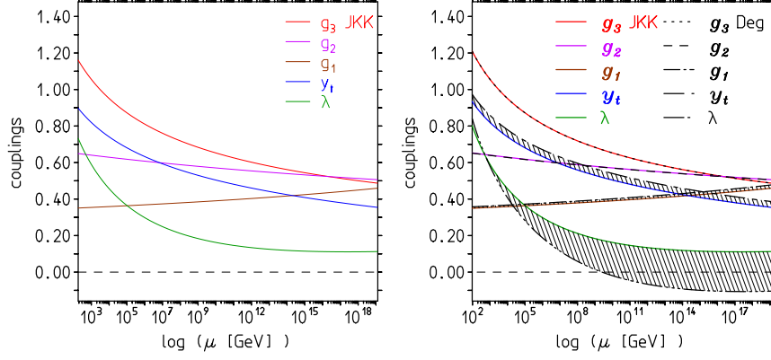
Fig. 1. Running SM parameters from the Z mass scale up to M_{P1} . Left: on-shell vs \overline{\text{MS}} parameter matching based on F.J., Kalmykov, Kniehl [57] (JKK). Right: the same in comparison with Shaposnikov et al. [52], Degrassi et al. [53] (Deg) matching. Using JKK input parameters the vacuum remains stable, with Deg input vacuum stability breaks down at about 10^9 GeV and enters in a metastable state of the effective potential [58] (i.e. including radiative corrections). Small cause, great impact, just by changing a little the input parameters, most sensitive on y_t , we get a completely different behavior of the Higgs system towards the Planck era. The shaded space illustrates the parameter-matching controversy, which concerns y_t at M_Z . Plots adapted from [44].
