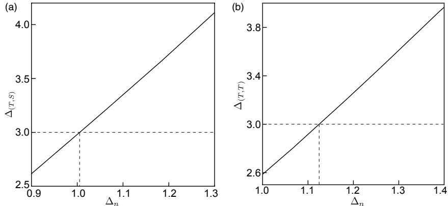
FIG. 3. (a-b) Numerical bounds of \Delta_{(T,S)} and \Delta_{(T,T)} for the N = 7 Stiefel liquid. The allowed region is below the black curve. Here we take \Lambda = 27 .
