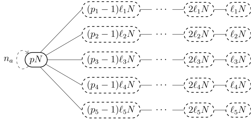
Figure 5.2: The comet-shaped quiver that depicts the Lagrangian \mathcal{N} = 1 quiver we consider. When we write a number M inside a gauge node we remind the reader that this corresponds to an SU(M) gauge group. A dashed-bordered circular node denotes an \mathcal{N} = 2 vector multiplet, a solid-bordered circular node denotes an \mathcal{N} = 1 vector multiplet, and an undirected link between two nodes denotes an \mathcal{N} = 2 bifundamental hypermultiplet. The dashed self-link corresponds to n_a adjoint chiral multiplets.
