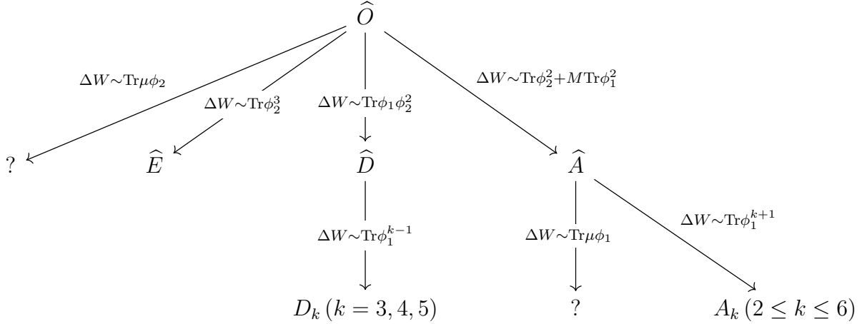
Figure 5.1: Deforming the theories with one \mathcal{D}_p(G) and two adjoint chiral multiplets (\phi_1, \phi_2) , that we refer to as \widehat{O} , via ADE-type superpotential. When the \widehat{O} is deformed by \text{Tr} \phi_2^2 , the \text{Tr} \phi_1^2 becomes free during the RG-flow and must be flipped by the flip-operator M . The question marks represent non-ADE deformations.
