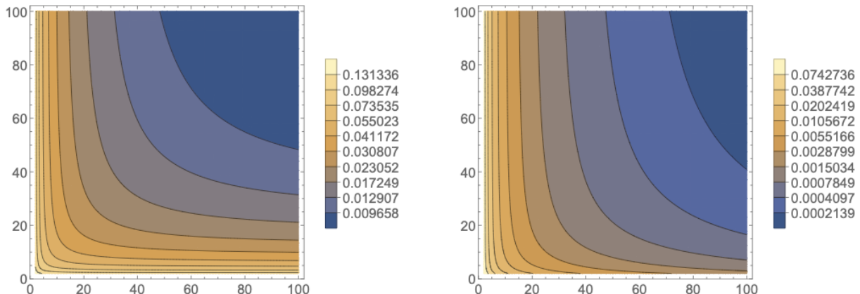
(a) Contour plot of -\epsilon_1 on the (p_3, p_4) -plane. (b) Contour plot of -\epsilon_3 on the (p_3, p_4) -plane.
