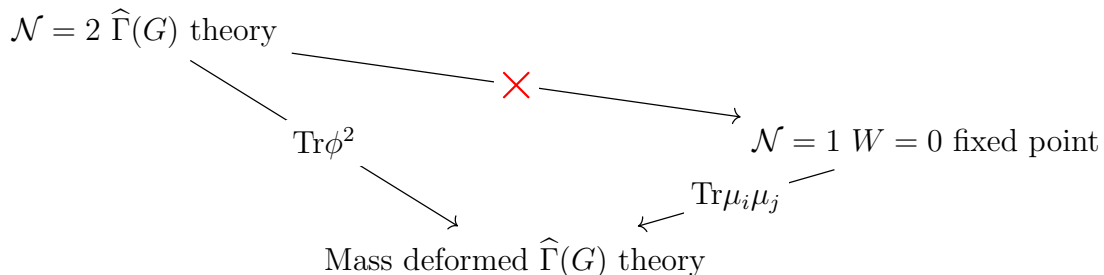
Figure 1.1: RG flows triggered by the mass deformation of the \mathcal{N} = 2 theory vs gauging an \mathcal{N} = 1 vector multiplet. The red cross is to emphasize that there is no direct renormalization group flow between the \mathcal{N} = 2 gauging and the \mathcal{N} = 1 gauging.
