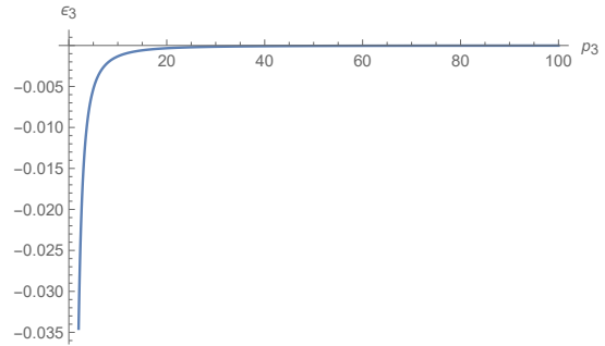
(b) Plot of \epsilon_3 against p_3 for the gauging (2, 2, p_3) with one adjoint chiral.
