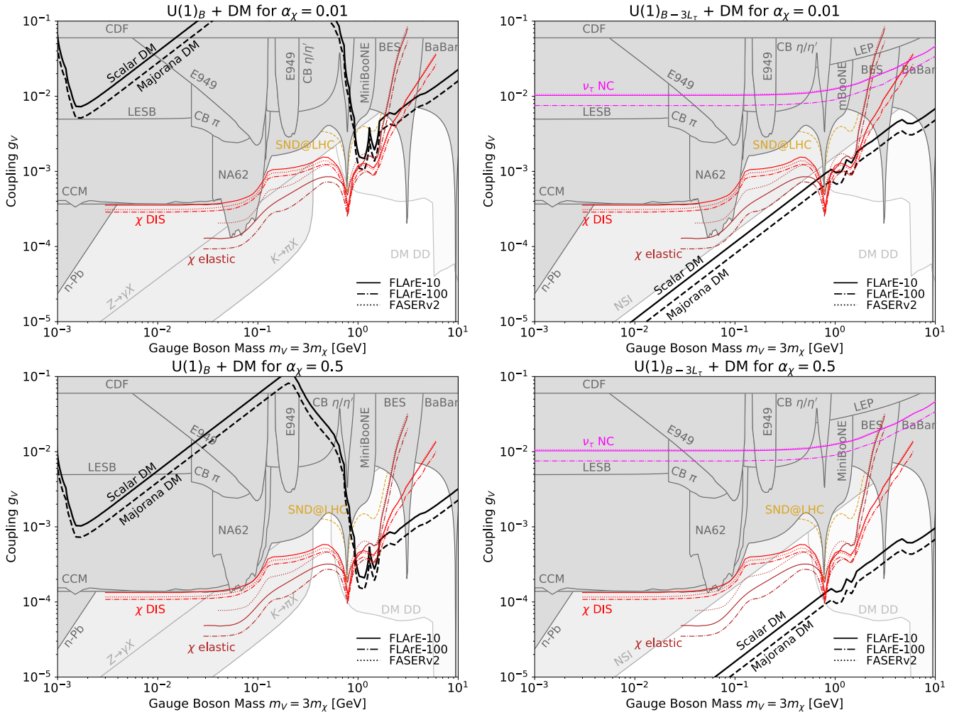
FIG. 2. The (m_V, g_V) parameter space of hydrophilic DM models with U(1)_B (left) and U(1)_{B-3\tau} (right) gauge boson mediators coupling to complex scalar DM, for dark matter coupling \alpha_\chi = 0.01 (top) and 0.5 (bottom), and m_V = 3m_\chi . The black contours are the thermal relic targets for complex scalar and Majorana DM; DM is thermally overproduced below these contours. The light (dark) red lines correspond to 90% CL exclusion bounds from DM DIS (elastic) scatterings off nuclei for FLArE-10, FLArE-100, and FASERV2, as indicated. The dotted brown contours are the sensitivity contours for SND@LHC [99]. In the right panels, the light purple contours are the projected sensitivity contours from probing the V -induced BSM NC interactions of tau neutrinos. In both panels, the dark gray shaded regions are excluded by current bounds. The light gray shaded regions in the left (right) panels correspond to the anomaly-induced K and Z decays (NSI bounds). The very light gray shaded regions are constraints from DM DD; these do not apply to Majorana and inelastic scalar DM (see Sec. IID).
