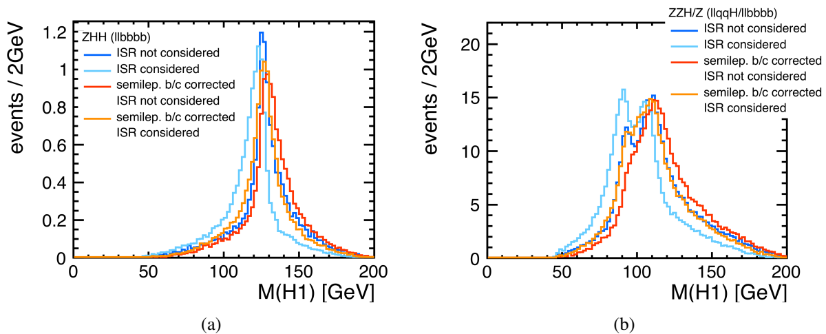
Figure 1: Higgs mass reconstruction in the presence of ISR photon and semi-leptonic decays: (a) The signal peak gets sharper by considering ISR photon and correction of semi-leptonic decays. (b) The background peak is pulled towards the signal.
