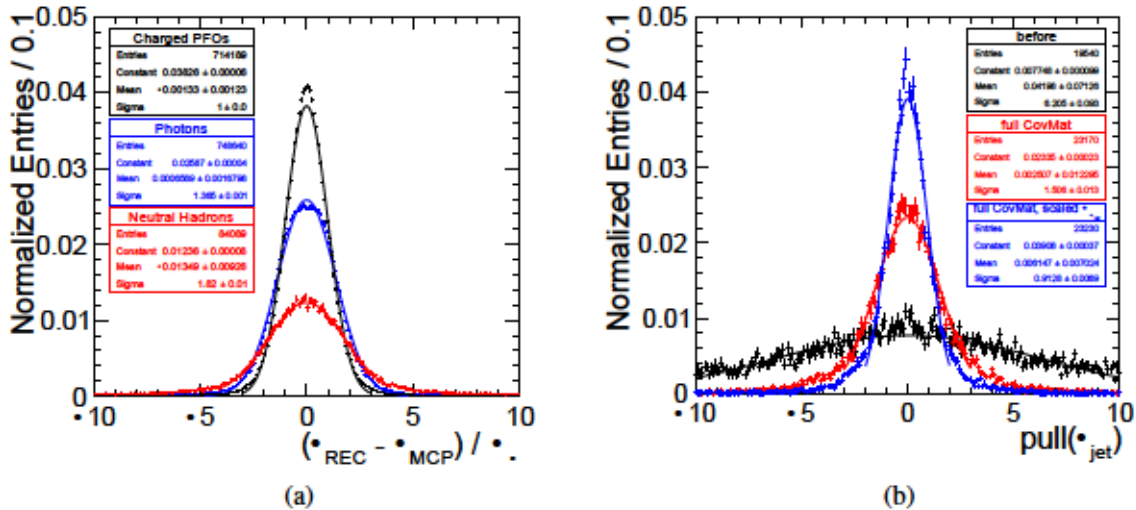
Figure 2: (a) Normalized residual of \theta_{\text{PFO}} for charged particles (black), photons (blue) and neutral hadrons (red) (b) Pull of the jet angle ( \theta_{\text{jet}} ) from the kinematic fit when the jet angular uncertainty ( \sigma_{\theta_{\text{jet}}} ) receives contribution from only charged particles (black), all particles (red) and when \sigma_{\theta_{\text{PFO}}} is scaled up for photons and neutral hadrons by a factor of 1.3 and 1.8, respectively, motivated from fig. 2(a)
