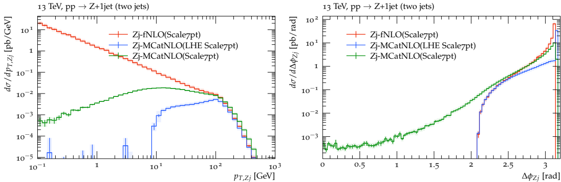
Figure 2: Transverse momentum spectrum of the Z+jet-system p_{T,Zj} (left) and \Delta\phi_{Zj} distribution (right). Shown are predictions from fixed NLO (fNLO), the (unphysical) distribution at LHE-level and the full simulation (after inclusion of PB-TMDs and TMD showers, MCatNLO+CAS3).
