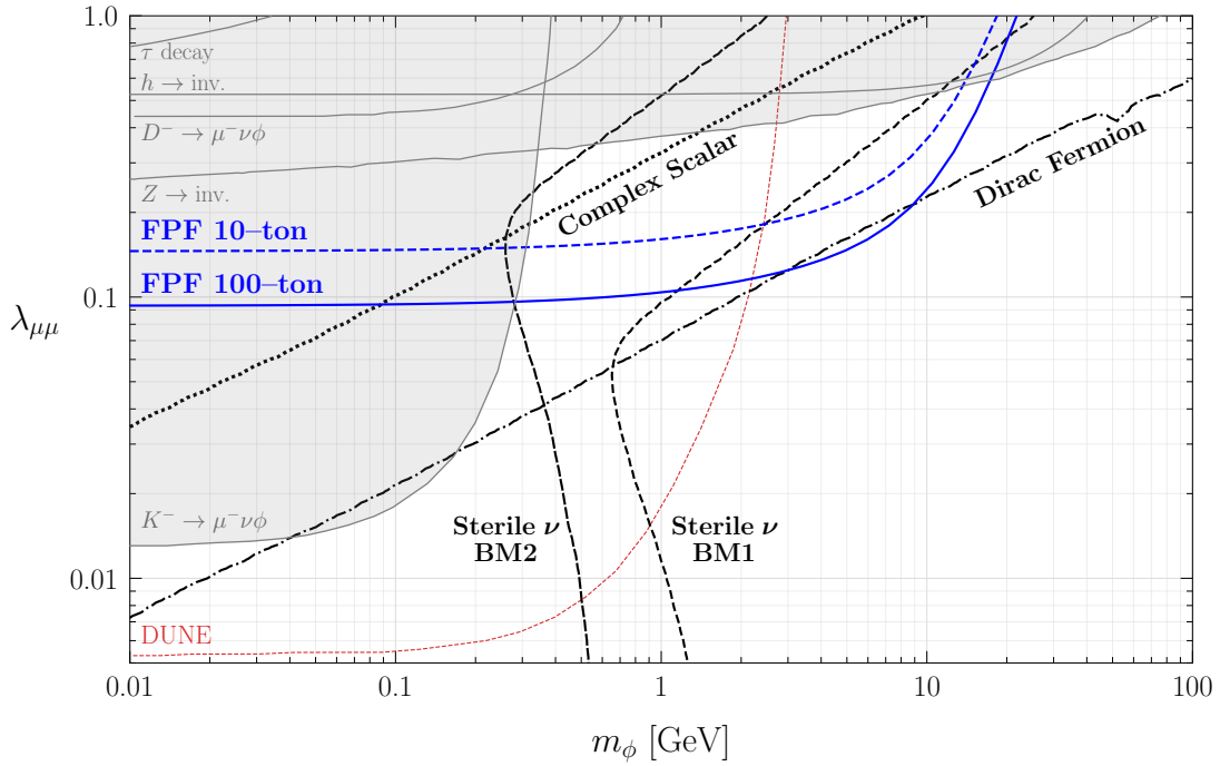
Figure 14. Parameter space of neutrinophilic scalar spanned by its coupling to muon neutrinos \lambda_{\mu\mu} and its mass m_\phi . The region excluded by previous measurements is shown in gray-shaded, while the projected reach of DUNE and the FPF are shown as red and blue colored lines, respectively. Various DM target lines are shown in black. See text and Refs. [9, 215] for details.
