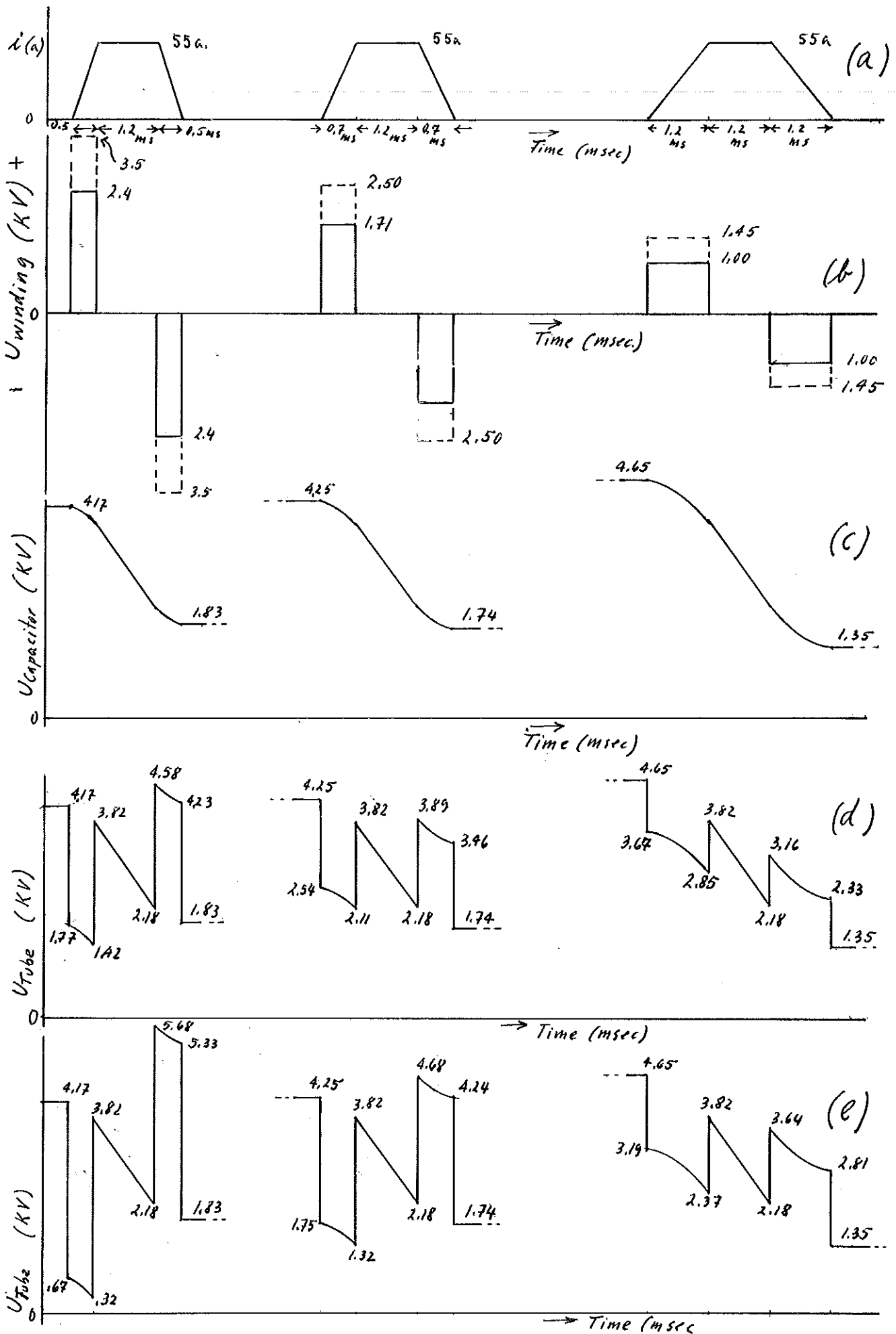
Fig 8.: E-Pulsar waveshapes a) Current b) Backleg winding voltage, dotted line; Airgap winding voltage, solid line c) Capacitor C voltage d) Tube voltage for airgap winding e) Tube voltage for backleg winding.
