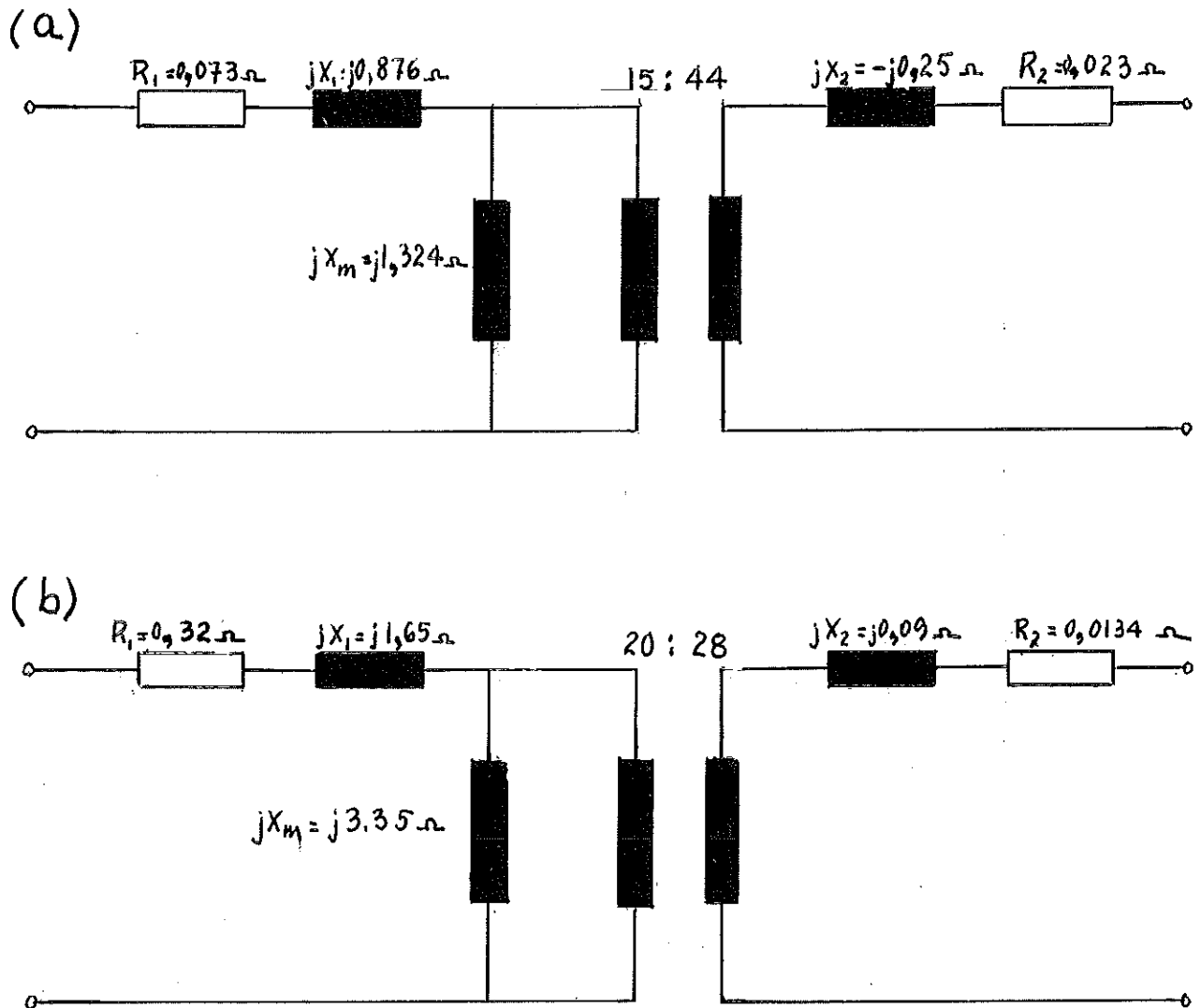
Figure 6.: a) D magnet equivalent circuit (backleg winding and main winding) b) F magnet equivalent circuit (backleg winding and main winding)
