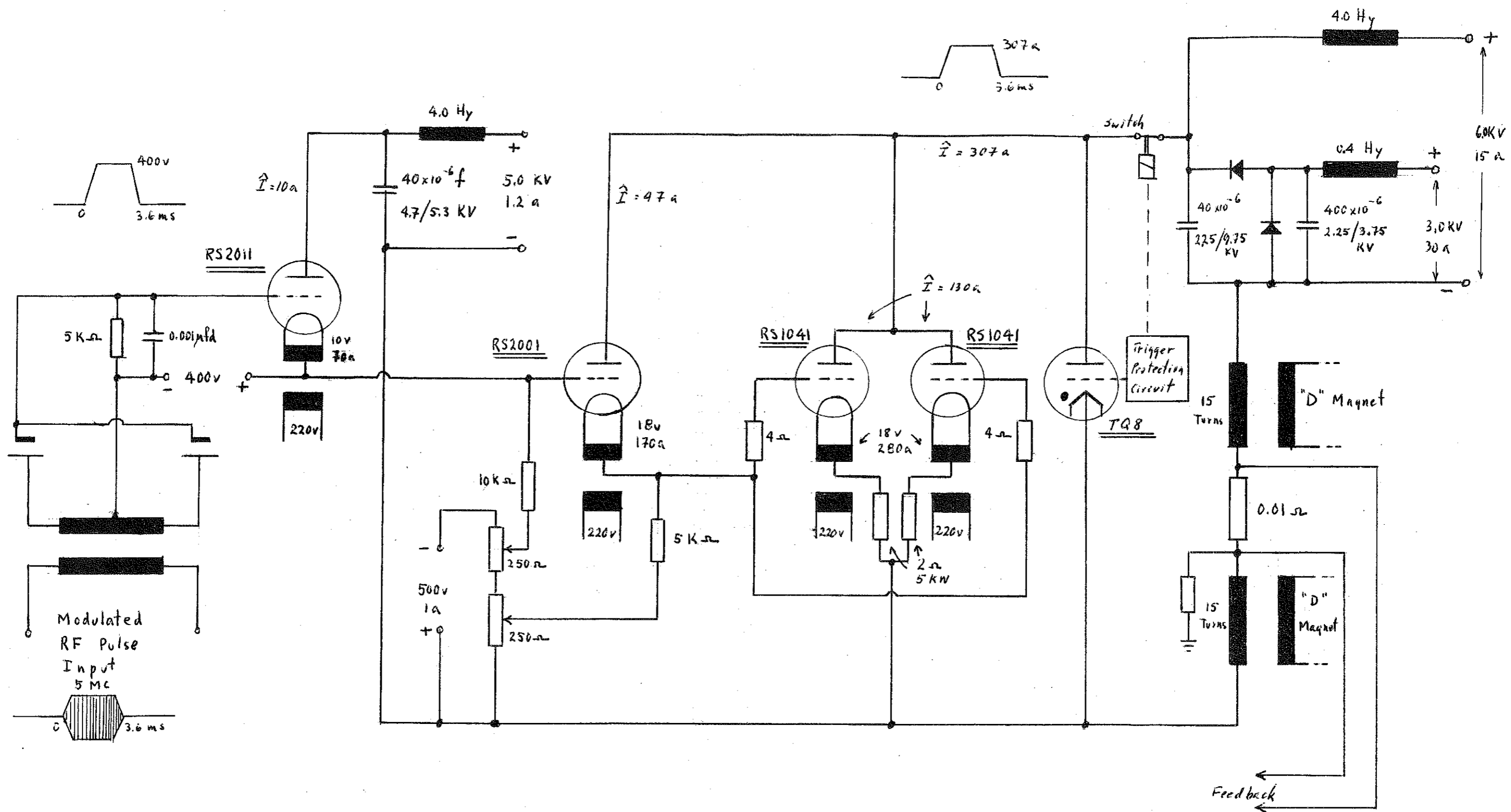
Fig. 2 : "D" Magnet Pulser
