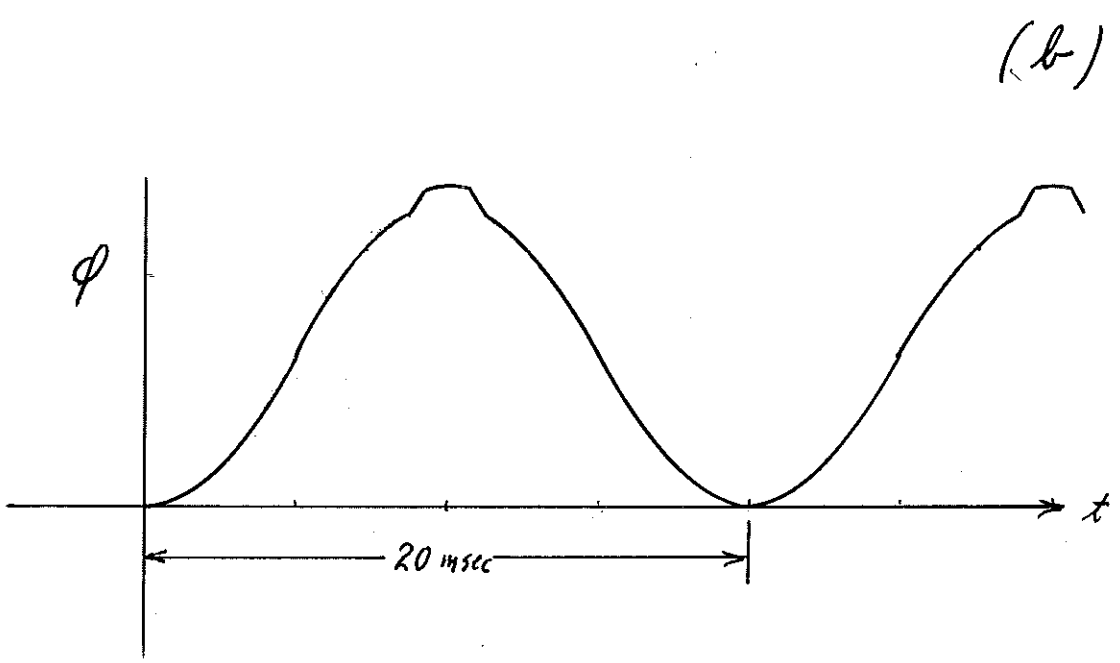
Figure 1: a) Pulse wave shape b) Flux in pulsed magnet
