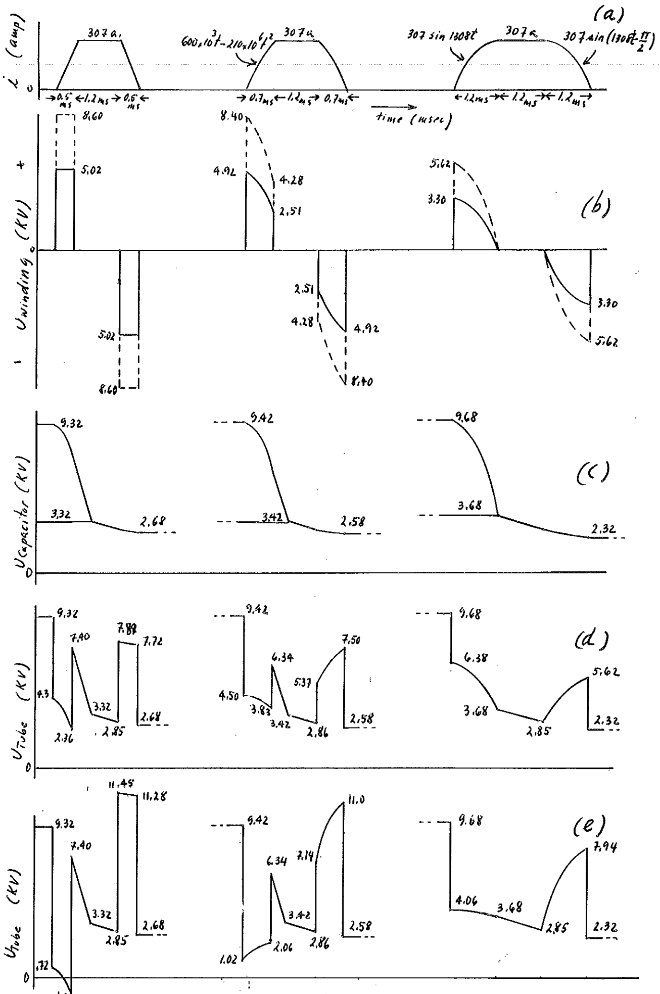
Fig. 9.: D Pulser waveshapes a) Current b) Backleg winding Voltage, dotted line; Airgap winding voltage, solid line c) Capacitor C_1 and C_2 voltages d) Tube voltage with airgap winding e) Tube voltage with backleg winding.
