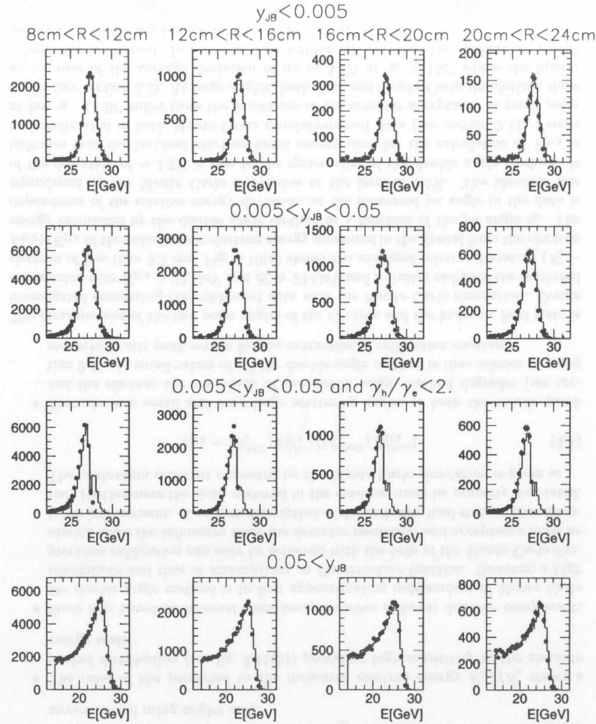
Figure 3.9: The reconstructed electron energies in the data (points) are globally decreased by 0.7% relative to the standard calibration. The Monte Carlo simulation (solid line) is unchanged compared to fig. 3.7.
