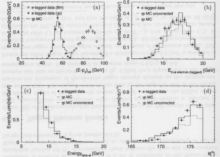
Figure 4.13: Tagged electron data (full points) and corrected PHOJET Monte Carlo simulation (solid line) are compared. (a) distribution of (E - p_z)_{\text{tot}} where the sum includes the energy in the electron tagger. For events with (E - p_z)_{\text{tot}} > 68 GeV (open points) the photon detector requirement is removed. In (b) the energy in the electron tagger, in (c) the energy of the fake electron candidate in the Spacal and in (d) the polar angular distribution of the fake electron candidate are shown. The dashed histogram represents the behavior of the PHOJET Monte Carlo simulation before any correction.
