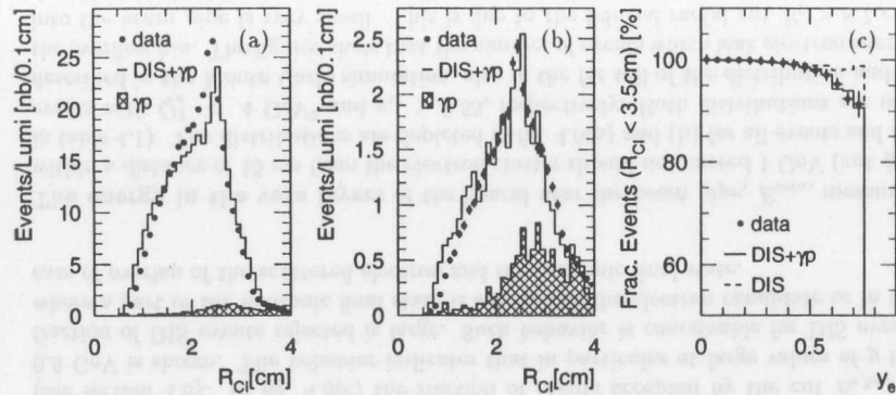
Figure 4.4: The cluster radius R_{cl} is shown in the data (points) and in the DIS+ \gamma p Monte Carlo simulation (solid line). (a) includes all events, (b) shows events with Q_e^2 < 4 \text{ GeV}^2 and y_e > 0.55 . The hatched histogram represents the simulated \gamma p background. In (c) the fraction of events accepted by the electron selection cut R_{cl} < 3.5 \text{ cm} is plotted. The dashed line shows the fraction of accepted true electron events as simulated in the DIS Monte Carlo.
