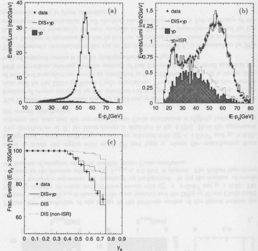
Figure 4.7: The distributions of E-p_z in the data (points) and in the Monte Carlo simulation (solid line). In (a) all events and in (b) events with Q_e^2 < 4 \text{ GeV}^2 and y_e > 0.55 are shown. The hatched histogram represents the simulated photoproduction background. In (b) ISR events are represented as a dashed line. In (c) the fraction of events accepted by the cut E-p_z > 35 \text{ GeV} is plotted for the data (points) and for the DIS+ \gamma p (solid line), DIS (dashed line) and DIS Monte Carlo simulations excluding ISR events (dotted line).
