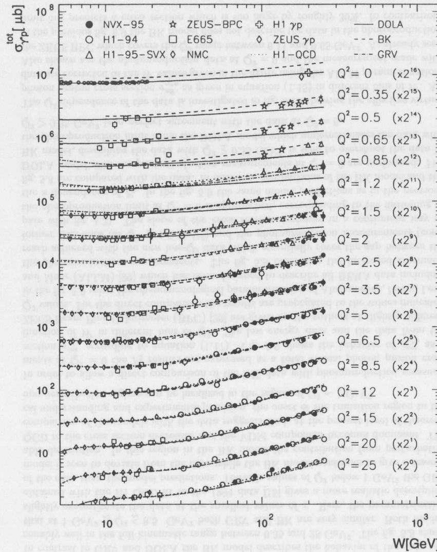
Figure 5.9: The total photon proton cross section \sigma_{\gamma p}^{\text{tot}} as a function of W in different bins of Q^2 . The cross sections are multiplied with the factors indicated in the figure. The results of this analysis are shown by full points. Open points (triangles) refer to results by the H1 Collaboration with the 1994 (1995 shifted vertex) data respectively. Also shown are results from E665 (squares) [98] and NMC (diamonds) [18] as well as the measurements of the total \gamma p cross section by the Collaborations H1 (cross) [23] and ZEUS (diamond) [24]. The data measured with the ZEUS Beam Pipe Calorimeter (BPC) [28] are shown by stars. The curves represent the models by DOLA (solid line), BK (dashed line) and the H1 QCD fit (dotted line).
