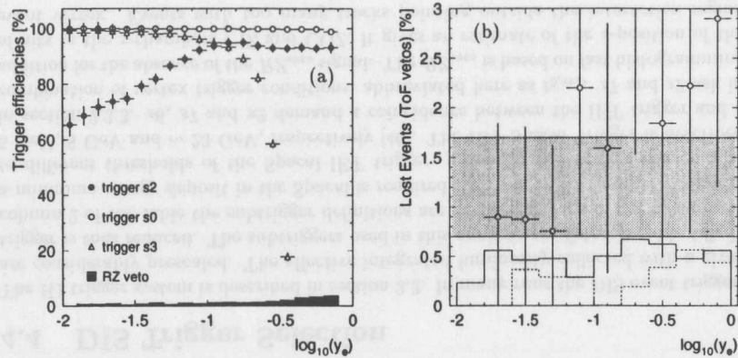
Figure 4.1: (a) The subtrigger efficiencies shown as a function of \log_{10}(y) for the subtriggers s_0 (open points), s_2 (full points) and s_3 (triangles). The black histogram indicates the fraction of events lost due to the RZ_{\text{veto}} requirement. (b) The fraction of lost events due to the ToF background veto is represented by the grey error band. Separately shown are the contributions from BToF-or-PToF (open points), FToF (solid line) and Veto Wall (dashed line).
