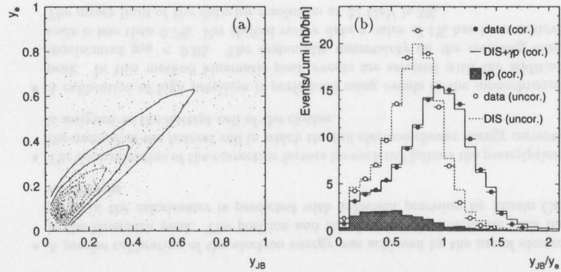
Figure 3.14: (a) Data are used to plot y_{JB} versus y_e . The contour lines indicate the correlation. For the calculation of y_{JB} hadronic energies in the Spacal are multiplied by a factor of 1.5 according to the findings below (see text). (b) The ratio y_{JB}/y_e is plotted before (open points, dashed line) and after (full points, solid line) the correction for data and Monte Carlo simulation, respectively.
