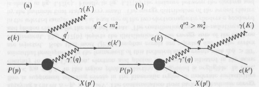
Figure 4.16: The most relevant Feynman diagrams of the process ep \rightarrow epr . (a) initial state radiation, (b) final state radiation. P(p) , e(k) denote the four-momenta of the incident particles. X(p') , e(k') , \gamma(K) refer respectively to the hadronic final state, the scattered electron and the radiated photon. q^2 ( q'^2 , q''^2 ) give the four momentum squared of the virtual photon (electron).
