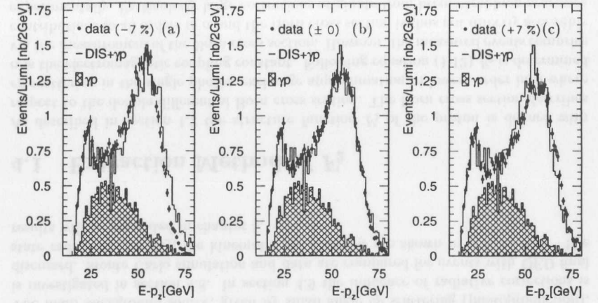
Figure 3.15: The systematic error of the hadronic energy calibration in the Spacal is determined using the E - p_z distribution for events with y_e > 0.55 . The hadronic energy scale in the data (points) is varied by \pm 7\% . In (a) the energy is reduced for data by 7%. In (b) the data are unchanged and in (c) the energy is increased by 7%. Also shown are the DIS+ \gamma p Monte Carlo simulation (solid line) and the simulated \gamma p Background.
