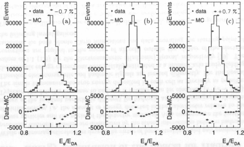
Figure 3.11: Distribution of the ratio between the electron energy measured in the Spacal and calculated via the double angle method E_e'/E_{DA} . The energy scale is varied for data (points) by (a) -0.7\% (b) 0\% (c) +0.7\% . The difference between the data and the simulation is shown in the small diagrams below.
