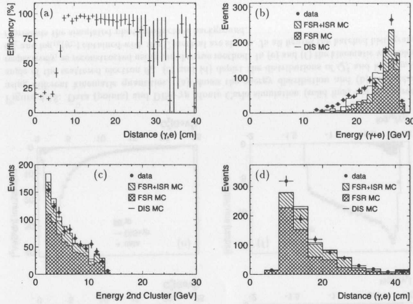
Figure 4.17: (a) Fraction of FSR events with two separate electromagnetic clusters in the Spacal as a function of the distance between the photon and the electron as determined from the Monte Carlo simulation. (b) The sum of the electron and the photon energy in the data (points) and in the Monte Carlo simulation (solid line). The dark hatched histogram shows the true FSR contribution as classified on Monte Carlo generator level. The light hatched histogram refers to events classified as ISR. (c) Energy distribution of the second electromagnetic cluster. (d) Distribution of the distance between the electron and the photon candidate.
