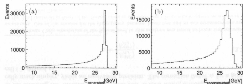
Figure 3.1: The kinematic peak of the energy spectrum of the scattered electrons using Monte Carlo simulated events (a) on generator level and (b) on reconstruction level.
