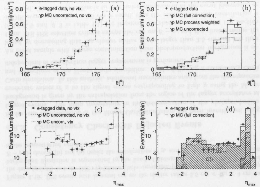
Figure 4.14: (a) Data (points) and PHOJET Monte Carlo simulation (dashed line) are compared with respect to the angular distribution of fake electrons for tagged events without vertex requirement. (b) The same distribution with vertex requirement in the data (points), the uncorrected PHOJET (dotted line) as well as the process weighted (dashed line) and the fully corrected PHOJET (solid line). (c) Distribution of \eta_{max} in the laboratory frame for the data (points) without vertex requirement and PHOJET with (dotted line) and without (dashed line) vertex requirement. (d) Composition of simulated subprocesses as a function of \eta_{max} after correction. EL, DD, GD, PD stand for elastic processes, double dissociation, photon dissociation and proton dissociation, respectively.
