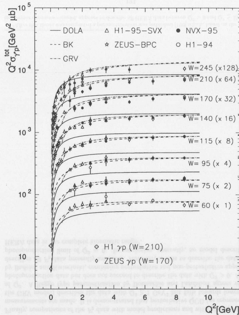
Figure 5.11: The total photon proton cross section \sigma_{\gamma p}^{\text{tot}} scaled with Q^2 as a function of Q^2 in different bins of W . Also shown are the photoproduction results by H1 (cross) [23] and ZEUS (diamond) [24] and the ZEUS BPC data points (stars) [28]. The curves refer to the models DOLA (solid), BK (dashed) and GRV (dashed-dotted).
