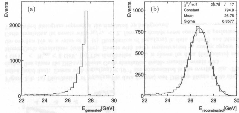
Figure 3.3: Monochromatic energy distribution of the scattered electron using Monte Carlo simulations (a) on generator and (b) on reconstruction level selecting events at y_{JB} < 0.05 . In (b) a Gaussian function is fitted in the interval of 25 GeV to 30 GeV. The parameters of the Gaussian are displayed in the figure caption.
