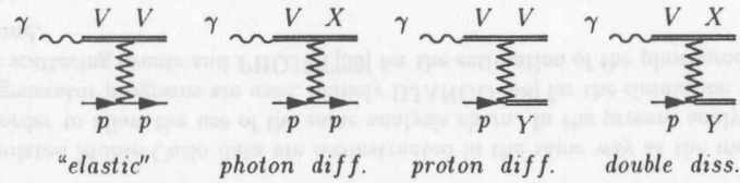
Figure 2.9: The four classes of diffractive processes are sketched. From left to right Elastic processes (EL), Photon Diffraction (GD), Proton Diffraction (PD) and Double Dissociation (DD).
