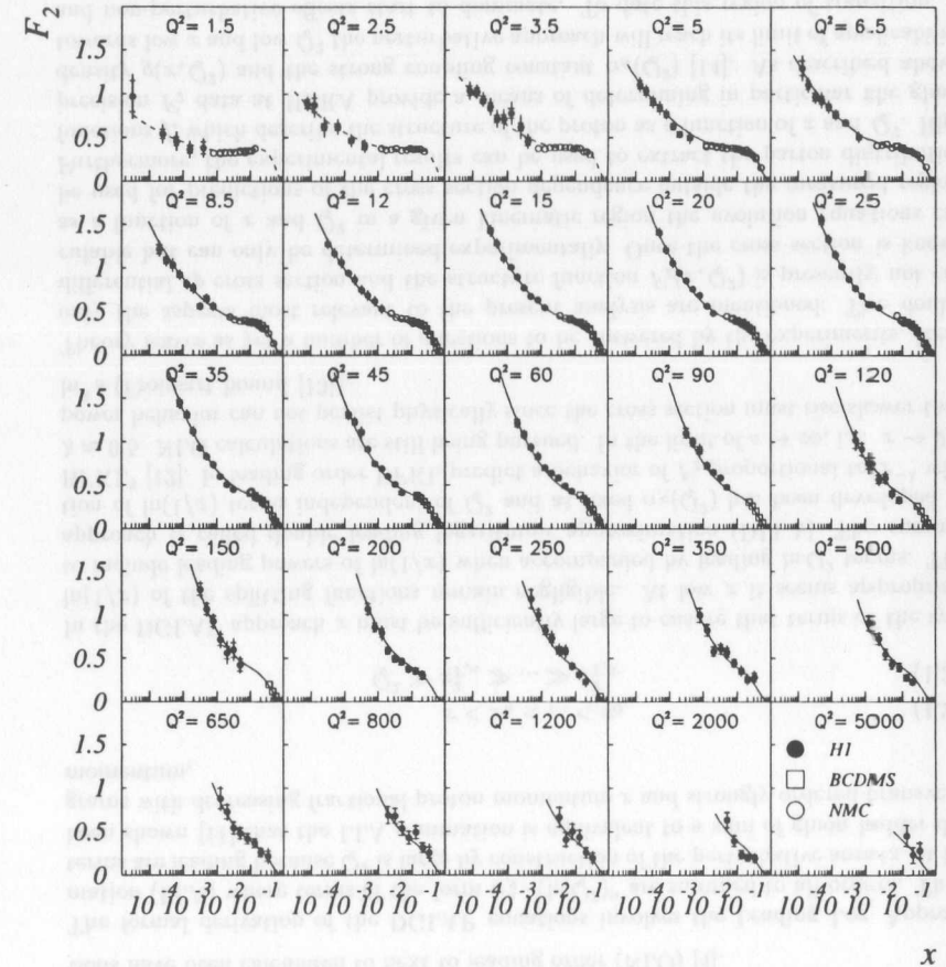
Figure 1.2: The structure function F_2 as a function of x in bins of Q^2 . The results of the H1 Collaboration obtained from data recorded in 1994 [15] are shown by the full points. The fixed target experiments NMC [18] (BCDMS [17]) are represented by open points (squares), respectively. The curves show the results of a NLO QCD fit which includes data for Q^2 \geq 5 \text{ GeV}^2 . The dashed lines show the extrapolation of the fit to lower values of Q^2 .
