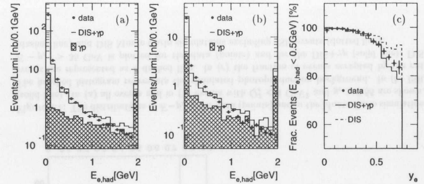
Figure 4.5: Distribution of the energy in the hadronic section of the Spacal behind the electron candidate E_{e,had} is shown for the data (points) and the DIS+ \gamma p Monte Carlo (solid line). (a) includes all events and (b) shows events with Q_e^2 < 4 \text{ GeV}^2 and y_e > 0.55 . The hatched histogram represents the simulated \gamma p background. In (c) the fraction of events accepted by the electron selection cut E_{e,had} < 0.5 \text{ GeV} is plotted. The dashed line shows the fraction of accepted events in the DIS Monte Carlo simulation.
