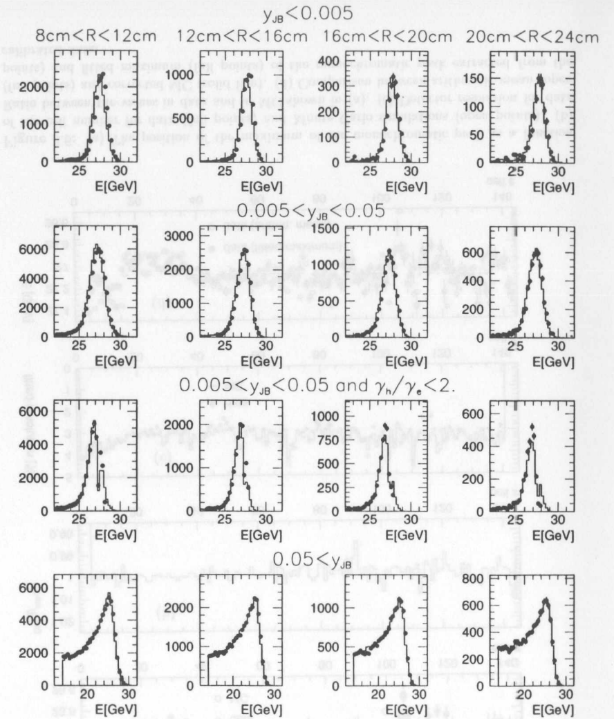
Figure 3.8: The reconstructed electron energies in the data (points) are globally increased by 0.7% relative to the standard calibration. The Monte Carlo simulation (solid line) is unchanged compared to fig. 3.7.
