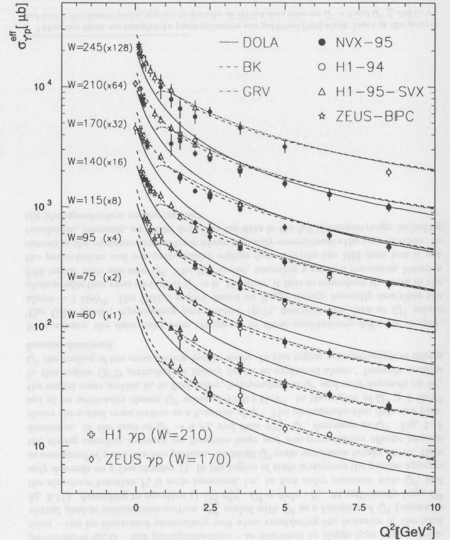
Figure 5.10: The effective photon proton cross section \sigma_{\gamma p}^{\text{eff}} as a function of Q^2 in different bins of W . Also shown are the photoproduction results at W = 170 GeV by the ZEUS Collaboration (diamond) and at W = 210 GeV by the H1 Collaboration (cross). The ZEUS BPC data points are also depicted (stars). The curves refer to the models DOLA (solid), BK (dashed) and GRV (dashed-dotted).
