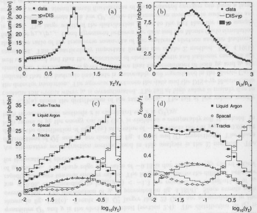
Figure 4.19: Data (points) and Monte Carlo simulation (solid lines) are compared with respect to the measurement of the hadronic final state. (a) shows the ratio y_h/y_e . (b) depicts the ratio of the transverse momenta of the hadronic final state and the scattered electron p_{T,h}/p_{T,e} as determined using the calorimeters. The hatched histogram represents the simulated photoproduction background. In (c) and (d) the contribution to the measured value of \log_{10}(y_h) is shown. (c) The overall distribution is shown by (full points). Also shown are the contributions from the different detector components, namely the Liquid Argon Calorimeter (full squares), the Spacal (open points) and the track chambers (triangles). In (d) the relative contribution of the Liquid Argon Calorimeter (full squares), the Spacal (open points) and the track chambers (triangles) are shown. The solid lines in (c) and (d) represent the respective distributions obtained by the Monte Carlo simulation.
