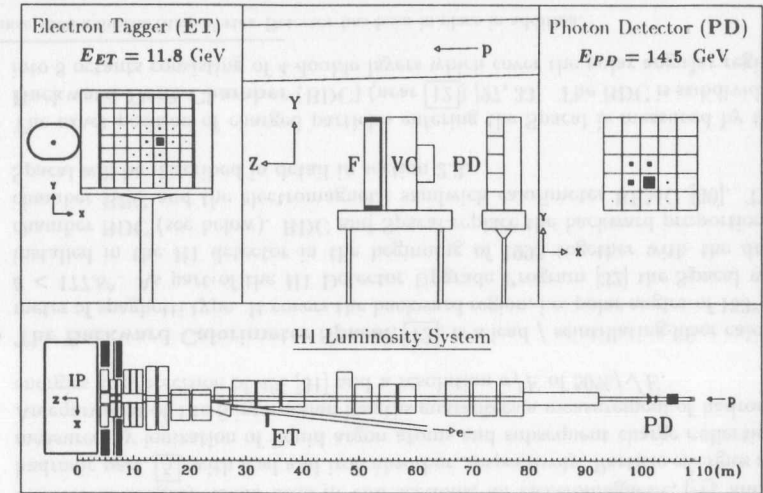
Figure 2.4: Bremsstrahlung event measured by the luminosity system. The scattered electron deposits 11.8 GeV in the electron tagger (ET, upper left panel). The photon energy of 14.5 GeV is measured by the photon detector (PD, upper right panel). The lower picture shows a sketch of the complete luminosity system. The upper central picture zooms the details of the photon detection system consisting of the photon detector (PD) itself and the filter (F) and veto counter (VC) against synchrotron radiation.
