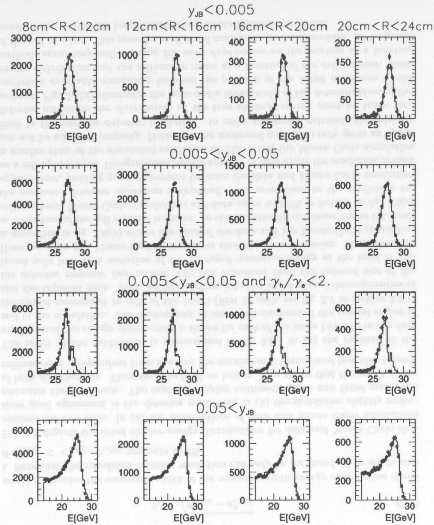
Figure 3.7: Electron energy spectra in Monte Carlo simulations (solid line) and data (points) are compared for four different regions of radius (columns) in different intervals of y_{JB} (rows).
