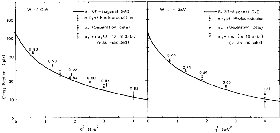
Fig. 3 Off-diagonal GVD prediction (from (14)) for the transverse virtual photon absorption cross section on protons, \sigma_T(W, q^2) , as a function of the virtual photon for momentum squared q^2
