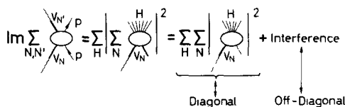
Fig 1 The imaginary part of the virtual forward Compton amplitude or the total virtual photon absorption cross section in GVD
