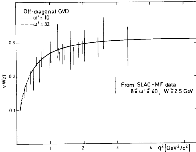
Fig. 4 The transverse part of the proton structure function \nu W_2 as a function of q^2 in the large \omega' diffraction region showing the approach to the scaling limit. The theoretical curve is the off-diagonal GVD prediction calculated from (14). The data points have been computed [9] (see refs. [9] and [1] for details) from the measured 6^\circ, 10^\circ and 18^\circ data [13].
