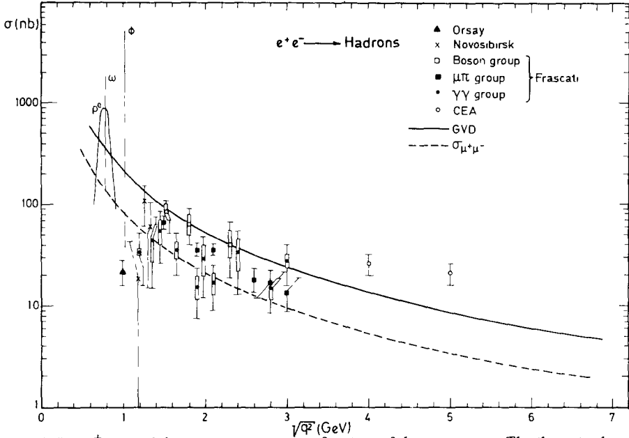
Fig. 2 The e^+e^- annihilation cross section as a function of the c m energy The theoretical curve GVD results from (1) and (2) with the level spacing \lambda = 2
