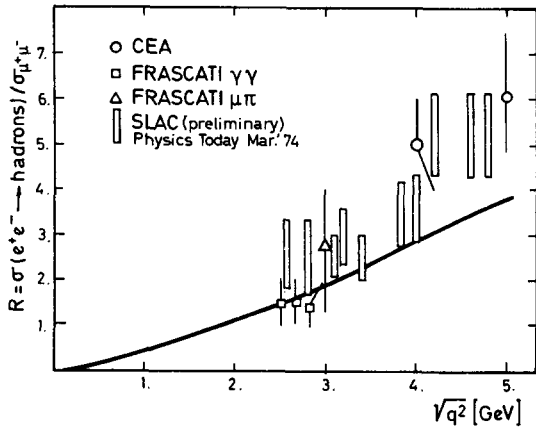
Fig. 4. Predicted total cross section compared to the world's data.
