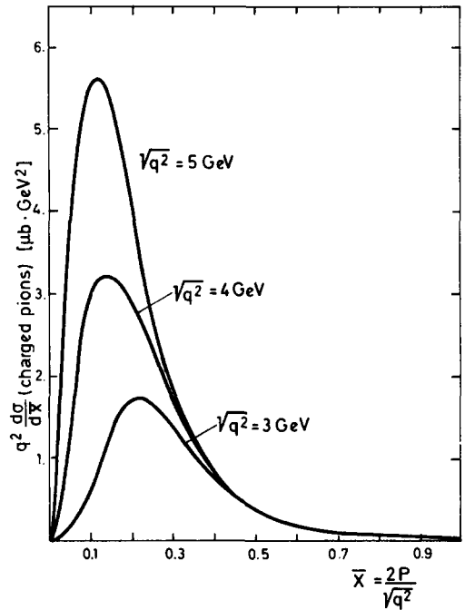
Fig. 3. Prediction of the charged pion inclusive cross section.
