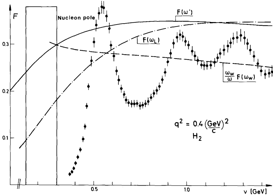
Fig. 3. \nu W_2 of hydrogen as a function of \nu for q^2 = 0.4 (\text{GeV}/c)^2 . For comparison the scaling function in the deep inelastic region is plotted for the variable \omega' , the light-cone variable \omega_L and the variable \omega_W .
