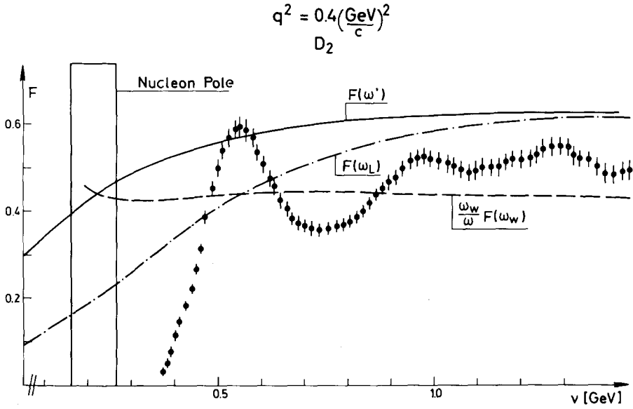
Fig. 5. \nu W_2 of deuterium as a function of \nu for q^2 = 0.4 (\text{GeV}/c)^2 . For comparison the scaling function in the deep inelastic region is plotted for the variable \omega' , the light-cone variable \omega_L and the variable \omega_w .
