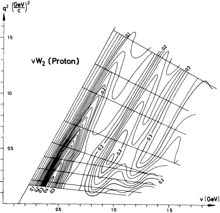
Fig. 1. Lines of constant \nu W_2 in the \nu - q^2 plane for protons. Data were taken along the straight lines of constant scattering angle.
