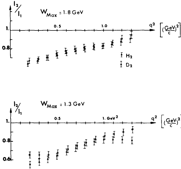
Fig. 7. Ratio (12) as a function of q^2 for two different values of the upper integration limit. Values for protons and deuterons are plotted.
