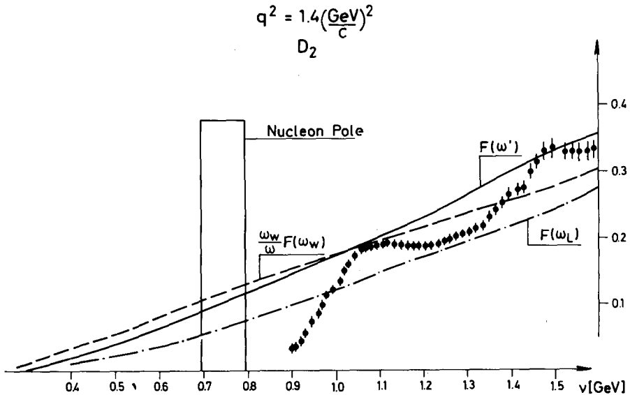
Fig. 6. Same as fig. 5 for q^2 = 1.4 (\text{GeV}/c)^2 .
