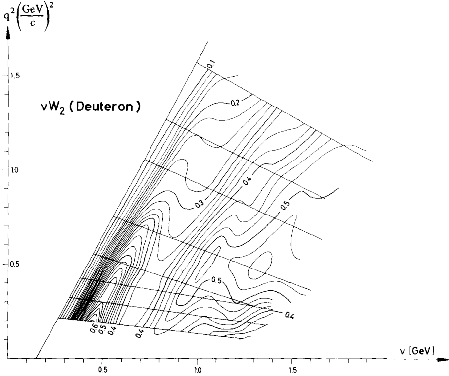
Fig. 2. Same as fig. 1 for deuterons.
