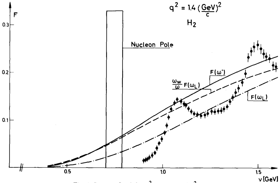
Fig. 4. Same as fig. 3 for q^2 = 1.4 (\text{GeV}/c)^2 .
