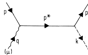
FIG. 2. Isobar contribution to resonant photo- and electroproduction.
