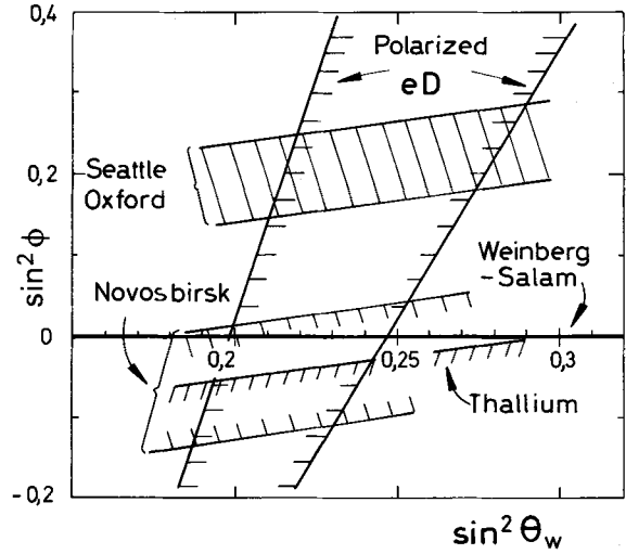
Fig. 1. Allowed region in \sin^2 \theta_w and \sin^2 \phi from polarized electron deuterium experiments [8], atomic bismuth [21, 22], and thallium [23] experiments with one standard deviation
