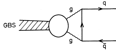
FIG. 1. The lowest-order diagram which gives a GBS decay.
