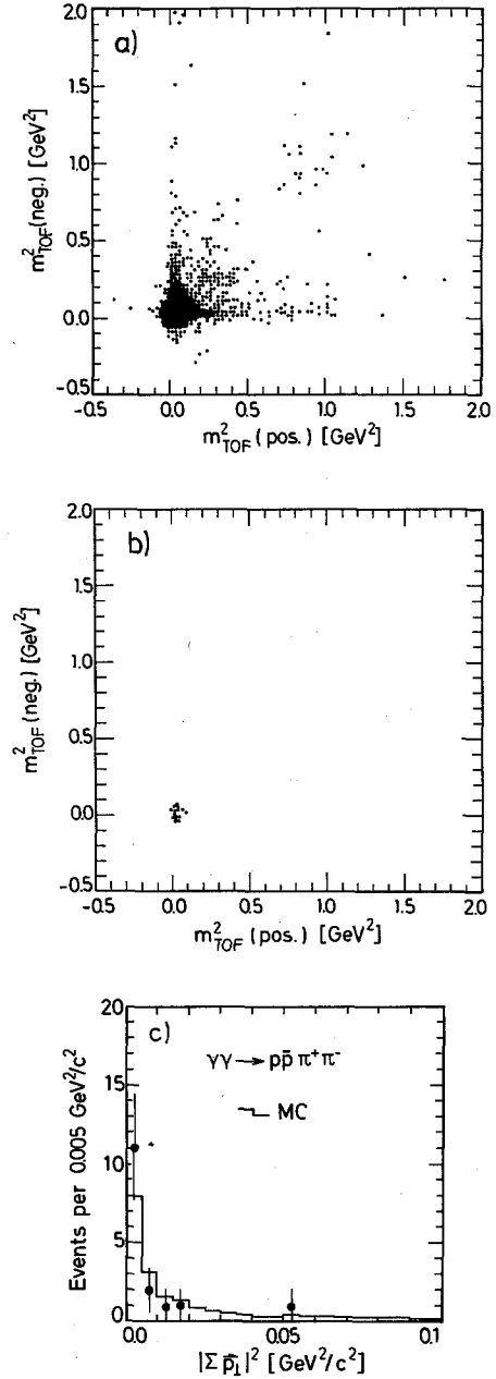
Fig. 1. (a) The larger m_{\text{TOF}}^2 of the positively charged particles versus the larger m_{\text{TOF}}^2 of the negatively charged particles for four-prong events with net charge zero ( |\mathbf{p}| \leq 1.6 \text{ GeV}/c , |\Sigma \mathbf{p}_\perp| < 0.14 \text{ GeV}/c ). (b) The smaller m_{\text{TOF}}^2 of the positively charged particles versus the smaller m_{\text{TOF}}^2 of the negatively charged particles for four-prong events with net charge zero and with one identified p\bar{p} pair. (c) Distribution of |\Sigma \mathbf{p}_\perp|^2 of the \gamma\gamma \rightarrow p\bar{p}\pi^+\pi^- system. The histogram shows the Monte Carlo prediction for phase space production of \gamma\gamma \rightarrow p\bar{p}\pi^+\pi^- .
