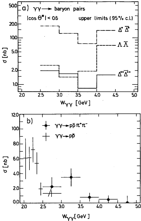
Fig. 3. (a) Upper limits (95% CL) on the cross sections for baryon pair production in two-photon collisions for |\cos \theta^*| \leq 0.6 . (b) Cross sections for the reaction \gamma\gamma \rightarrow p\bar{p}\pi^+\pi^- assuming phase space production. Also shown is the cross section for \gamma\gamma \rightarrow p\bar{p} from ref. [6], extrapolated to |\cos \theta^*| \leq 1 .
