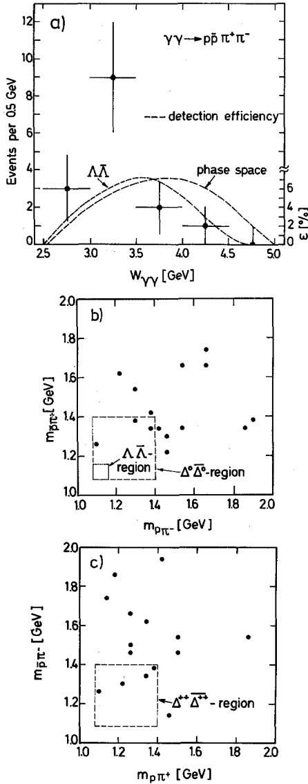
Fig. 2. (a) Uncorrected distribution of the CM energy of \gamma\gamma \rightarrow p\bar{p}\pi^+\pi^- events. Also shown is the energy dependence of the detection efficiency \epsilon for production according to phase space and via \Lambda\bar{\Lambda} pairs (dashed lines). (b) Scatter plot of the invariant mass of the p\pi^- -system versus the invariant mass of the \bar{p}\pi^+ -system for the \gamma\gamma \rightarrow p\bar{p}\pi^+\pi^- events. (c) Scatter plot of the invariant mass of the p\pi^+ -system versus the invariant mass of the \bar{p}\pi^- -system for the \gamma\gamma \rightarrow p\bar{p}\pi^+\pi^- events.
