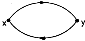
FIG. 1. The quark propagator configuration needed for flavor nonsinglet mesons.
