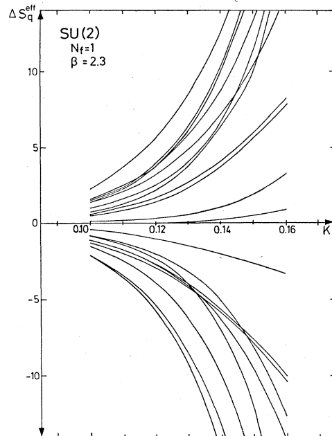
FIG. 7. The dependence of the fermion part of effective action S_{\text{eff}}^q (the average subtracted: \delta S_{\text{eff}}^q \equiv S_{\text{eff}}^q - \langle S_{\text{eff}}^q \rangle_0 ) on the hopping parameter K , for 20 different gauge configurations (Joos and Montvay, 1983). The color group is SU(2) at \beta = 2.3 and N_f = 1 flavor is taken.
