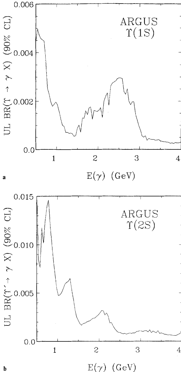
Fig. 3a and b. Upper limit (90% confidence level) for the branching ratio for the decay \Upsilon(1S) \rightarrow \gamma X a and \Upsilon(2S) \rightarrow \gamma X b
