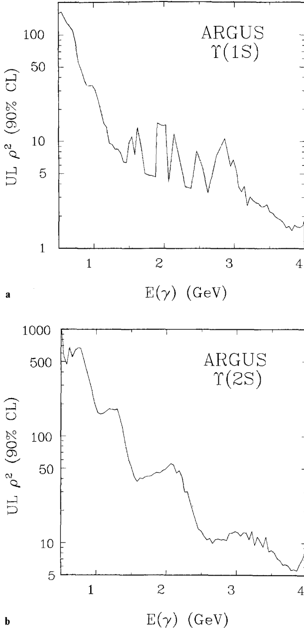
Fig. 8a and b. Upper limits (90% confidence level) for the ratio of vacuum expectation values of the doublet Higgs model [2] and the standard Higgs model [18] as derived from the upper limits for the decays a \Upsilon(1S) \rightarrow \gamma X and b \Upsilon(2S) \rightarrow \gamma X
