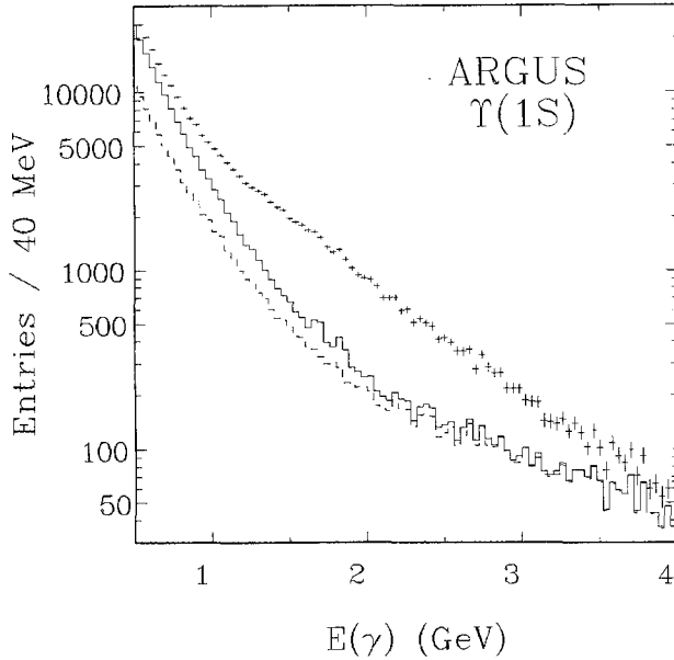
Fig. 1. Gamma spectrum observed with the barrel shower counters. The different curves correspond to successively stricter cuts applied in order to suppress contribution from \pi^0 \rightarrow 2\gamma decays. ++++ raw data, — data after shower shape cut, --- data with \pi^0 -mass cut
