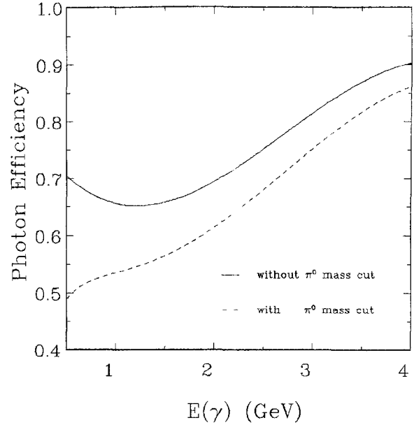
Fig. 2. Reconstruction efficiency of single photons considering the shower shape cut (—) and the \pi^0 -mass cut (---) discussed in the text
