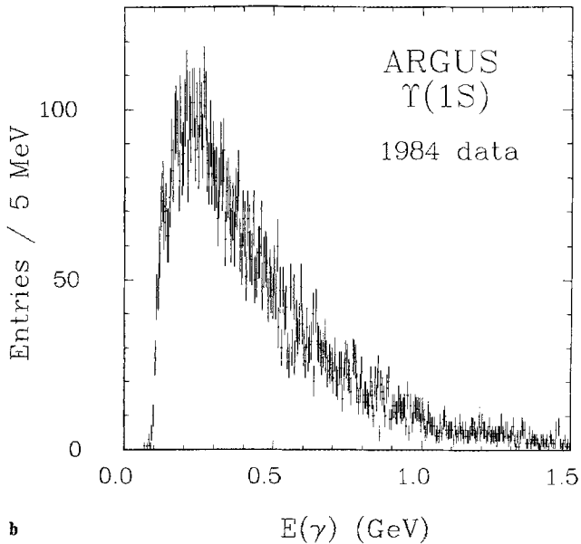
Fig. 5a and b. Spectrum of photons from the decay \Upsilon(1S) \rightarrow \gamma X converted in the beam tube or the inner chamber wall of the ARGUS detector a without and b with \pi^0 mass cut described in the text
