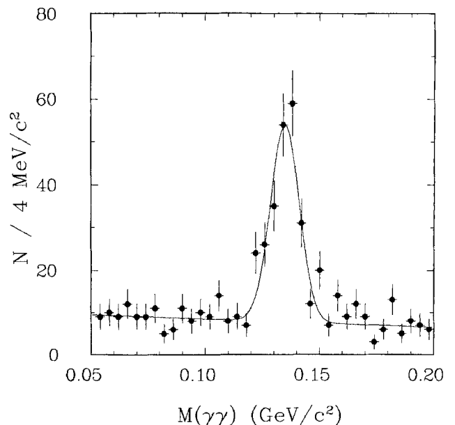
Fig. 4. Invariant mass of pairs of converted photons. The mass of the observed \pi^0 corresponds to (134.8 \pm 0.6) MeV/c 2
