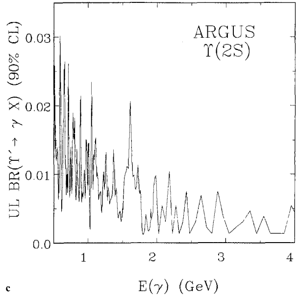
Fig. 7a-c. Upper limits (90% confidence level) for the branching ratio for Y(1S) \rightarrow \gamma X from converted photons, a for the two running periods separately (— data taken 1984, --- data taken 1983) and b combined result. c Corresponding result for the decay Y(2S) \rightarrow \gamma X
