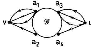
Fig. 6. Arrangement of extra vertices and lines added to the graph \mathcal{G} . The paths \mathcal{P}_1, \dots, \mathcal{P}_4 start at u and pass through a_3 or a_4 via the extra lines connecting these vertices with u . After traversing \mathcal{G} , they arrive at a_1 or a_2 and end at v
