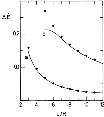
Fig. 3. Comparison of the large L expansions (2.60) (curve a ) and (2.74) (curve b ) with numerically calculated energy values (dots) for \nu=\pi . The energy shift \Delta\hat{E} is equal to \hat{E}-\hat{E}_0 , where \hat{E}_0=0 for the ground state and \hat{E}_0=1 for the first excited state
