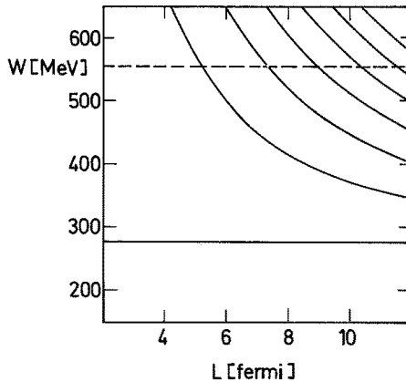
Fig. 1. Energy values of \pi\pi -states with zero total momentum as a function of the box size L neglecting pion interactions. The dashed line indicates the 4-pion threshold. The multiplicity of the levels shown is 1 in the channel with zero spin and isospin
