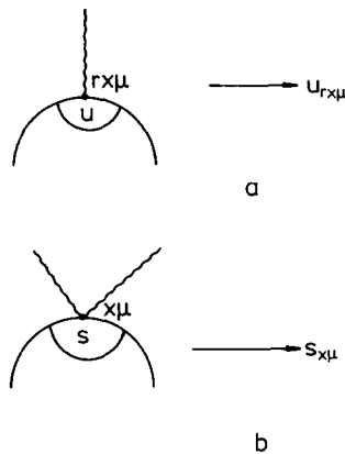
Fig. 1. The gauge field lines end on the scalar blobs either as a single line (fig. 1a) or as a pair of lines in the same point (fig. 1b).
