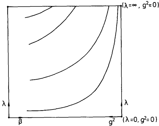
Fig. 5. The qualitative picture of CCP's in the standard Higgs model projected on the (g^2, \lambda) plane. The small g^2 behaviour is the result of WGCE. The extension to larger g^2 is a guess supported by some approximate numerical Monte Carlo calculations at \lambda = \infty, \beta = 2-3 [17, 18]. Note that in reality there is a two-parameter family of CCP's, but here only a one-parameter subset is shown for simplicity.
