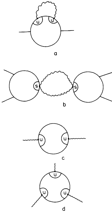
Fig. 2. The WGCE graphs for 1PI vertex functions which have to be calculated for the leading order equations of CCP's. Wavy lines denote gauge fields, full lines the scalar field.
