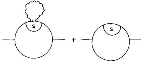
Fig. 4. The lowest order WGCE graphs for the determination of the critical surface. The second graph has an external composite field s_{x\mu} and is proportional to (\kappa - \kappa_0) . (It corresponds to N = 1 in the master formula (44).)
