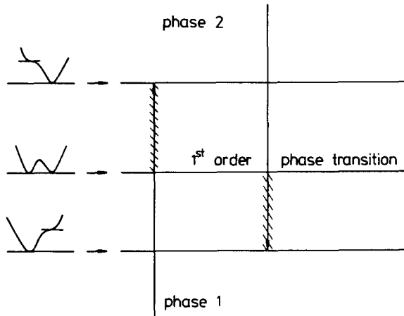
Fig. 3. The critical structure corresponding to a first order phase transition. On the left the qualitative behaviour of the effective potential is shown. Coming from either phase 1 or from phase 2, metastable states occur in the regions where the arrows are hatched. At the phase transition the two minima of the effective potential are equal. At the limits of the metastability the second derivative at one of the local minima becomes zero.
