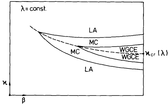
Fig. 6. The schematic lay-out of the regions where interesting Monte Carlo calculations for the coupled gauge-scalar system can be done (MC) and where WGCE can be expected to give a good approximation (WGCE). The uninteresting region of dominant lattice artifacts is denoted by LA. The confining-Higgs phase transition is at the dashed line. The whole picture is for \lambda = \text{const.}
