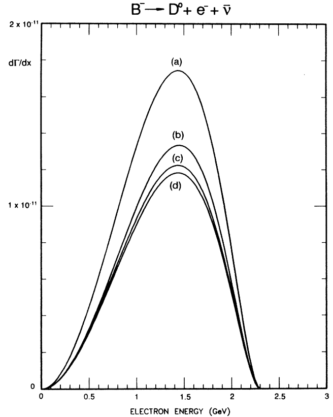
FIG. 2. Electron spectrum d\Gamma/dx in GeV units for the semileptonic decay B^- \rightarrow D^0 + e^- + \bar{\nu} for the models described in the text. x = 2E_e/m_B . (a) ISGW, (b) HMW, (c) KP, (d) KS.
