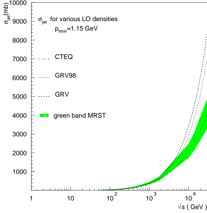
Fig. 1: minijet cross section for different input parton densities.
