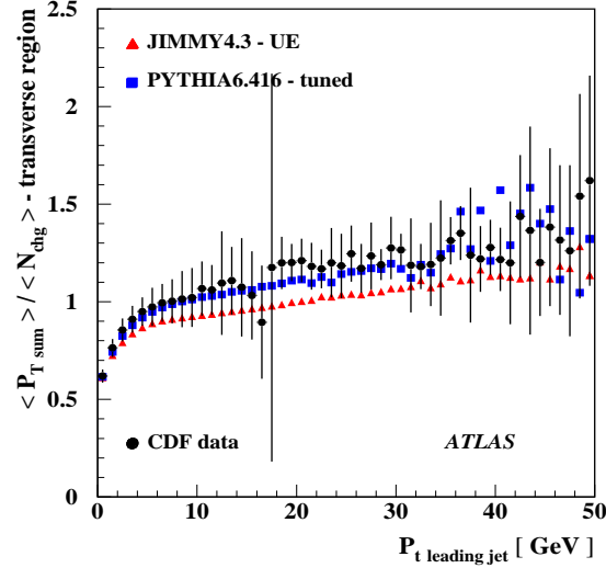
Fig. 3: PYTHIA version 6.416 - tuned and JIMMY version 4.3 - UE predictions for the underlying event in p\bar{p} collisions at \sqrt{s} = 1.8 TeV compared to the ratio \langle p_T^{\text{sum}} \rangle / \langle N_{\text{chg}} \rangle .
