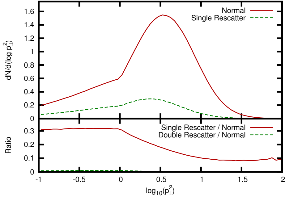
Fig. 2: Average distribution of scatterings, single rescatterings and double rescatterings per event ( \sqrt{s} = 1.96 \text{ GeV} , minimum bias). Double rescattering is not visible at this scale in the dN/d(\log p_{\perp}^2) plot, but is visible in the ratio
