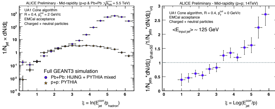
Fig. 6: Left : Hump-backed plateau in p + p (stars) and Pb + Pb collisions not background subtracted (circles) as a function of \xi at \sqrt{s_{NN}} = 5.5 TeV. Right : ratio of the HBP obtained in a p + p quenched scenario over a non quenched one vs \xi in p + p collisions at \sqrt{s_{NN}} = 14 TeV.
