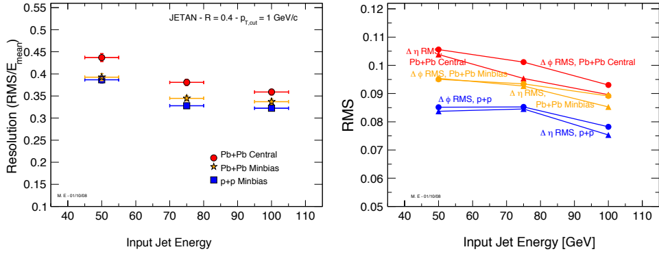
Fig. 5: Left : jet energy resolution versus the input jet energy of 50, 75 and 100 \pm 5 GeV for p + p (squares), Pb + Pb Minbias (stars) and Pb + Pb Central (circles) collisions. Right : angular resolutions (same experimental conditions).
