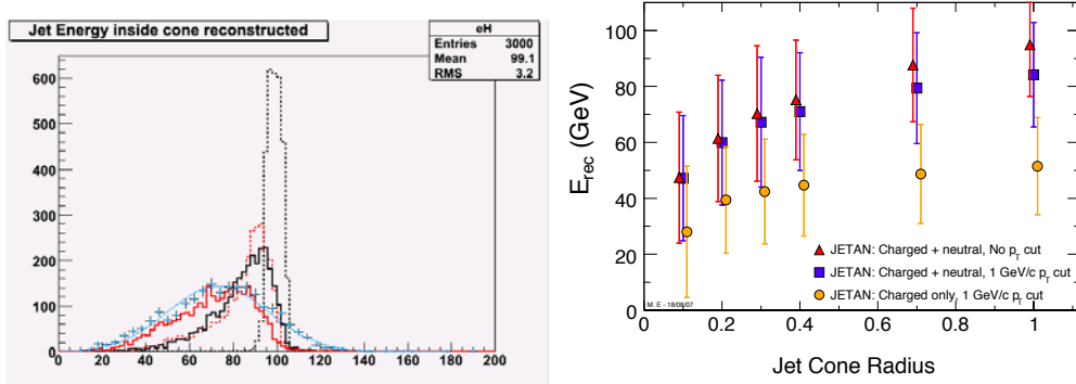
Fig. 1: Left : cone energy of 100 GeV jets reconstructed with PYCELL with R = 1 (dark dashed line), with the ALICE cone finder with detector inefficiencies and acceptance included in the simulation with R = 1 (red dashed), without detector effects but R = 0.4 (dark full), with both effects (red full). The markers shows the result from a full simulation. Right : cone energy of 100 \pm 5 GeV fully simulated jets vs R for the three cases described in the text.
